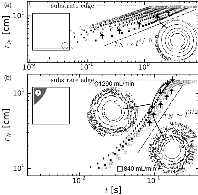
FIG. 5. Plots of measurements of the azimuthally averaged spreading radii as functions of time for rinsing liquids (water) spreading across bare and SDS-coated substrates from (a) Region 1 and (b) Region 3. Symbol shapes indicate a particular flow rate as in Fig. 3(b). Color \blacksquare indicates the rotation rate as 0 rev/min in panel (a), and \blacksquare and \blacksquare indicate 750 and 1000 rev/min, respectively, in panel (b). Open and filled symbols indicate bare or SDS-coated substrates, respectively. Dashed and dotted lines indicate power laws and the edge of the substrate, respectively. Arrows indicate points in experiments on bare substrates [(a) Q = 1290 ml/min, \Omega = 0 rev/min; (b) Q = 840 and 1290 ml/min, \Omega = 1000 rev/min] corresponding to the concentric outlines of the spreading fronts (insets).
