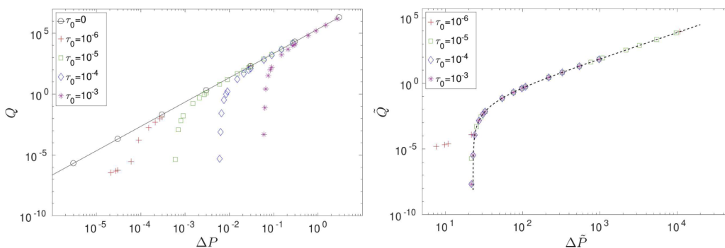
FIG. 11. Flow rate of the FCC packing as a function of the pressure difference \Delta P for different values of \tau_0
