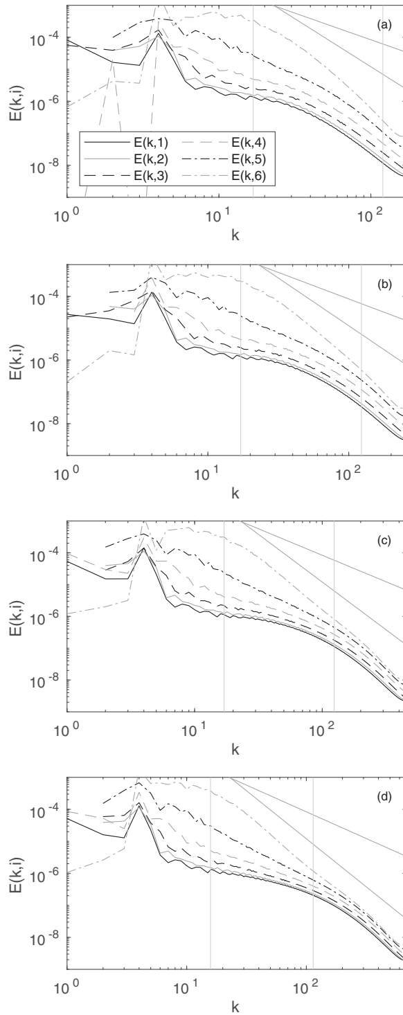
FIG. 9. Directional kinetic energy spectra for N = 0.30 for (a) n = 384 , (b) 576, (c) 1024, and (d) 1536. In all cases, k_b \approx 17 and k_o \approx 120 are shown with vertical lines. The reference lines have slopes of -5/3 and -3 .
