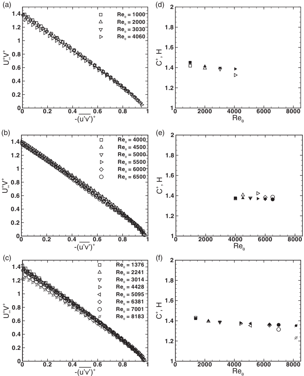
FIG. 1. (a–c) Variation of U_\infty^+ V^+ with the Reynolds shear stress. (d–f) Comparison of C^+ (open symbol) with the shape parameter (filled symbol). Data shown are Schlatter and Örlü [6] in panels (a) and (d), Simens et al. [5] in panels (b) and (e), and Eitel-Amor et al. [7] in panels (c) and (f).
