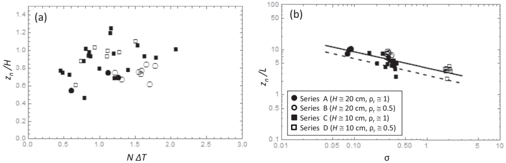
FIG. 5. (a) Plume neutral buoyancy depth vs release duration. (b) Plume neutral buoyancy depth scaled by intrinsic scales.
