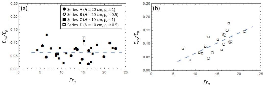
FIG. 8. Energy ratio. (a) \rho_r \cong 1 ; (b) \rho_r \cong 0.5 .
