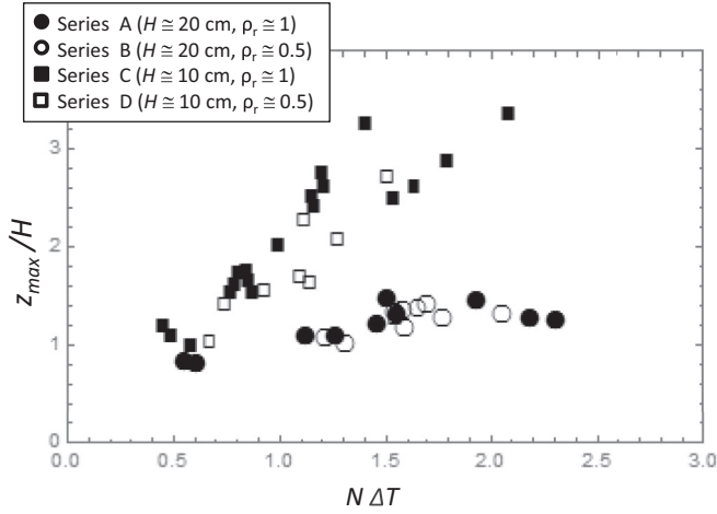
FIG. 4. Plume maximum depth vs release duration.
