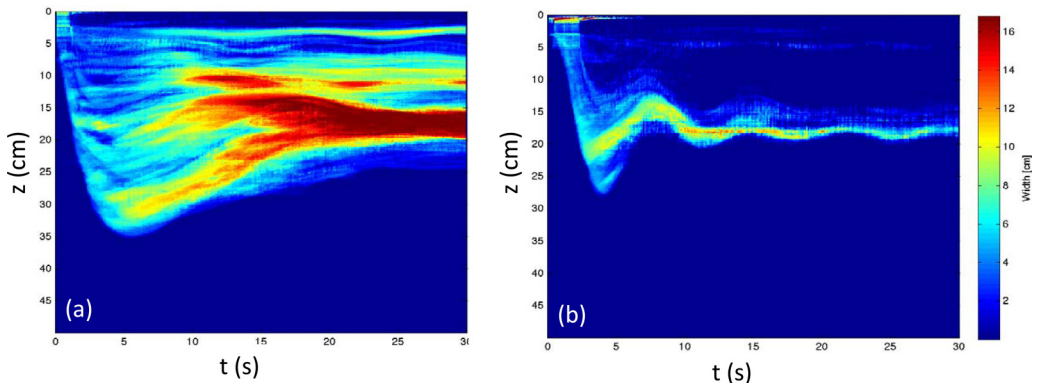
FIG. 3. Plume width as a function of depth and time, evaluated over a cross-sectional window of 17.2 cm. (a) Series C, run 19: H = 14.0 cm, \rho_r = 1.49 , \Delta T = 1.68 s, z_{\max} = 35.3 cm, and z_n = 16.7 cm. (b) Series B, run 66: H = 21.7 cm, \rho_r = 0.58 , \Delta T = 1.83 s, z_{\max} = 28.2 cm, and z_n = 17.9 cm.
