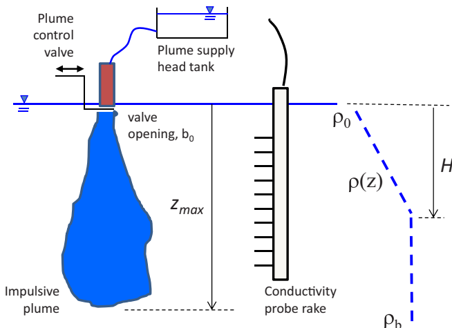
FIG. 1. Schematic of experimental configuration.
