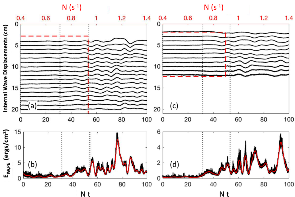
FIG. 7. Internal wave displacements and cumulative energy within the stratified layer. (a,b) Series A, run 3B: H = 21.5 cm, \rho_r = 1.31 , and \Delta T = 1.62 s. (c,d) Series D, run 84: H = 12.3 cm, \rho_r = 0.44 , and \Delta T = 1.25 s. Wave displacements in (a,c) are scaled by a factor of 5, for clarity.
