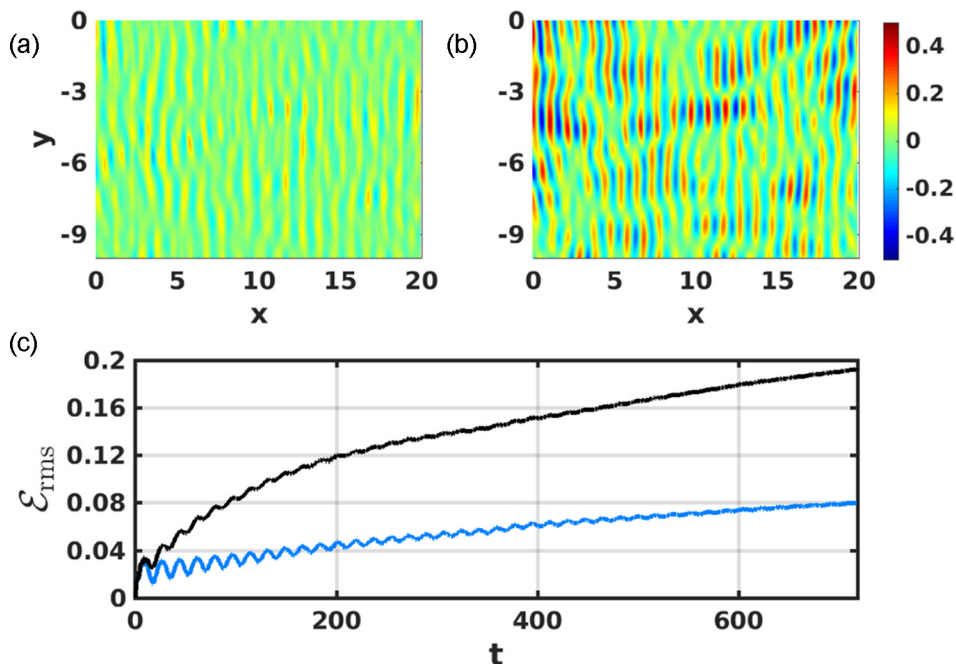
FIG. 6. Top row: difference of \eta computed with (a) improved amplitude model Eq. (22) and HOSM and (b) amplitude model Eq. (17) and HOSM, for the scattering experiment in Fig. 1. The panels shown here correspond to the same time and spatial location as those shown in Figs. 1(b) and 1(d). Notice that the improved model has relatively less pointwise errors. Bottom: root-mean-square error, \mathcal{E}_{\text{rms}} , versus time for the scattering experiment in Fig. 1 when computed with the improved amplitude model Eq. (22) (blue) and amplitude model Eq. (17) (black). Observe that the improved model accumulates less error over time compared to the original model.
