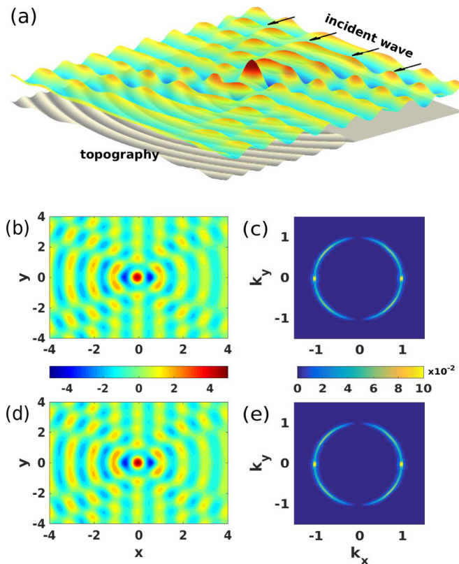
FIG. 2. (a) Three-dimensional depiction of surface gravity wave focusing, showing the free surface displacement \eta computed from the amplitude Eq. (22) at t = 152 (21.2 wave periods), a time of maximum focusing after equilibration is reached with a focal amplitude of 5.0a . The topography \zeta is shown underneath and is shaped as a concave mirror designed to focus the incident waves (entering from the right side) at the center of the domain. The focal point is indicated by the red peak at the center. Panels (b) and (c) show the amplification \eta/a and the spectrum of \eta , while (d) and (e) are the same quantities obtained by integrating the fully nonlinear Eqs. (1).
