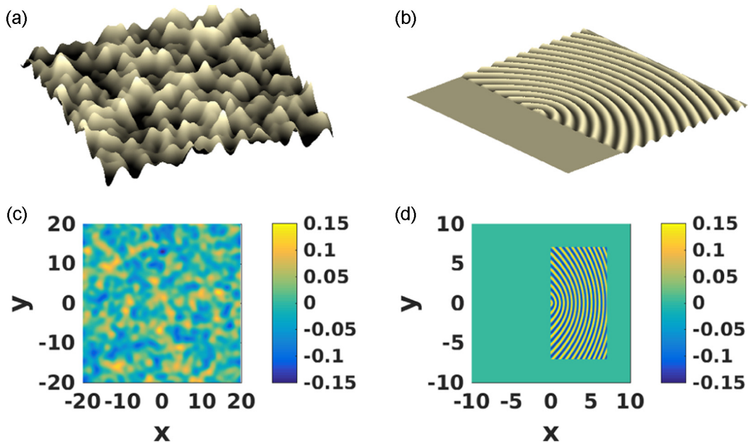
FIG. 5. Topographic field \zeta used for the scattering experiments shown in a three-dimensional depiction (a) and from directly overhead (c). The colors shown in (c) are for the case with \epsilon = 0.15 , corresponding to that used in Fig. 1. The random topography stretches across the entire domain. Topographic field for the focusing experiments with \epsilon = 0.15 are shown in (b) and (d) corresponding to that used in Fig. 2. \zeta was computed using Eq. (A5) in the patch shown and is zero outside the patch. Only a subdomain is shown with the full domain stretching from -20 to 20 in both x and y . The coordinates x and y are nondimensionalized by \lambda .
