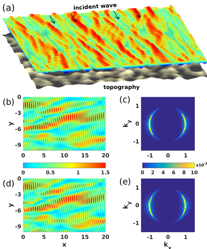
FIG. 1. (a) Three-dimensional depiction of surface gravity wave scattering, showing the free surface displacement \eta computed from the amplitude Eq. (22) at the final time of integration t = 720 (100 wave periods) and the random topography underneath for \epsilon = 0.15 . Incident waves enter the domain from the far side and are scattered by the bottom topography, as can be seen by the irregular and elongated wave envelopes (features highlighted in red) which have developed. Panels (b) and (c) show the scaled magnitude of the surface wave field, |\eta|/a , and the Fourier spectrum of \eta at the same time, obtained by integrating the amplitude equation. Panels (d) and (e) are the same quantities shown in (b) and (c), but obtained by integrating the fully nonlinear Eqs. (1).
