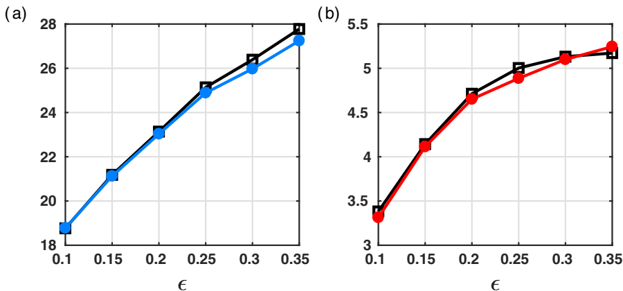
FIG. 4. (a) Effect of \epsilon on effective scattering angle \theta_e (degrees) and comparison between amplitude Eq. (22) (blue, dots) and fully nonlinear Eqs. (1) (black, squares) for scattering experiments. (b) Effect of \epsilon on amplification and comparison between amplitude equation (red, dots) and fully nonlinear equations (black, squares) for focusing experiments. (See text for definitions of \theta_e and amplification.)
