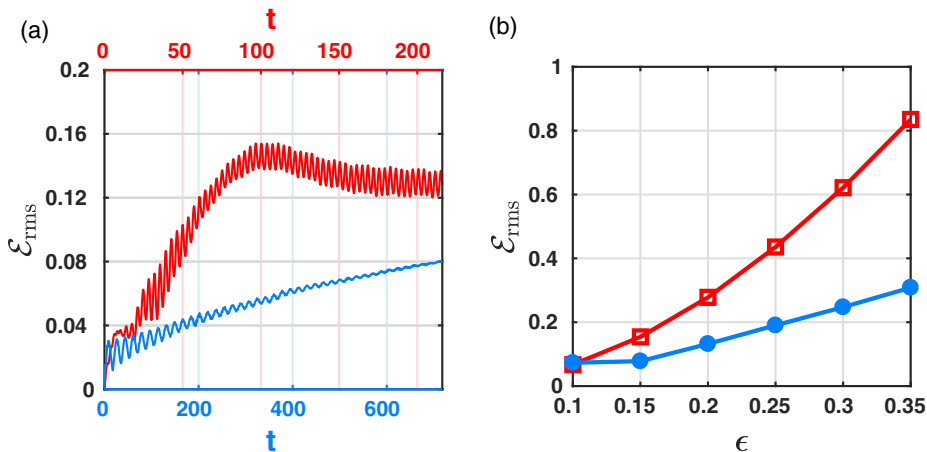
FIG. 3. (a) The root-mean-square error \mathcal{E}_{\text{rms}} at time t for the scattering (blue) and focusing (red) experiments shown in Figs. 1 and 2, respectively. (b) Effect of \epsilon on \mathcal{E}_{\text{rms}} for a set of scattering (blue, dots) and focusing (red, squares) experiments.
