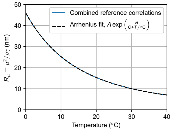
FIG. 5. Viscous length scale of seawater as a function of temperature. Reference correlations [45,46] for the viscosity, density, and surface tension of seawater with salinity 35 \text{ g kg}^{-1} (typical of the oceans) as a function of temperature are combined to form the viscous length scale R_\mu \equiv \mu^2/\rho\gamma . This length scale is plotted along with an Arrhenius fit of the form R_\mu(T) = A \exp\left(\frac{B}{C+T/^\circ\text{C}}\right) , where A = 0.06202 \text{ nm} , B = 661.3 , and C = 100.1 . The Arrhenius fit differs from the combined reference correlations by less than 0.5% for the whole temperature range 0^\circ\text{C} \leq T \leq 40^\circ\text{C} .
