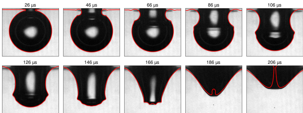
FIG. 10. Overlays of the air-water interface during bubble burst from simulation results (red) with experimental images. The experimental bubble radius is R = 209 \mu m and bursts in water, corresponding to a Laplace number La = 17200 . The time between snapshots is 20 \mu s and no fitting parameters are used other than the offset time, here 26 \mu s , of the first experimental image relative to t = 0 in the simulation.
