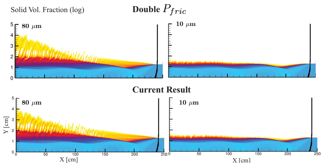
FIG. 16. Particle volume fraction of a shock passing over a dust layer containing two types of particles ( d_{s1} = 80 \mu\text{m} , d_{s2} = 10 \mu\text{m} ). Top: simulation results with 2 \times P_{fric,i} ; bottom: results with current model ( 1 \times P_{fric,i} ).
