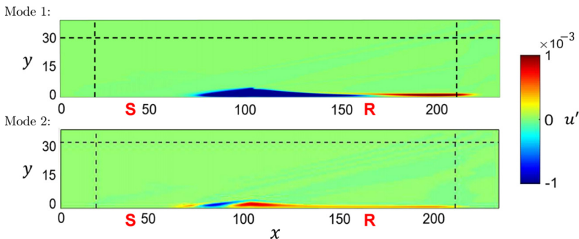
FIG. 8. Stable global modes labeled in Fig. 7 colored by the real part of the nondimensional streamwise velocity perturbation. Here the dashed lines indicate the start of three different sponge layers.
