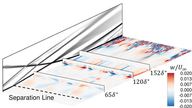
FIG. 6. Color contours of spanwise velocity for a SWBLI at \theta = 13.6^\circ . Contours are shown on the same planes as in Fig. 4, including grayscale contours of density gradient magnitude on the left.
