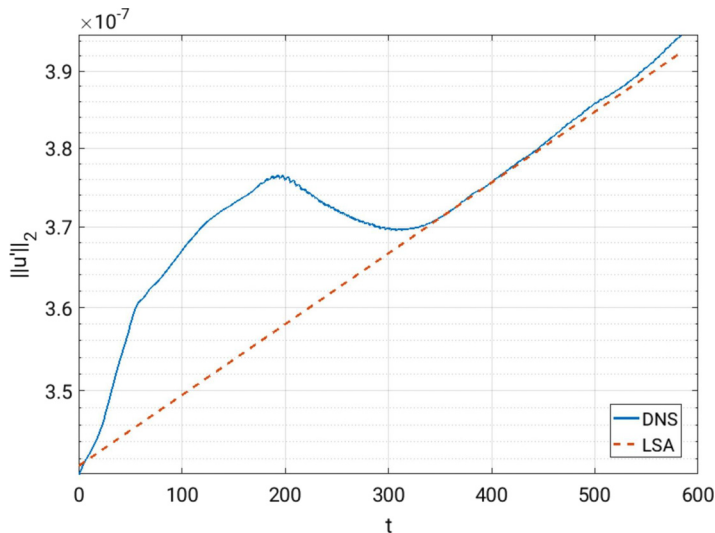
FIG. 12. Temporal variation of the L_2 -norm of an unstable stationary mode predicted by global stability analysis compared to the growth rate from the DNS after adding this global mode. This corresponds to an incident shock angle of \theta = 13^\circ and a spanwise wave number of \beta = 0.25 .
