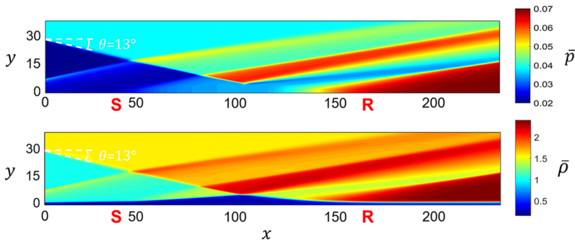
FIG. 2. Contours of nondimensional pressure and density for a 2D oblique shock-wave/laminar-boundary-layer interaction with an incident shock angle of \theta = 13^\circ .
