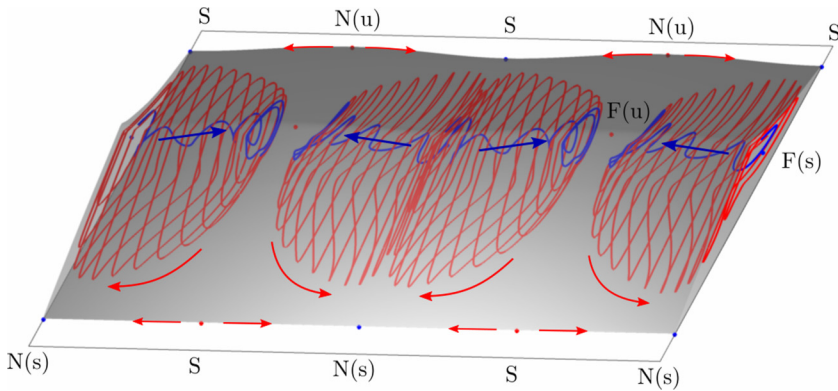
FIG. 15. Toroidal streamline patterns inside the recirculation bubble created by three-dimensional SWBLI instability. Corrugation of the impinging shock creates a region of high pressure just upstream of the point F(u) . This pushes streamlines at the periphery of the recirculation bubble away from this point and towards the point F(s) . As they recirculate, these streamlines (red) trace the exterior of a horizontally aligned torus. At F(s) , they are attracted to the center of the recirculation bubble and then quickly pass through the center of the torus to reemerge close to F(u) .
