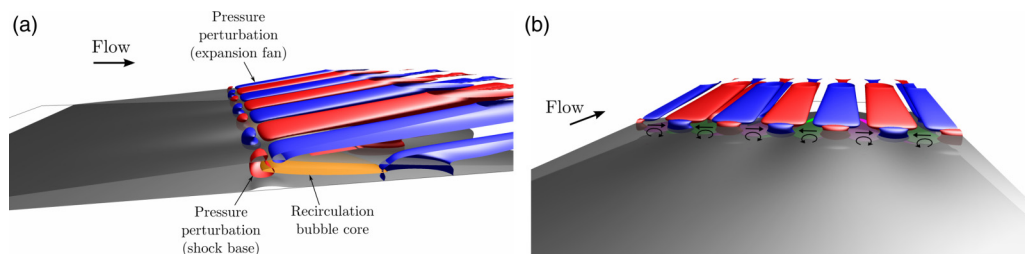
FIG. 14. (a) Side view of the recirculation bubble (gray) perturbed by the same global mode shown in Fig. 13. The front edge cuts through the spanwise location of maximum bubble strength (the spanwise position corresponding to the maximum streamwise extent of the bubble core as indicated by the yellow isosurface). At this spanwise location, the bubble pushes the impinging shock foot forward, producing a patch of positive pressure perturbation bounded by a red isosurface. Above the bubble, a shift in the expansion fan produces a negative pressure perturbation bounded by a blue isosurface. (b) Pressure perturbations produced by the impinging shock foot have the correct phase to drive the streamwise vortices (magenta and green isosurfaces) shown in Fig. 13(a). See [38] for a movie showing these figures from different angles.
