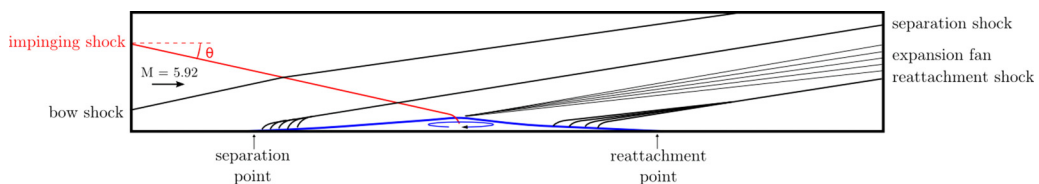
FIG. 1. Schematic of an oblique shock wave (red) impinging on a Mach 5.92 boundary layer. The adverse pressure gradient associated with the impinging shock causes the boundary layer to separate from the wall, forming a recirculation bubble (blue).
