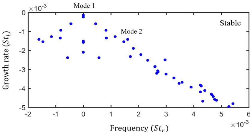
FIG. 7. Eigenvalue spectrum of a SWBLI at M_\infty = 5.92 from GSA with \theta = 12.6^\circ and \beta = 0.25 .
