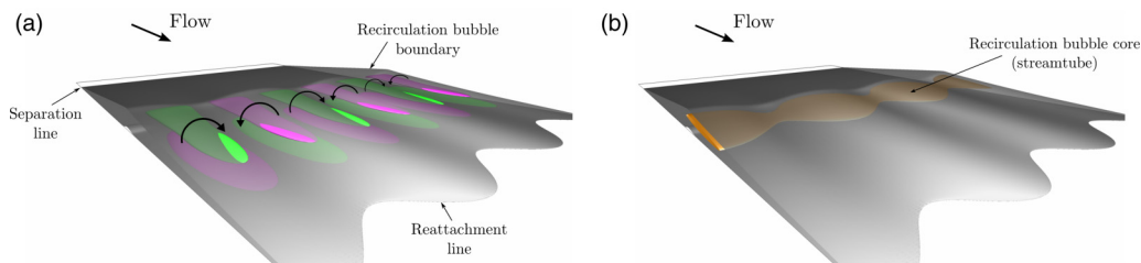
FIG. 13. Rear view of the SWBLI recirculation bubble perturbed by the critical global mode. In both images, the gray separation stream surface bounds the recirculating flow contained in the bubble. (a) Magenta and green isosurfaces of positive and negative streamwise vorticity show a spanwise array of counterrotating streamwise vortices that form just under the apex of the recirculation bubble. (b) In response to the streamwise vortices, the recirculation bubble expands and contracts periodically in the span. The yellow surface represents another stream surface, taken closer to the core of the recirculation bubble. See [38] for a movie showing these figures from different angles.
