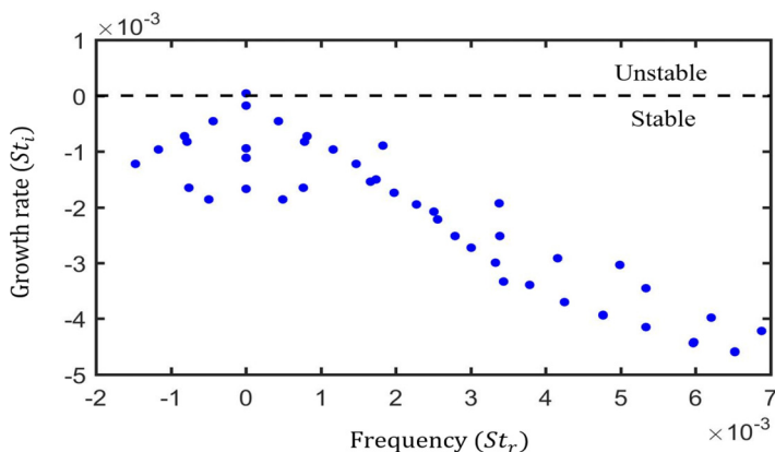
FIG. 9. Eigenvalue spectrum of a SWBLI at M_\infty = 5.92 from GSA with \theta = 13^\circ and \beta = 0.25 . These conditions produce one eigenvalue in the unstable upper half plane. The unstable eigenvalue has zero frequency, indicating stationary instability.
