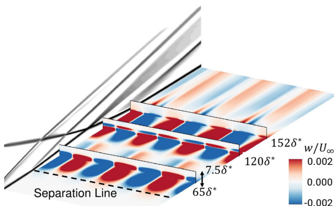
FIG. 4. Color contours of spanwise velocity shown on a wall-parallel plane close to the wall and three wall-normal planes for a 3D oblique shock-wave/boundary-layer interaction with \theta = 13^\circ . Grayscale contours of the density gradient magnitude are shown on a streamwise slice on the left.
