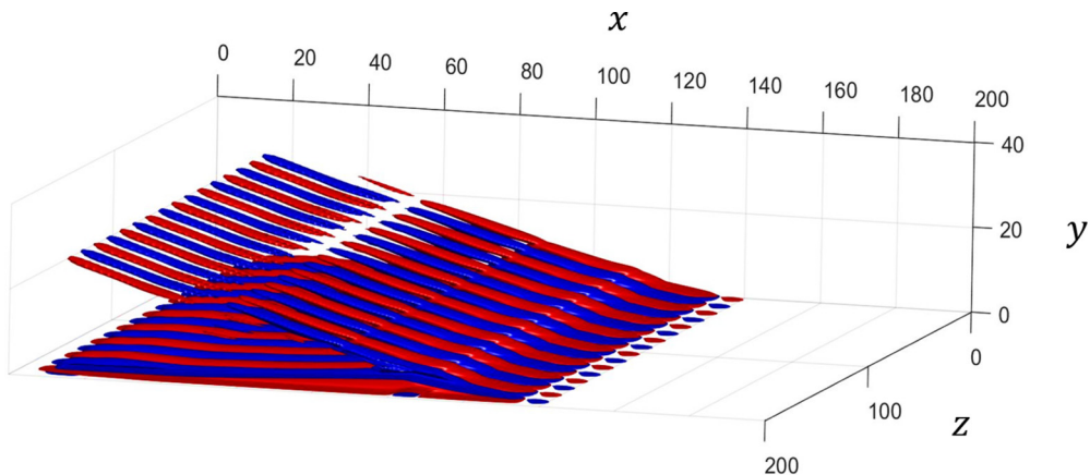
FIG. 18. Adjoint mode corresponding to the critical direct global mode shown in Fig. 10. Red and blue isosurface contours represent, respectively, positive and negative adjoint streamwise velocity perturbations.
