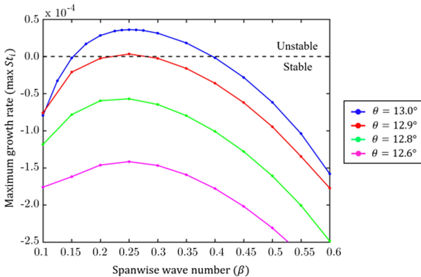
FIG. 11. Maximum growth rate versus spanwise wave number for an oblique shock-wave/laminar-boundary-layer interaction at four different incident shock angles.
