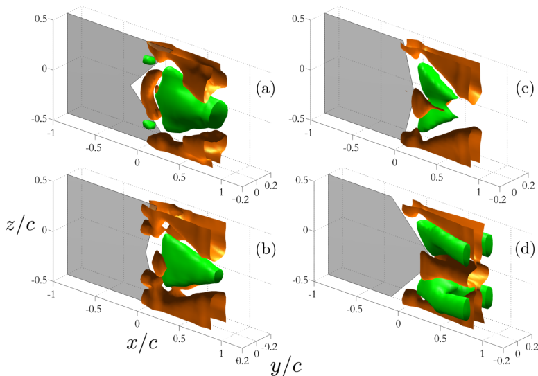
FIG. 6. Isosurfaces of time-averaged streamwise velocity \bar{U}/U_\infty thresholded at 0.92 (orange) and 1.03 (green), for St = 0.2 . (a) \phi = 45^\circ , (b) 75^\circ , (c) 105^\circ , (d) 135^\circ .
