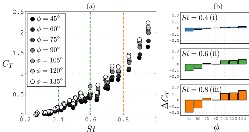
FIG. 9. (a) Thrust coefficient variation with Strouhal number. (b) Change in thrust coefficient relative to the square trailing edge case ( \phi = 90^\circ ), for (i) St = 0.4 , (ii) 0.6 (ii), and (iii) 0.8.
