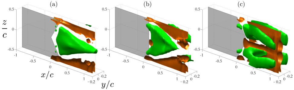
FIG. 5. Isosurfaces of time-averaged streamwise velocity \bar{U}/U_\infty thresholded at 0.92 (orange) and 1.03 (green), for St = 0.2 . (a) \phi = 60^\circ , (b) 90^\circ , (c) 120^\circ . See also Fig. 6.
