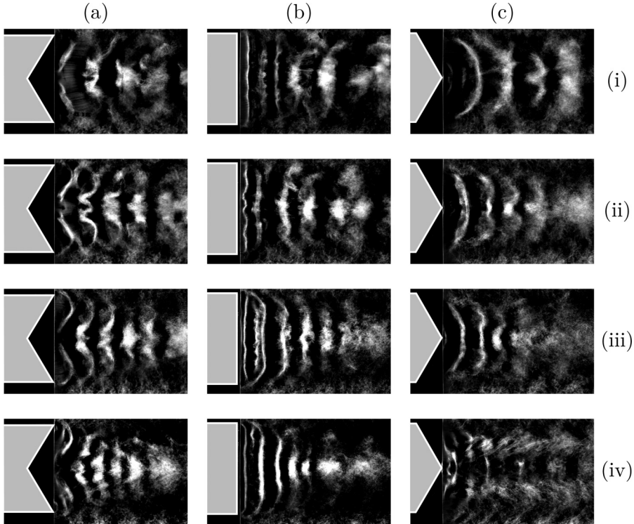
FIG. 8. Phase-averaged hydrogen bubble flow visualizations of the vortex structure for trailing edge angles (a) \phi = 60^\circ , (b) 90^\circ , and (c) 120^\circ . The Strouhal number is fixed St = 0.2 , but it is achieved using different pitch angle and frequency combinations: (i) \theta = 4.3^\circ, k = 8.36 ; (ii) \theta = 3.4^\circ, k = 10.5 ; (iii) \theta = 2.85^\circ, k = 12.57 ; and (iv) \theta = 2.3^\circ, k = 15.71 . Videos are available in the Supplemental Material [14].
