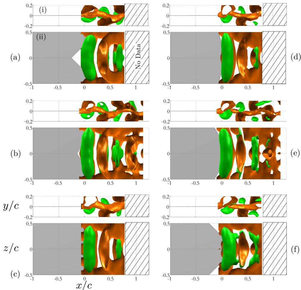
FIG. 7. Isosurfaces of phase-averaged streamwise velocity ( \langle U \rangle / U_\infty = 0.9 , orange; \langle U \rangle / U_\infty = 1.1 , green), for St = 0.2 . Spanwise and panel-normal views are shown for each case. (a) \phi = 45^\circ , (b) 60^\circ , (c) 75^\circ , (d) 105^\circ , (e) 120^\circ , (f) 135^\circ . Each panel is moving into the negative y domain (phase angle 180^\circ ).
