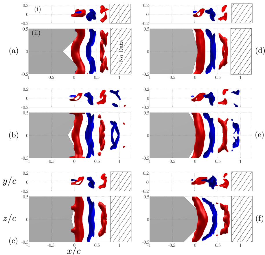
FIG. 4. Isosurfaces of phase-averaged spanwise vorticity ( \langle \omega_z^* \rangle ), for St = 0.2 . Red is positive, blue is negative. Spanwise and panel-normal views are shown for each case. (a) \phi = 45^\circ , (b) 60^\circ , (c) 75^\circ , (d) 105^\circ , (e) 120^\circ , (f) 135^\circ . The panel is moving into the negative y domain (phase angle 180^\circ ). Videos of the phase-averaged vortex time evolution for \phi = 60^\circ , 90^\circ , and 120^\circ are available in the Supplemental Material [14].
