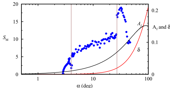
FIG. 8. Variations of S_M with \alpha . The two vertical lines at \alpha = 4^\circ and 27^\circ demarcate three regimes of differing dynamics. Included are the variation of the amplitude of the forcing A_f and the detuning parameter \delta with \alpha (right vertical axis).
