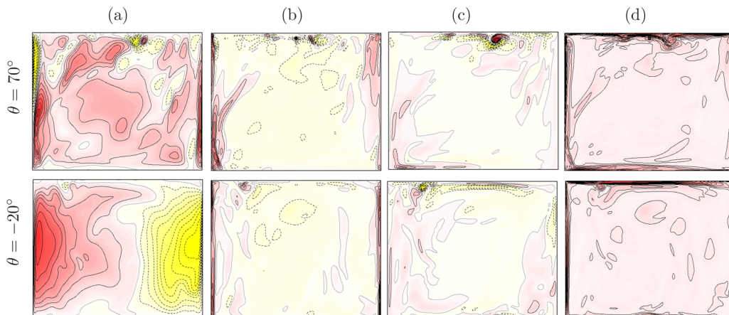
FIG. 10. The SC2 at \alpha = 32^\circ in orthogonal meridional planes; the plane \theta = 70^\circ separates approximately the up and down parts of the overturning flow. There are 20 contours equispaced between the minimum and maximum values in the section for (a) w , (b) \zeta , and (c) \mathcal{H} . (d) For the enstrophy, there are 15 contours quadratically spaced in \mathcal{E} \in (0, 8 \times 10^9) .
