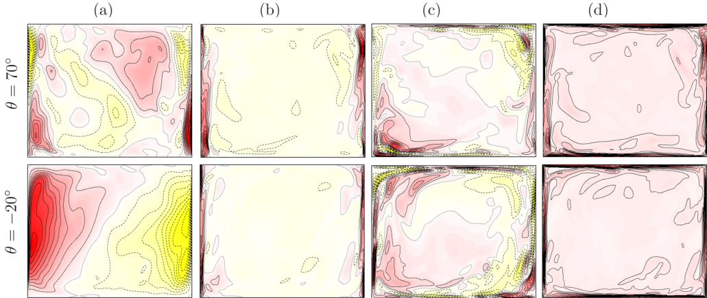
FIG. 12. The SC2 at \alpha = 47^\circ in orthogonal meridional planes; the plane \theta = 70^\circ separates approximately the up and down parts of the overturning flow. There are 20 contours equispaced between the minimum and maximum values in the section for (a) w , (b) \zeta , and (c) \mathcal{H} . (d) For the entrophy, there are 15 contours quadratically spaced in \mathcal{E} \in (0, 8 \times 10^9) .
