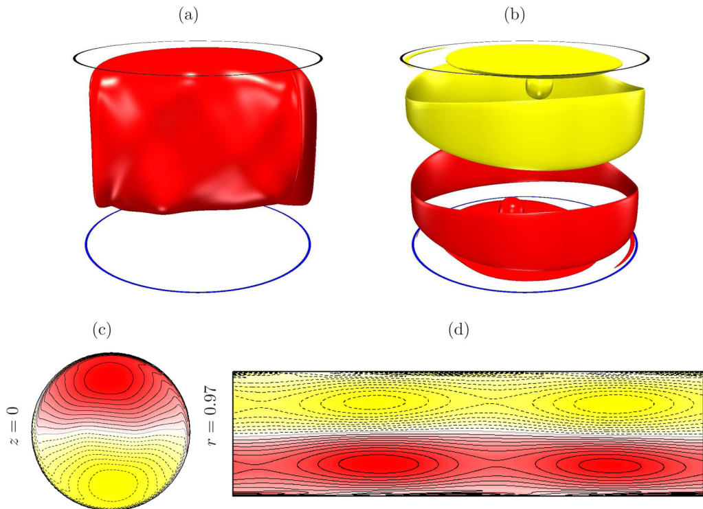
FIG. 2. The BS at \alpha = 1.146^\circ : isosurfaces of (a) w and (b) \mathcal{H} at levels w = 40 and \mathcal{H} = \pm 1.5 \times 10^5 and contours of (c) axial velocity w at midheight z = 0 and (d) helicity \mathcal{H} in (\theta, z) at r = 0.97 .
