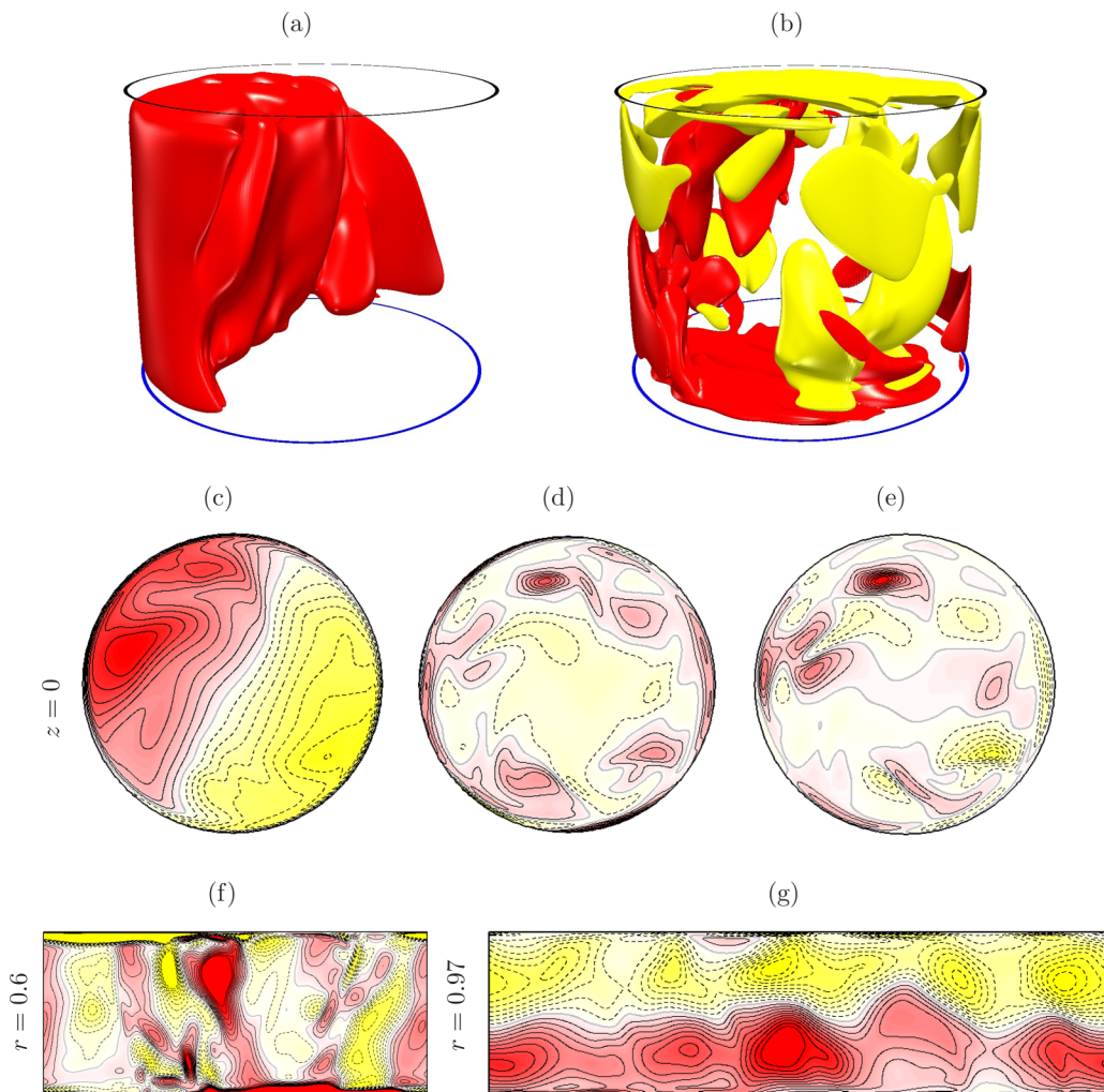
FIG. 7. The SC1 at \alpha = 8.6^\circ : isosurfaces of (a) axial velocity and (b) helicity at levels w = 100 and \mathcal{H} = \pm 2 \times 10^6 (see [29]) and contours of (c) axial velocity, (d) axial vorticity, and (e) helicity at midheight z = 0 ; there are 20 contours equispaced between the minimum and maximum values in the section. Also shown are helicity contours in (\theta, z) at (f) r = 0.6 and (g) r = 0.97 ; there are 20 contours equispaced in the interval \mathcal{H} \in [-4 \times 10^6, 4 \times 10^6] .
