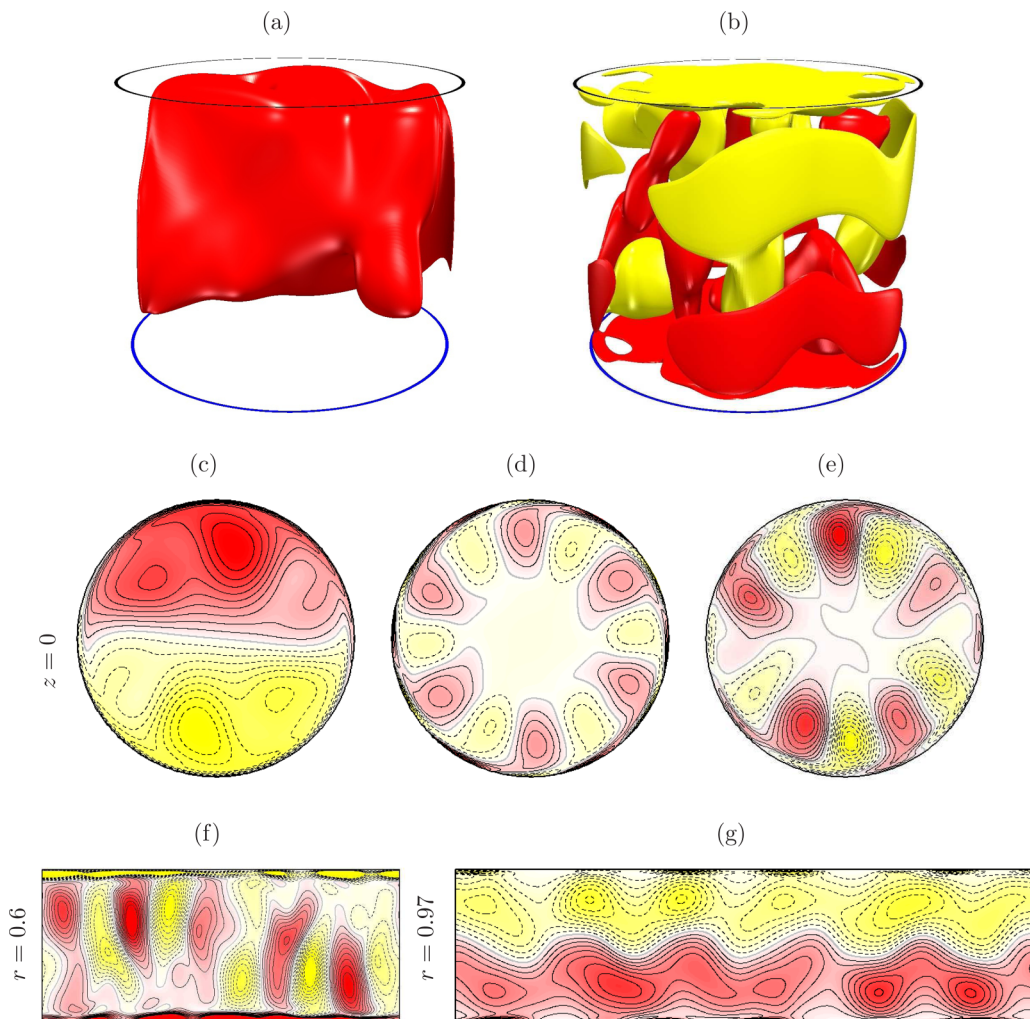
FIG. 3. The LC at \alpha = 1.432^\circ : isosurfaces of (a) axial velocity w and (b) helicity \mathcal{H} at levels w = 50 and \mathcal{H} = \pm 2 \times 10^5 (see [29]) and contours of (c) axial velocity w , (d) axial vorticity \zeta , and (e) helicity \mathcal{H} at midheight z = 0 ; there are 20 equispaced contours between the minimum and maximum values in the section. Also shown are helicity contours in (\theta, z) at (f) r = 0.6 and (g) r = 0.97 ; there are 20 contours equispaced in the interval \mathcal{H} \in [-5 \times 10^5, 5 \times 10^5] .
