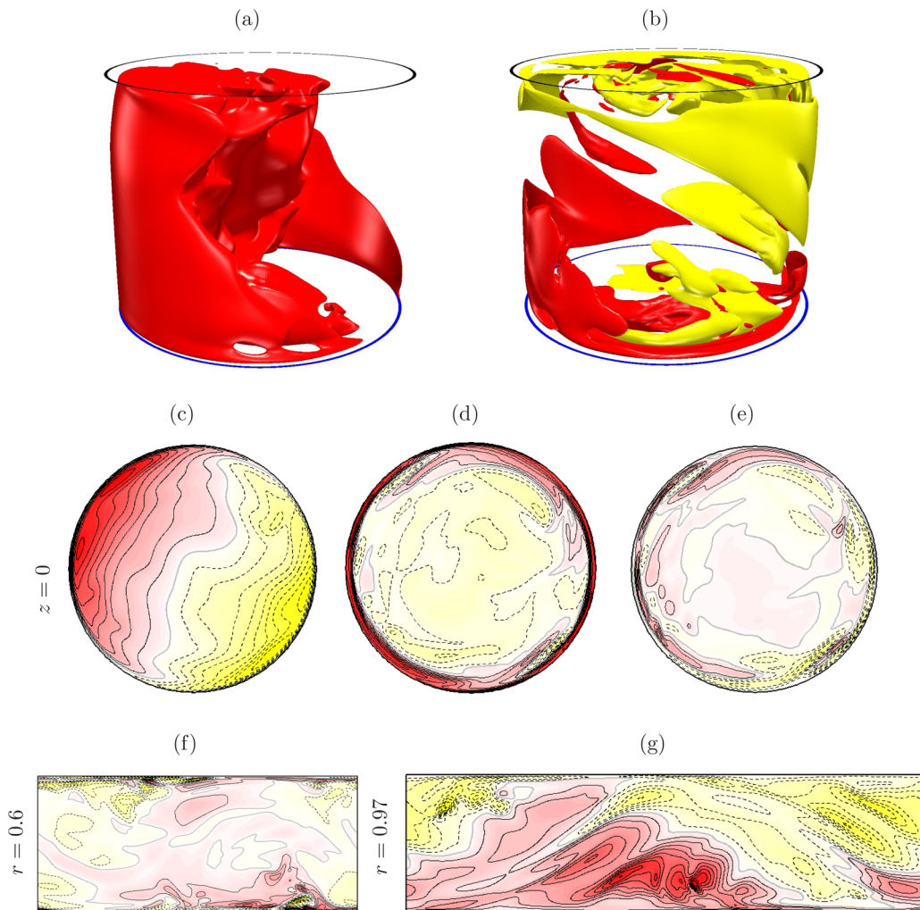
FIG. 11. The SC2 at \alpha = 47^\circ : isosurfaces of (a) axial velocity and (b) helicity at levels w = 100 and \mathcal{H} = \pm 2 \times 10^7 (see [29]) and contours of (c) axial velocity, (d) axial vorticity, and (e) helicity at midheight z = 0 ; there are 20 contours equispaced between the minimum and maximum values in the section for w and \zeta . Also shown are helicity contours in (\theta, z) at (f) r = 0.6 and (g) r = 0.97 ; there are 20 contours equispaced in the interval \mathcal{H} \in [-6 \times 10^7, 6 \times 10^7] for (e)–(g).
