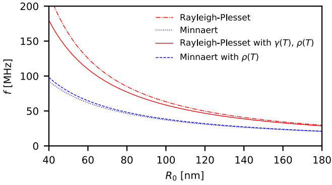
FIG. 6. Resonance frequencies for vapor nanobubbles in pentane, according to the Rayleigh-Plesset and Minnaert models, with and without considering the temperature dependence of the surface tension \gamma and the density \rho .
