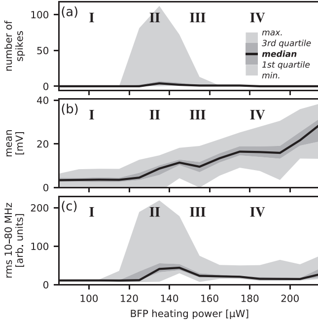
FIG. 4. Dependence of vapor nanobubble behavior on laser power, based on 8050 single-shot time traces measured at one nanoparticle, like those shown in Fig. 3. (a) Number of spikes (extrema d\tilde{u}/dt = 0 where d^2\tilde{u}/dt^2 < 0 is below a heuristically chosen threshold, \tilde{u}(t) being the signal smoothed with a 30 ns Hann filter) in the signal. (b) Mean scattering signal during heating. (c) RMS power of the frequency components between 10 MHz and 80 MHz.
