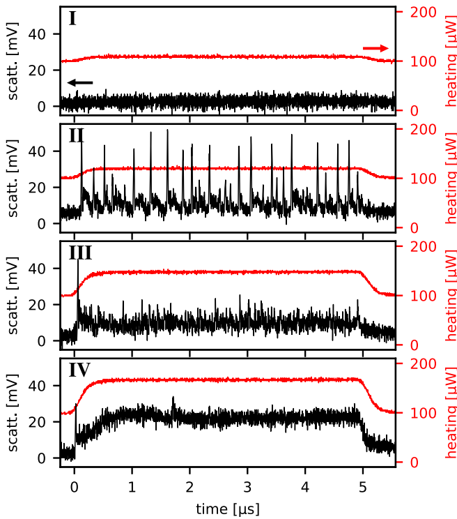
FIG. 3. Single-shot scattering time traces of the same 80 nm Au sphere. Black: scattering in the detector's units; red: heating intensity in the back focal plane. Four principal regimes of heated AuNP behavior are observed: (I) below boiling threshold, small thermal lensing effect. (II) Near boiling threshold, repeated short-lived vapor nanobubble formation. (III) Above boiling threshold, unstable vapor nanobubble for the duration of heating. (IV) Far above threshold, relatively stable nanobubble, probable damage to AuNP. See also Fig. 4.
