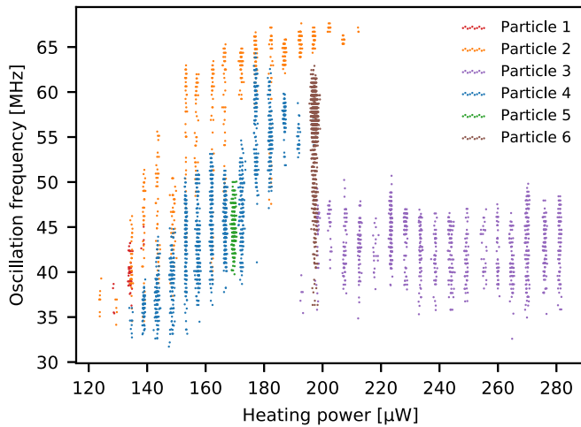
FIG. 8. Change of the apparent oscillation frequency with heating power for different AuNPs. This figure shows the location of peaks in the fast Fourier transforms of individual time traces such as those shown in Fig. 5(b). Only measurements showing good oscillations are shown: those with Q > 10 , where the quality factor Q = f_{\max}/\text{FWHM} is calculated from the FFT. “Particle 4” refers to the set of measurements used in Figs. 5, 7, and 10.
