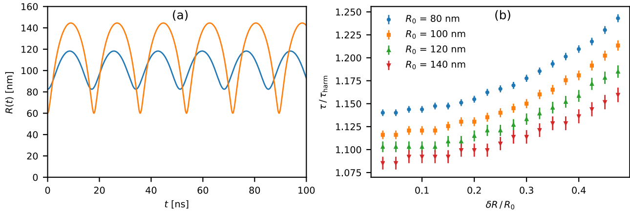
FIG. 9. Anharmonicity of the Rayleigh-Plesset equation for a freely oscillating bubble, with the viscosity set to zero. Calculated by direct numerical (Runge-Kutta) integration with \Delta t = 10 ps using the parameters for saturated pentane. (a) Example time traces of a bubble with R_0 = 120 nm oscillating at two different amplitudes. The bottom of the curve, especially at larger amplitude, is noticeably more “pointed,” and the oscillation period is clearly different. (b) Calculated oscillation periods \tau with different equilibrium radii R_0 and oscillation amplitudes \delta R , relative to the corresponding period \tau_{\text{harm}} in the harmonic approximation.
