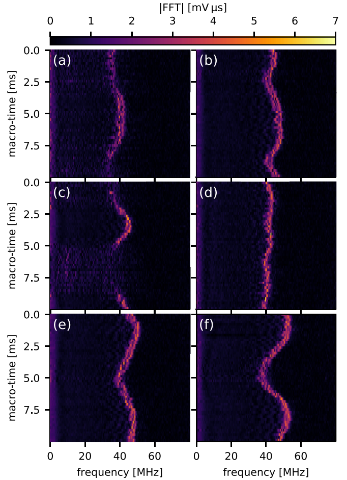
FIG. 7. Example series of oscillating-bubble event Fourier transforms, all for the same nanoparticle, in the same form as Fig. 5(b).
