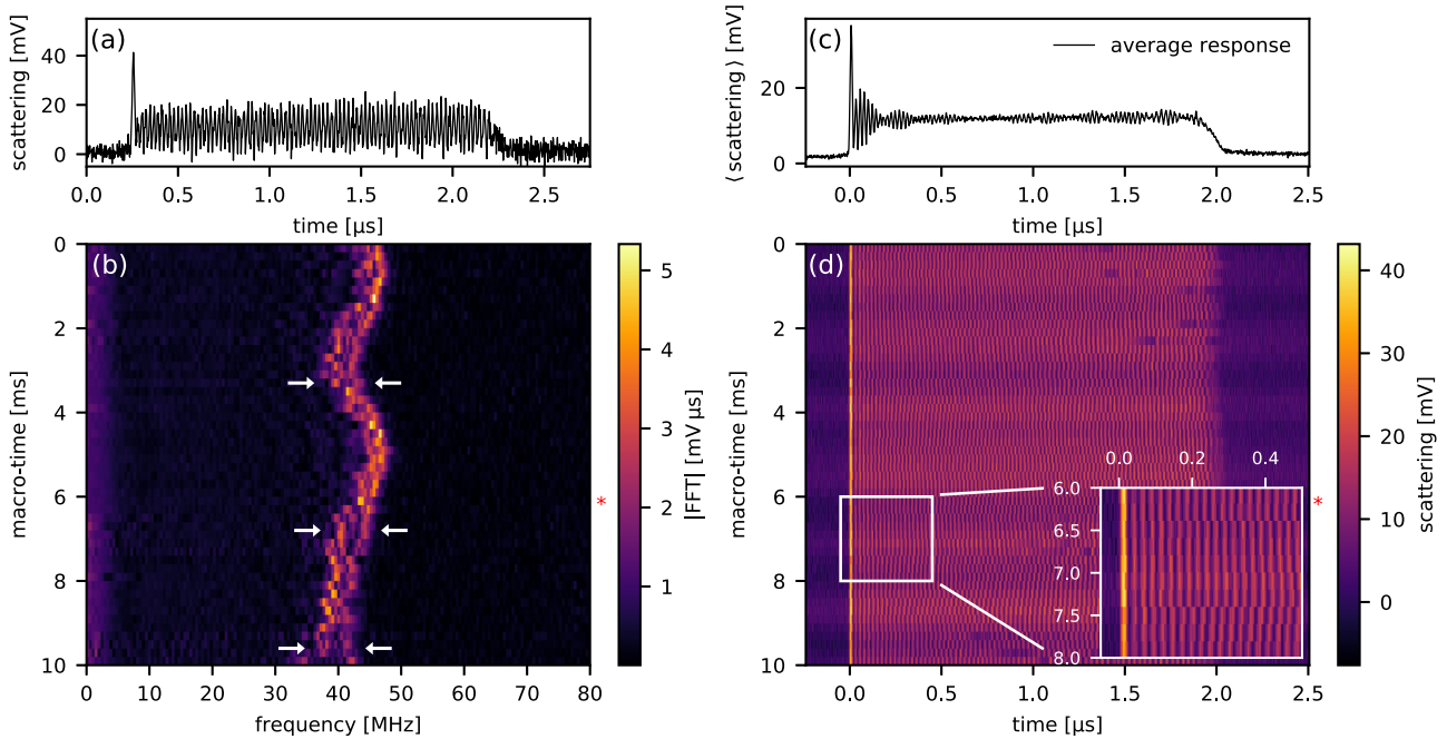
FIG. 5. Nanobubble oscillations; (a) Single-shot nanobubble timetrace with clearly visible oscillations. (b) Fourier transforms of 50 subsequent such time traces of the same AuNP subject to an unchanging heating profile. White arrows highlight some points with particularly clear frequency splitting. (c) Average of the time traces in panel (d), synchronized on the initial rising edge. (d) Fifty time traces used in panels (b) and (c). In panels (b) and (d), the lines marked with an asterisk correspond to panel (a).
