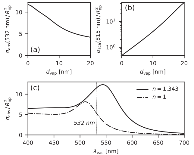
FIG. 2. Layered-sphere Mie theory calculation [22] with an 80 nm diameter gold core and a vacuum shell (bubble, n = 1 ) of varying thickness d_{\text{vap}} in a medium with refractive index n = 1.33 . (a) Absorption of \lambda_{\text{vac}} = 532 nm and (b) scattering of \lambda_{\text{vac}} = 815 nm, both shown as a function of bubble thickness. (c) Absorption spectra of 80 nm AuNPs, when in n -pentane as compared to vacuum. See also Appendix A.
