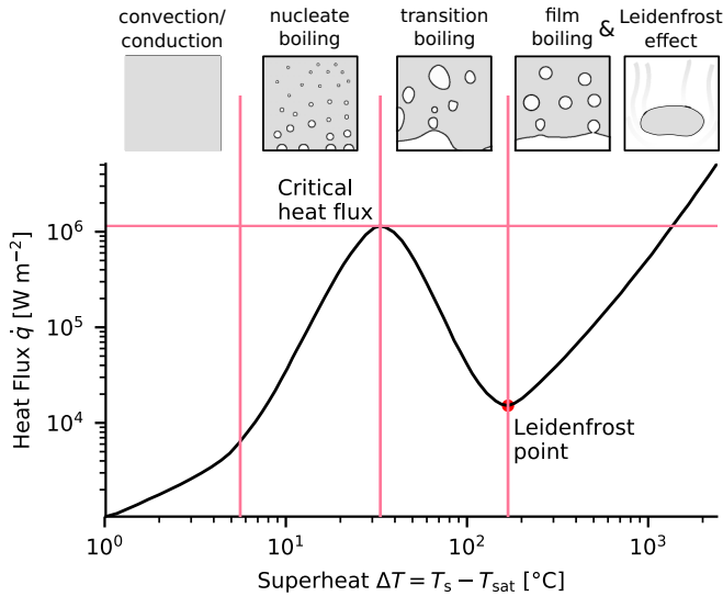
FIG. 1. The well-known traditional boiling curve of macroscopic pools of water at atmospheric pressure with sketches of the different boiling regimes. Curve data adapted from Ref. [4].
