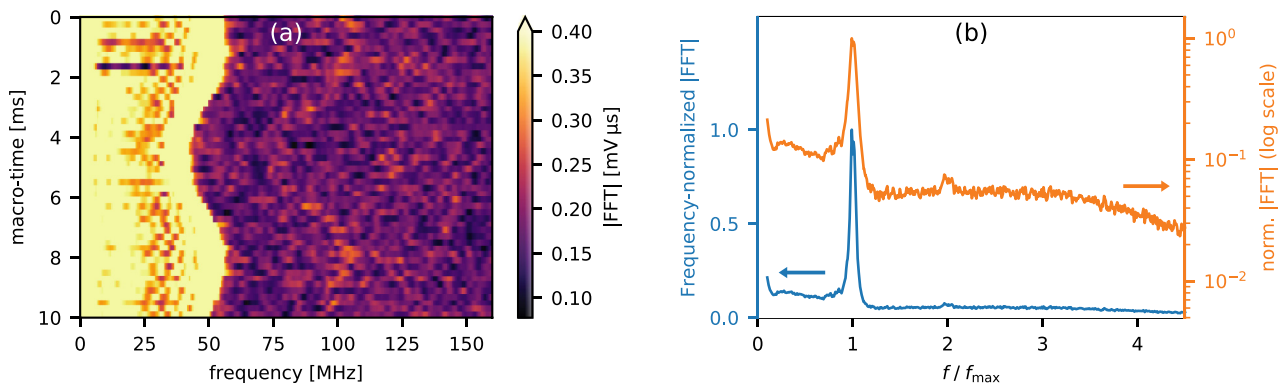
FIG. 10. (a) Series of oscillating-bubble event Fourier transforms [same data as Fig. 7(f), smoothed with a 6 MHz Hann filter] showing, faintly, the second harmonic. (b) Mean of the Fourier transforms shown, calculated after rescaling the frequency axis of each to put the maximum at unity, showing clearly the second harmonic. Note that the upper cutoff frequency of our detector is 80 MHz, which reduces the apparent prominence of the second harmonic, and completely obscures higher harmonics.
