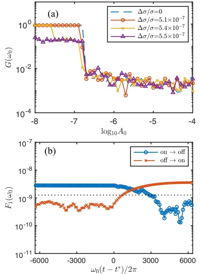
FIG. 15. (a) The gain G(\omega_0) [defined in Eq. (4)] plotted as a function of the driving amplitude A_0 at fixed driving frequency \omega_0 = 16.0 for a device with a single control particle at \Delta\sigma/\sigma = 0 (dashed line), 5.1 \times 10^{-7} (circles), 5.4 \times 10^{-7} (Xs), and 5.5 \times 10^{-7} (triangles), using damping parameter b = 10^{-3} . (b) The Fourier transform F_1(\omega_0) of the x displacement of disk 1 as a function of time \omega_0(t - t^*)/2\pi when switching the device from the on ( \Delta\sigma/\sigma = 0 ) to off ( \Delta\sigma/\sigma = 5.4 \times 10^{-7} ) state (circles) and vice versa (Xs) at time t^* using a single control particle and damping parameter b = 10^{-3} . The driving frequency and amplitude are \omega_0 = 16.0 and A_0 = 6.3 \times 10^{-8} , respectively.
