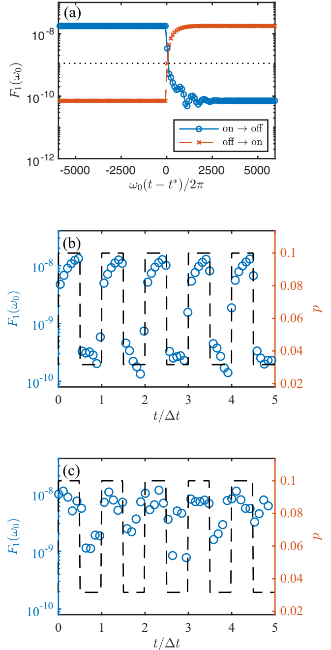
FIG. 11. (a) The Fourier transform F_1(\omega_0) of the x displacement of disk 1 as a function of time \omega_0(t-t^*)/2\pi when switching the device at time t^* from the “on” (pressure p = 10^{-1} ) to “off” ( p = 3.2 \times 10^{-2} ) states (circles) and vice versa (Xs) using a damping coefficient b = 10^{-2} . The horizontal dotted line indicates the geometric mean \bar{F}_1(\omega_0) of the on and off values of F_1(\omega_0) . The switching times t_s are obtained by finding when F_1(\omega_0) crosses \bar{F}_1(\omega_0) . (b) The Fourier transform F_1(\omega_0) (open circles and left axes labels) of the x displacement of disk 1 as a function of time t/\Delta t (after reaching an initial steady state at t = 0 ) during continuous switching of the device between the “on” and “off” states using b = 10^{-2} . The pressure of the device (dashed line and right axes labels) follows a square-wave signal with \Delta t/t_s \approx 3.7 . (c) Same as (b) except \Delta t/t_s \approx 0.7 .
