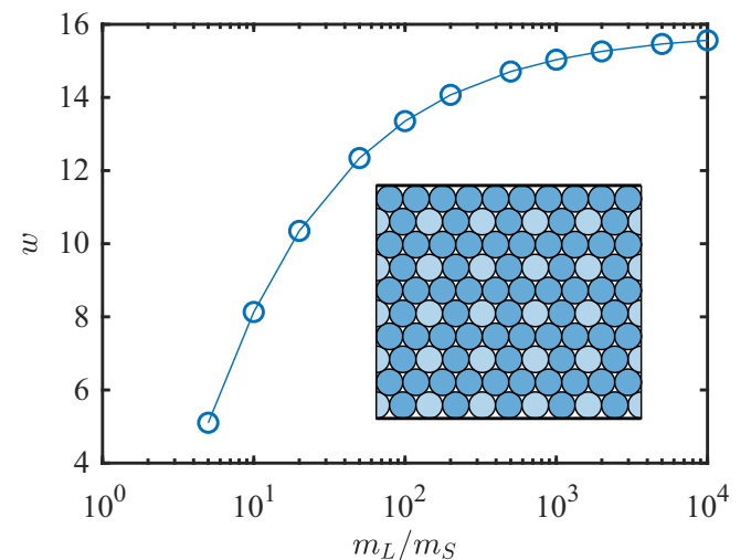
FIG. 4. The width w of the maximum band gap in the eigenfrequency spectrum of the mass-weighted dynamical matrix for the configuration in Fig. 2(d) (and inset) as a function of the mass ratio m_L/m_S .
