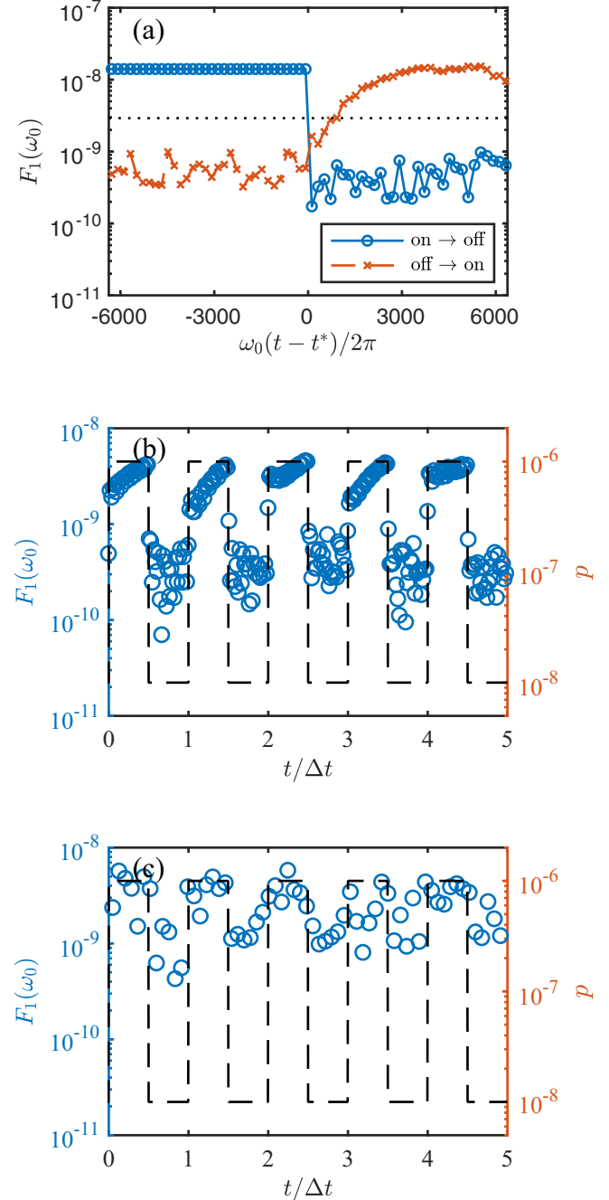
FIG. 13. (a) The Fourier transform F_1(\omega_0) of the x displacement of disk 1 as a function of time \omega_0(t - t^*)/2\pi when switching the device from the “on” (pressure p = 10^{-6} ) to “off” ( p = 10^{-8} ) states (circles) and vice versa (Xs) at time t^* using a damping coefficient b = 10^{-3} . The driving frequency and amplitude are \omega_0 = 16.0 and A_0 = 3.2 \times 10^{-7} . (b) The Fourier transform F_1(\omega_0) of the x displacement of disk 1 (circles and left axes labels) as a function of time t/\Delta t when continuously switching the device between the “on” and “off” states using b = 10^{-3} . The dashed line shows the pressure of the device (right axes labels), which has a square-wave form with \Delta t/t_s \approx 2.7 (where t_s is the time for the device to switch from the off to the on states). (c) Same as (b) except \Delta t/t_s \approx 0.68 . For (a)–(c), the off and on states possess different interparticle contact networks.
