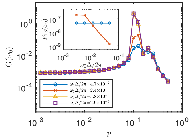
FIG. 21. The gain G(\omega_0) for the acoustic device as a function of pressure p (for a system with no contact breaking) measured with system with sampling interval \omega_0 \Delta/2\pi = 4.7 \times 10^{-2} (circles), 2.4 \times 10^{-2} (Xs), 5.8 \times 10^{-3} (triangles), and 2.9 \times 10^{-3} (squares). The inset shows the Fourier transforms of the output and input signals, F_1(\omega_0) (Xs) and F_3(\omega_0) (circles), as a function of \omega_0 \Delta/2\pi for the device with pressure p = 10^{-1} . For all data, \omega_0 = 14.9 , A_0 = 10^{-6} , b = 10^{-3} , and the total simulation time \omega_0 T/2\pi = 5.9 \times 10^4 .
