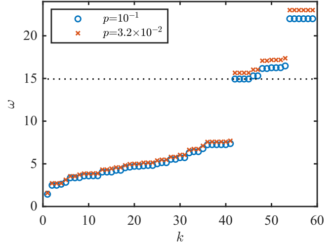
FIG. 7. The eigenfrequencies of the mass-weighted dynamical matrix plotted in increasing order with index k for the acoustic device in Fig. 6 at pressure p = 10^{-1} (the “on” state, circles) and 3.2 \times 10^{-2} (the “off” state, Xs). The horizontal line at \omega = 14.9 indicates a potential driving frequency that yields a large gain ratio between the on and off states.
