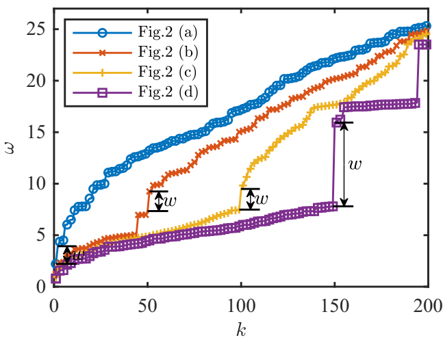
FIG. 3. Eigenfrequencies of the mass-weighted dynamical matrix \omega_k , sorted in ascending order and indexed by k , for the N = 100 configurations in Fig. 2. (a) Circles, (b) Xs, (c) pluses, and (d) squares with periodic and fixed boundary conditions in the x and y directions, respectively. w indicates the maximum band gap in the eigenfrequency spectrum.
