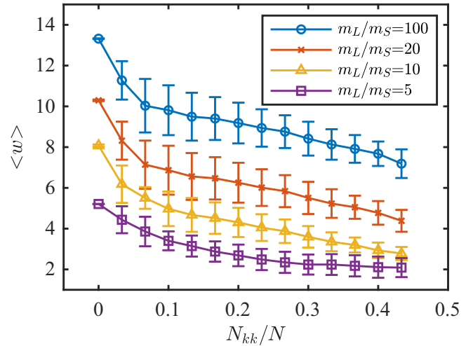
FIG. 18. The average maximum difference between adjacent eigenfrequencies \langle w \rangle of the mass-weighted dynamical matrix versus the number of contacts between the grains with knobs N_{kk}/N for a hexagonal packing with N_L = 21 and N_S = 9 and mass ratio m_L/m_S = 100 (circles), 20 (Xs), 10 (triangles), and 5 (squares). The means and standard deviations (error bars) are obtained by averaging over 50 configurations in which the masses of the grains are chosen randomly as either m_L and m_S to yield a given N_{kk}/N .
