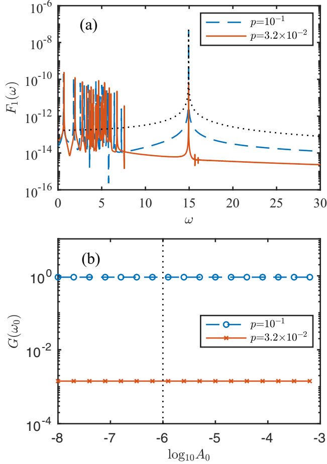
FIG. 8. (a) The Fourier transform F_1(\omega) of the x displacement of disk 1 for the acoustic device with pressure p = 10^{-1} (dashed line) and 3.2 \times 10^{-2} (solid line) obtained by driving disk 3 sinusoidally with amplitude A_0 = 10^{-6} and frequency \omega_0 = 14.9 . The dotted line shows the Fourier transform F_3(\omega) of the x displacement of the input disk 3. (b) The gain G(\omega_0) [defined in Eq. (4)] plotted as a function of the driving amplitude A_0 with driving frequency \omega_0 = 14.9 for the device at pressure p = 10^{-1} (open circles) and 3.2 \times 10^{-2} (Xs).
