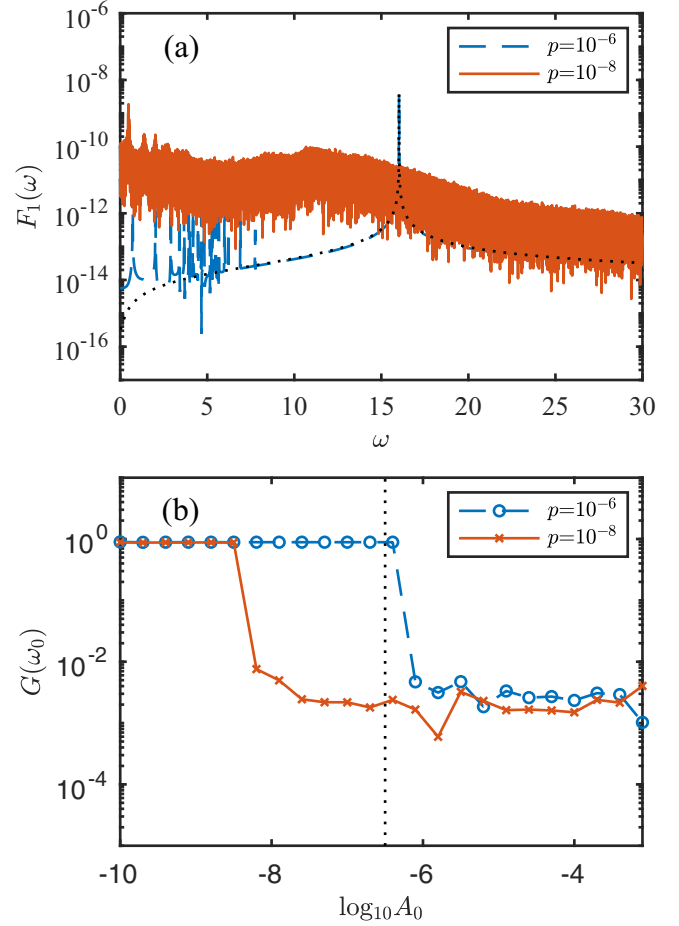
FIG. 12. (a) The Fourier transform F_1(\omega) of the x displacement of disk 1 for the device with pressure p = 10^{-6} (dashed line) and 10^{-8} (solid line) obtained by driving disk 3 sinusoidally with amplitude A_0 = 3.2 \times 10^{-7} and frequency \omega_0 = 16.0 , using damping coefficient b = 10^{-3} . The dotted line shows the Fourier transform F_3(\omega) of the x displacement of the input disk 3. (b) The gain G(\omega_0) [defined in Eq. (4)] plotted as a function of the driving amplitude A_0 with driving frequency \omega_0 = 16.0 for a device at pressure p = 10^{-6} (dashed line) and 10^{-8} (solid line), using damping parameter b = 10^{-3} . The vertical dotted line indicates the amplitude of the driving A_0 = 3.2 \times 10^{-7} in (a).
