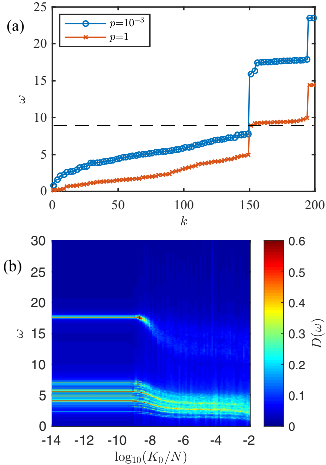
FIG. 5. (a) Spectrum of eigenfrequencies of the mass-weighted dynamical matrix sorted in ascending order with index k for systems with N = 100 disks, m_L/m_S = 10 , and arranged on a hexagonal lattice in the optimal configuration in Fig. 2(d) at pressure p = 10^{-3} (circles) and 1 (Xs). The dashed line indicates a driving frequency at which the acoustic switch can operate. (b) The Fourier transform of the velocity correlation function D(\omega) for the mechanically stable packing in Fig. 2(d) at pressure p = 10^{-4} after adding velocities to all grains such that the eigenfrequencies of the mass-weighted dynamical matrix are included with equipartition of the total kinetic energy K_0 . The color scale from dark red to violet represents decreasing D(\omega) on a linear scale.
