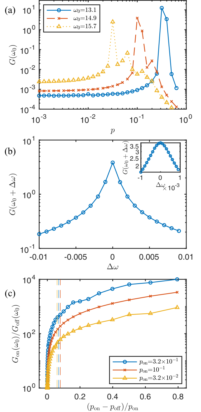
FIG. 9. (a) The gain G(\omega_0) for the acoustic device as a function of pressure p for three values of the driving frequency \omega_0 = 13.1 (circles), 14.9 (Xs), and 15.7 (triangles). (b) The gain G(\omega_0 + \Delta\omega) over a small frequency range \Delta\omega near the driving frequency \omega_0 = 14.9 . The inset is a close-up of the gain to within 10^{-3} of \omega_0 . (c) The gain ratio G_{\text{on}}(\omega_0)/G_{\text{off}}(\omega_0) as a function of the normalized change in pressure between the on and off states, (p_{\text{on}} - p_{\text{off}})/p_{\text{on}} , for p_{\text{on}} = 3.2 \times 10^{-1} (circles), 10^{-1} (Xs), and 3.2 \times 10^{-2} (triangles) and the sizes of all particles are changed to control the pressure. The vertical dashed lines indicate the value of (p_{\text{on}} - p_{\text{off}})/p_{\text{on}} at which contacts would begin breaking if the size of only a single particle was changed to control the pressure. For all data, the driving amplitude is A_0 = 10^{-6} and the damping parameter b = 10^{-3} .
