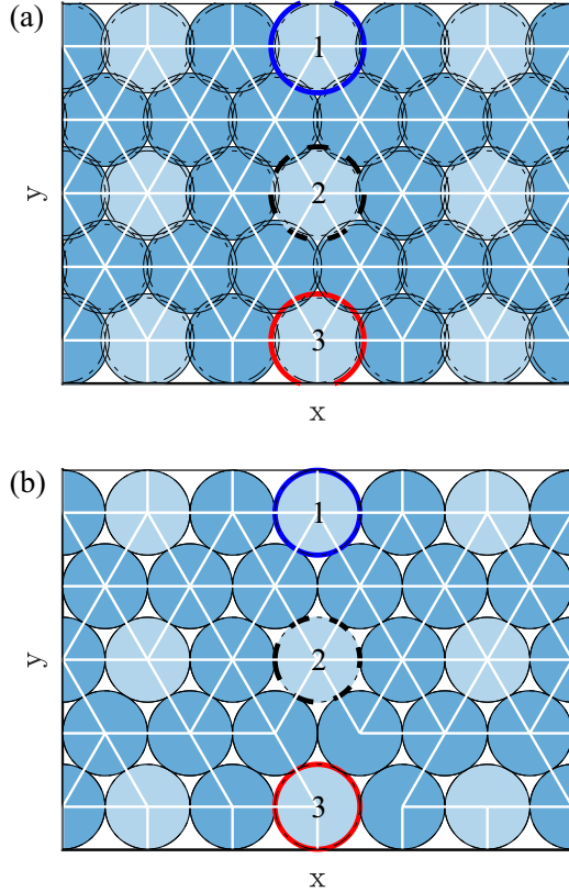
FIG. 6. (a) An illustration of a three port acoustic switch with fixed, flat boundary conditions in the y direction and periodic boundary conditions in the x direction. The device includes N = 30 disks (with N_L = 21 (dark), N_S = 9 (light), and m_L/m_S = 10 ) arranged on a hexagonal lattice. The solid white lines indicate the N_c = 90 distinct contacts between disks. Disk 3 is the input port, indicating where the system will be driven. The gain of the system is measured via the output port, labeled disk 1. The switch can be turned on and off by varying the pressure of the system through port 2, e.g., by changing the size of a single disk or all disks in the system. Here, the device changes from pressure p = 10^{-6} (dashed outline) to 10^{-1} (solid outline) when all disks increase in size. (b) Illustration of the device in (a) at p = 10^{-6} with disk 3 driven at A_0 = 10^{-6} and frequency \omega_0 = 16.0 , which causes contact breaking. In this snapshot, the device has four fewer contacts than in (a). The central grain with the dashed outline provides the pressure control when we use single-particle control for port 2.
