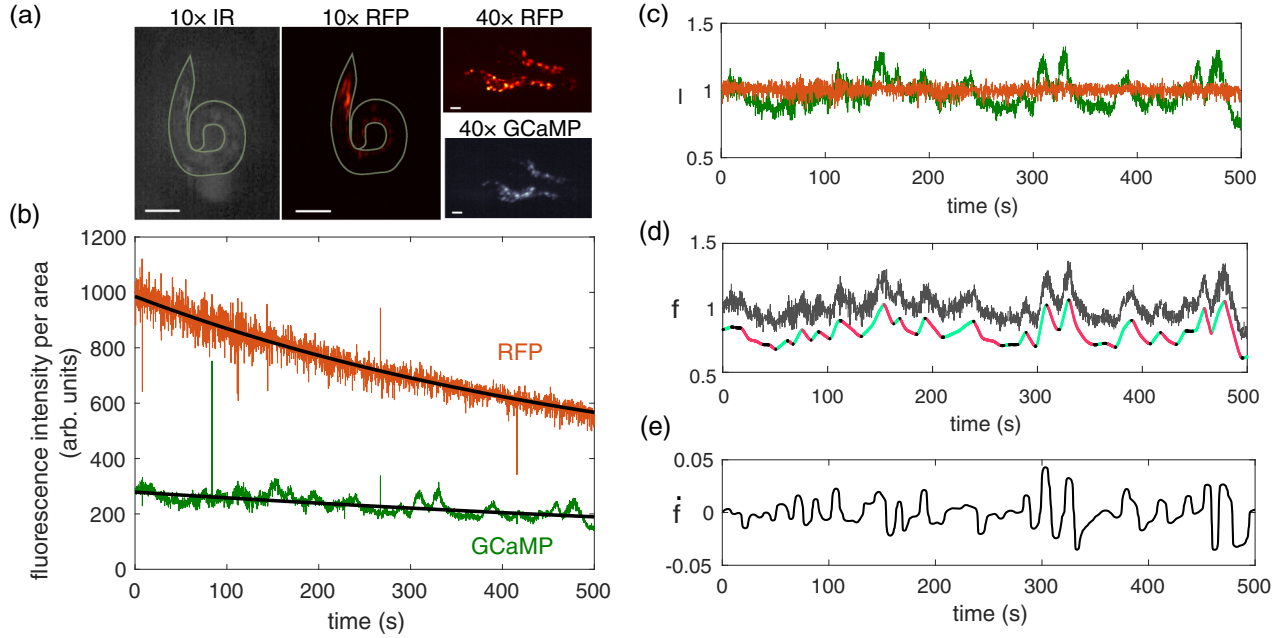
FIG. 1. Schematics of data acquisition and processing. (a) Examples of the raw images acquired through the 10 \times (scale bar equals 100 \mu\text{m} ) and 40 \times (scale bar equals 10 \mu\text{m} ) objectives. The body of the nematode is outlined with light green curves. As an example, we show for one neuron that (b) the intensity of the nuclei-localized fluorescent protein tags—the calcium-sensitive GCaMP and the control fluorophore RFP—are measured as functions of time. Photobleaching occurs on a longer timescale than the intracellular calcium dynamics, which allows us to perform photobleaching correction by dividing the raw signal with its exponential fit, resulting in the signals of panel (c). (d) The normalized ratio of the photobleaching-corrected intensity, f , is a proxy for the calcium concentration in each neuron nuclei (dark gray). As described in the text, this signal is discretized using the denoised time derivative \hat{f} ; we use three states, marked as red, blue, and black after smoothing (lightly offset for ease of visualization). (e) The time derivative \dot{\hat{f}} , extracted using total-variation regularized differentiation.
