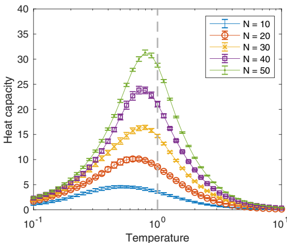
FIG. 9. The heat capacity is plotted against temperature for models with different number of neurons, N . The maximum of the heat capacity approaches the operational temperature of the C. elegans neural system T_0 = 1 from below as N increases. Error bars are the standard error across 10 random subgroups of N neurons.
