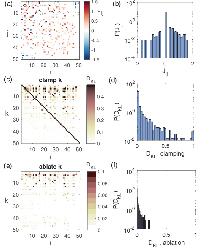
FIG. 11. Local perturbation of the neural network leads to global response. (a), (b) For a typical group of N = 50 neurons, the inferred interaction matrix J is sparse. Here, the neuron indexes i and j are sorted based on m_i^{\text{flat}} , as in Fig. 4. (c), (d) When neuron k is clamped to a constant voltage, the Kullback-Leibler divergence (in bits) of the marginal distribution of states for neuron i is distributed throughout the network. (e), (f) When neuron k is ablated, the D_{\text{KL}} is also distributed throughout the network, but is smaller than in response to clamping.
