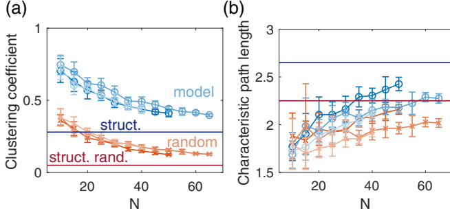
FIG. 10. The topology of the learned maximum entropy model approaches that of the structural connectome, as the number of neurons being modeled, N , increases. The two global topological properties being measured are the clustering coefficient C [panel (a)] and characteristic path length L [panel (b)]. Here, the inferred network topology for three different worms is plotted in blue circles. Red crosses are for the randomized network with the same number of neurons, N , and number of connections, N_E , as the model, where we expect L_{\text{random}} \sim \ln(N)/\ln(2N_E/N) and C_{\text{random}} \sim 2N_E/N^2 . The dark blue line corresponds to the network property of the structural connectome; the dark red line corresponds to randomized network with number of nodes and edges equal to those of the structural connectome [45]. Error bars are generated from the standard deviation across different 10 subgroups of N neurons.
