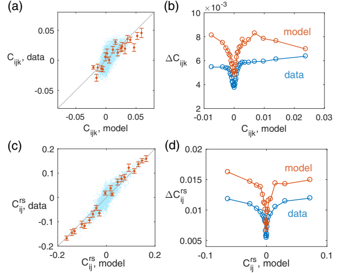
FIG. 6. Model validation: The model predicts unconstrained higher order correlations of the data. Panel (a) shows the comparison between model prediction and data for the connected three-point correlation C_{ijk} for a representative group of N = 50 neurons. All 19 800 possible triplets are plotted with the blue dot. Error bars are generated by bootstrapping random halves of the data, and are shown for 20 uniformly spaced random triplets in red. Panel (b) shows the error of three-point function \Delta C_{ijk} as a function of the connected three-point function C_{ijk} , binned by its value predicted by the C_{ijk} model. The red curve is the difference between data and model prediction. The blue curve is the standard error from mean of C_{ijk} over the course of the experiment, extracted by bootstrapping random halves of the experiment. Panels (c) and (d) are the same as panels (a) and (b), but for the connected two-point correlation tensor C_{ij}^{\text{rs}} .
