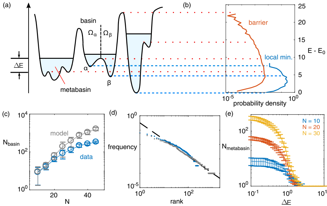
FIG. 8. Energy landscape of the inferred maximum entropy model. (a) Schematic of the energy landscape with local minima \alpha, \beta and the corresponding basin \Omega_\alpha, \Omega_\beta . Colored in light blue is the metabasin formed at the given energy threshold, \Delta E . (b) Typical distribution of the value of the energy minima and the barriers of a maximum entropy model on N = 30 neurons. The global energy minimum, E_0 , is subtracted from the energy, E . (c) The number of energy minima increases subexponentially as number of neurons included in the model increases. Error bars are the standard deviation of 10 different subgroups of N neurons. (d) The rank-frequency plot for frequency of visiting each basin matches well between data and model for a typical subgroup of 40 neurons. (e) The number of metabasins, grouped according to the energy barrier, diverges when the energy threshold \Delta E approaches 1 from above.
