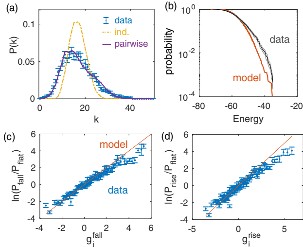
FIG. 7. Model validation: Comparison between model prediction and data for observables not constrained by the model. The neuron network has N = 50 neurons. (a) Probability of k neurons being in the same state. Blue dots are computed from the data. Yellow dash-dotted line is the prediction from a model in which all neurons are independent, generated by applying a random temporal cyclic permutation to the activity of each neuron. Purple line is the prediction of the pairwise maximum entropy model. (b) Tail distribution of the energy for the data and the model. All error bars in this figure are extrapolated from bootstrapping. (c), (d) Probability ratio of the state of a single neuron as a function of the effective field g_i^f , binned by the value of the effective field. Error bars are the standard deviation after binning.
