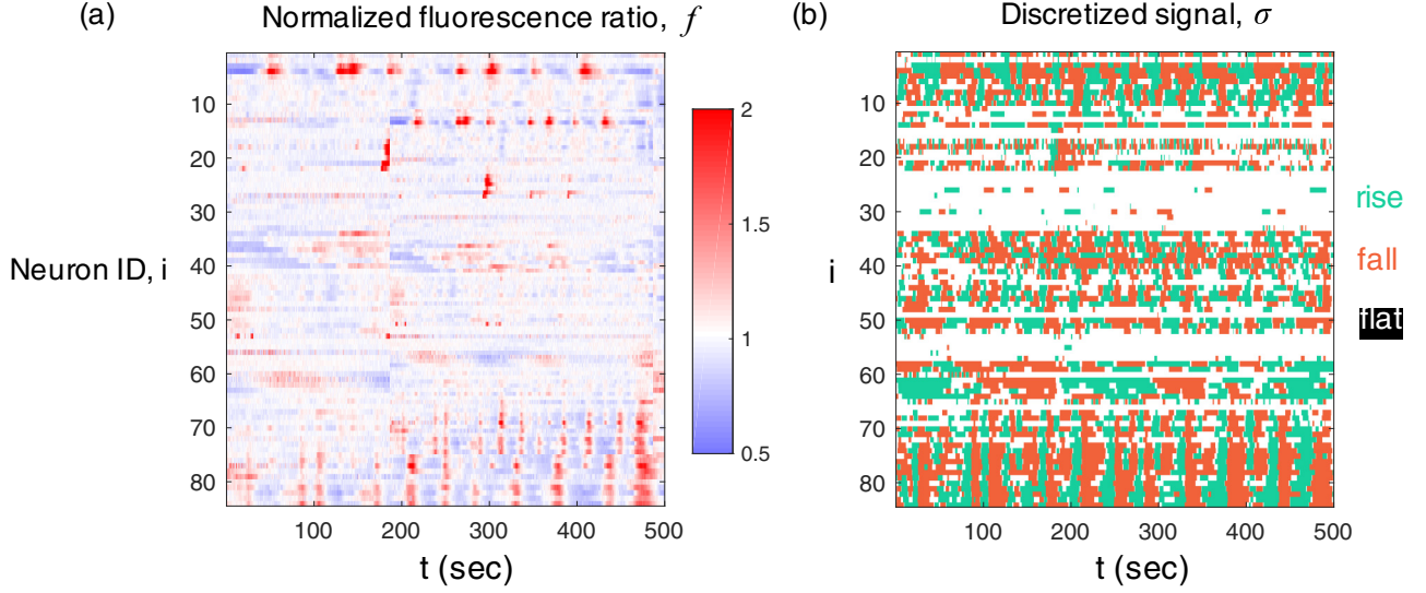
FIG. 3. Discretization of the empirically observed fluorescence signals. (a) Heat map of the normalized fluorescence ratio between photobleaching-corrected GCaMP fluorescence intensity and RFP fluorescence intensity, f , for each neuron as a function of time. (b) Heat map of the neuronal activity after discretization based on time derivatives of f . Green corresponds to a state of “rising,” red “falling,” and white “flat.”
