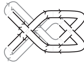
Diagram 7 with weight N^4 and multiplicity 1:
