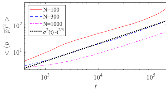
FIG. 3. Evolution of \langle (p - \bar{p})^2 \rangle for different system sizes and the subdiffusive behavior prediction, Eq. (13). The system is initially in a WB state with \Delta p = 0.5 .
