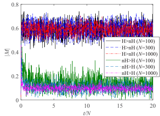
FIG. 4. Evolution of magnetization for a configuration where the Hamiltonian coupling is stronger than the nonsymmetric one ( \Delta = -2\kappa and -2g^2\kappa/(\kappa^2 + \Delta^2) = 1 , labeled “H > nH”), and for the opposite configuration ( \Delta = -\kappa/2 and -2g^2\kappa/(\kappa^2 + \Delta^2) = 1 , labeled “nH > H”), for different system sizes. The system is initially in a WB state with \Delta p = 0.5 .
