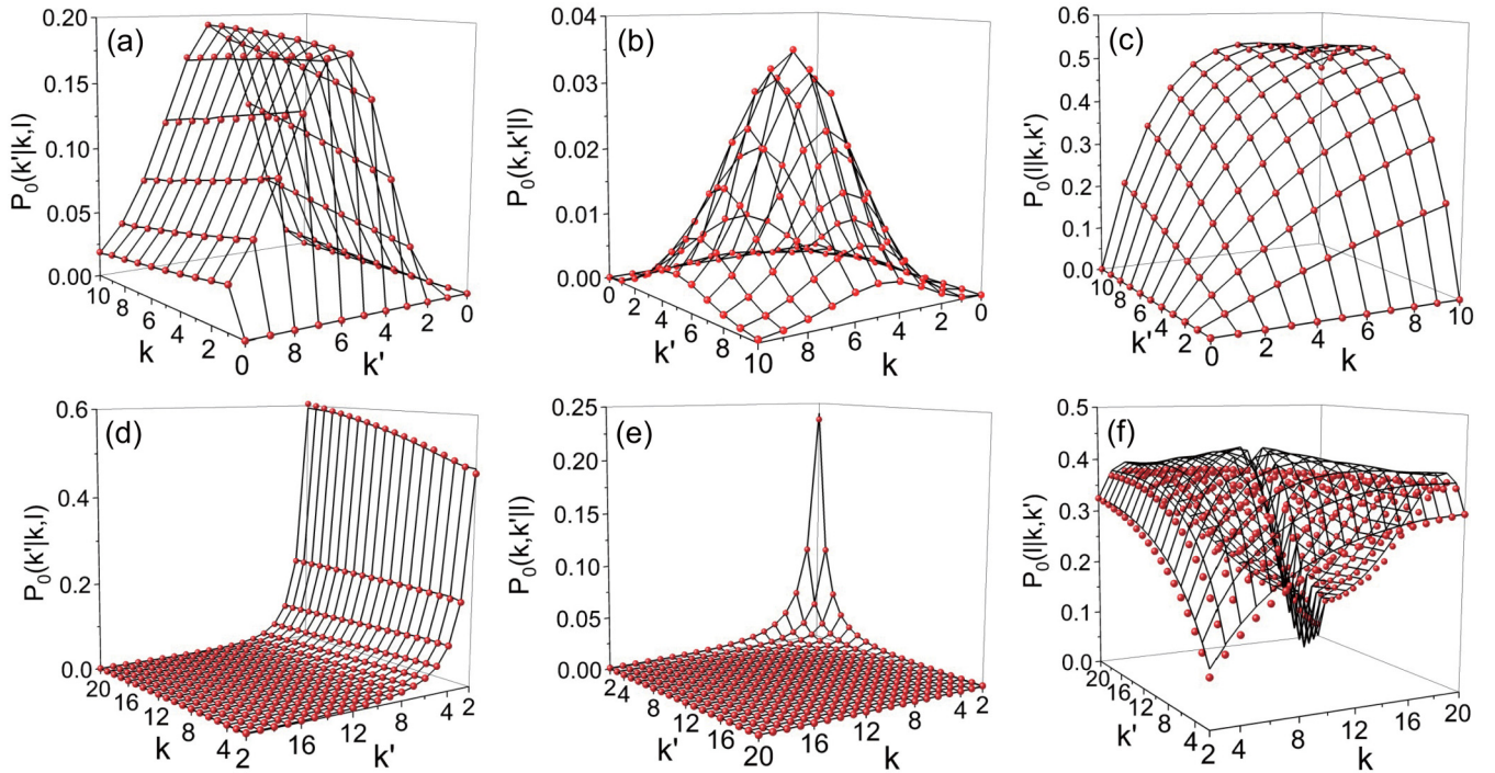
FIG. 1. Probability distributions P_0(k'|k,l) , P_0(k,k'|l) , and P_0(l|k,k') as functions of k and k' for l = 4 and N = 1000 . Wireframes indicate the distributions calculated analytically by the method explained in Sec. III B, and dots represent those measured for numerically realized random networks. Upper three panels [(a)–(c)] are the results for Erdős-Rényi random graphs with \langle k \rangle = 5.0 , and lower panels [(d)–(f)] for scale-free random networks with the degree distribution P(k) \propto k^{-3} .
