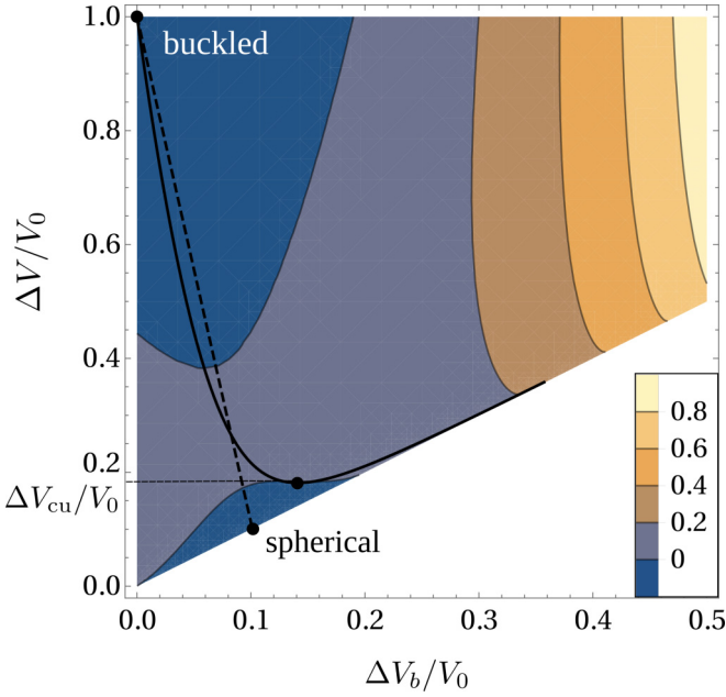
FIG. 7. Contour plot of Pogorelov enthalpy F(p, \Delta V_b, \Delta V)/Y R_0^2 as a function of precompression volume \Delta V_b of the spherical capsule body and total volume deficit \Delta V with \Delta V_b \leq \Delta V ( \gamma = 100 , p R_0/Y = 0.15 > p_{c1} , \nu = 1/2 , F in units of Y R_0^2 ). Solid black lines represent local minima and maxima as a function of \Delta V_b , which only exist above the critical unbuckling volume deficit \Delta V_{cu} . Along the dashed path from the metastable spherical shape to the buckled shape, the energy barrier F_B from Eq. (29) has to be overcome.
