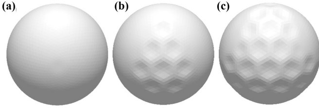
FIG. 12. Postbuckling shapes obtained from numerical energy minimization with a constrained variance \Delta R^2 and unconstrained z for (a) \Delta R^2/R_0^2 = 1.3 \times 10^{-7} , (b) \Delta R^2/R_0^2 = 1.5 \times 10^{-5} , and (c) \Delta R^2/R_0^2 = 4.7 \times 10^{-5} for p/p_c = 0.85 .
