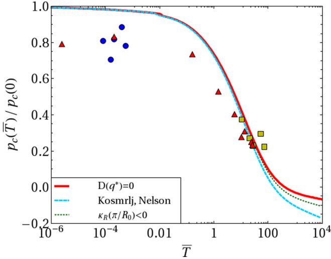
FIG. 3. Critical buckling pressure p_c(T) as a function of the dimensionless temperature \bar{T} = k_B T \sqrt{\gamma} / \kappa according to the buckling criterion D_R(q^*) = 0 (dark red solid line) and according to the criterion p_R(q^*) = p_{c,R}(q^*) from Košmrlj and Nelson [44] (light blue dashed line). The criterion p_R(q^*) = p_{c,R}(q^*) gives slightly smaller values of p_c(T) but both criteria lead to p_c(T) < 0 for high temperatures, signaling that fluctuating shells can spontaneously buckle even without external compressive pressure. We also show the pressure where \kappa first renormalizes to zero at the largest scale, \kappa_R(\pi/R_0) = 0 (green dotted line). This pressure is always below the critical p_c(T) from the buckling criterion D_R(q^*) = 0 , signaling that there are already fluctuations with \kappa_R < 0 present before buckling. Data points show numerical results from Ref. [43].
