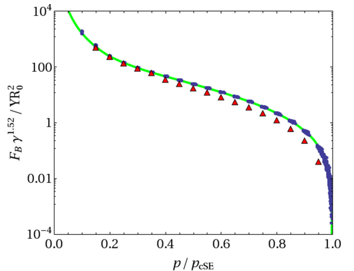
FIG. 16. Collapse of the energy barrier obtained by applying an additional z constraint and for increasing \Delta R^2 (dots), numerical approximation of these values (line), and the slightly lower energy barrier (red triangles) obtained by reducing \Delta R^2 starting from a concave, indented shape.
