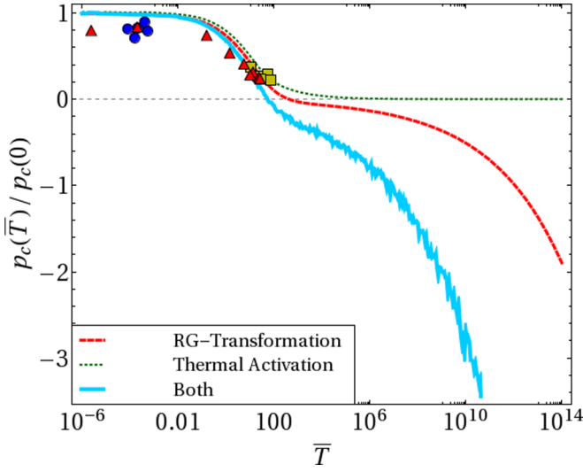
FIG. 11. Critical buckling pressure p_c(T) as a function of the dimensionless temperature \bar{T} = k_B T \sqrt{\gamma}/\kappa according to the buckling criterion D_R(q^*) = 0 which includes renormalization effects only (dark red dashed line, see also red solid line in Fig. 3), p_c(T) according to the criterion F_B[p_c(T)] = k_B T or Eq. (37) for thermal activation over the buckling energy barrier (green dotted line, for \nu = 1/3 ), and p_c(T) according to the generalized criterion F_{B,R}(q^*)/k_B T = 1 or Eq. (38) which combines renormalization effects and thermal activation (light blue solid line, for \nu = 1/3 ). Inclusion of thermal activation leads to a decrease of the critical buckling pressure for \bar{T} > 1 . As in Fig. 3, data points show numerical results from Ref. [43].
