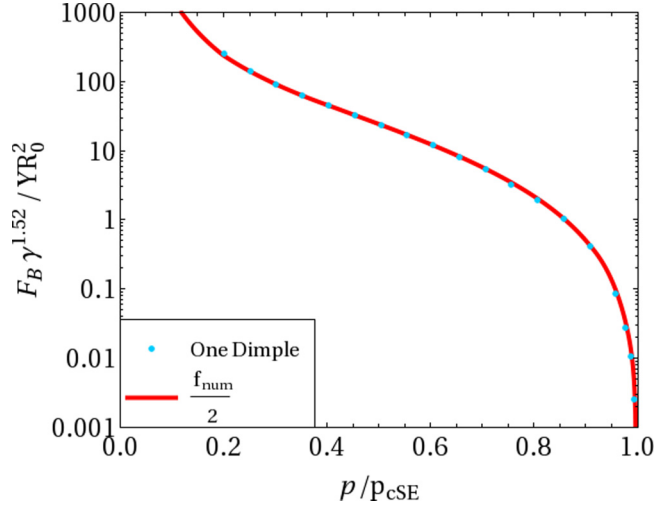
FIG. 18. Energy barrier as a function of pressure for one dimple (light blue points) and half of the approximated energy barrier for two dimples (solid dark red line) from numerical simulations; see Eq. (B1) (for \gamma = 10^4 and \nu = 0.3 ).
