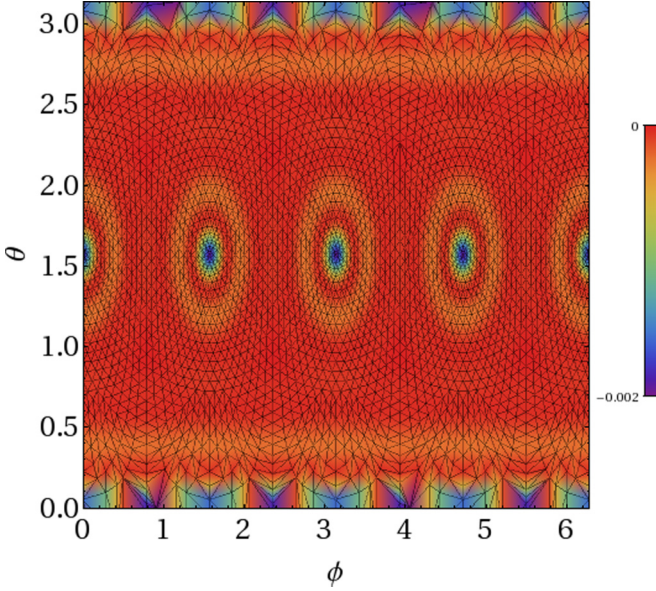
FIG. 14. R(\phi, \theta) - \bar{R} , in spherical coordinates, where R(\phi, \theta) is the distance to the center of the sphere, and \bar{R} is its average, for an additional z constraint and directly before the first jump in Fig. 13(b) for p/p_c = 0.85 . The variance \Delta R^2 is mostly caused by six fourfold disclinations (four at \theta \sim \pi/2 and one at \theta = 0, \pi ), such that the triangulation determines the formation and location of six dimples instead of a single dimple. As a result, the black line in Fig. 13(b) does not envelope the colored lines in Fig. 13(b) for small \Delta R^2 .
