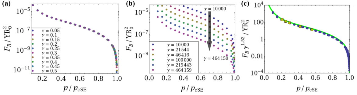
FIG. 9. Energy barrier as a function of the pressure for (a) several values of \nu at \gamma = 10^5 and (b) several values of \gamma (see arrow) at \nu = 0.3 . (c) Collapse of the energy barrier for different values of \gamma (dots). The numerical approximation f_{p,\text{num}}(p/p_{c,\text{SE}}) for the scaling function from Eq. (B3) is shown as green line. For small pressures, the energy barrier scales as p^{-2.8} , which is close to the p^{-3} law from the Pogorelov approximation (29). In the collapse, we also inserted the experimental data from Ref. [38] (yellow squares), which show excellent agreement with our numerical results.
