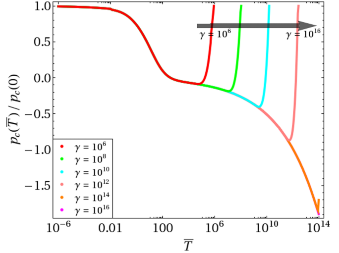
FIG. 4. Nonuniversality of the critical buckling pressure p_c(\bar{T}) for different Föppl–von Kármán numbers \gamma (see arrow). For large values of \gamma , the nonuniversality is shifted to large dimensionless temperatures \bar{T} .
