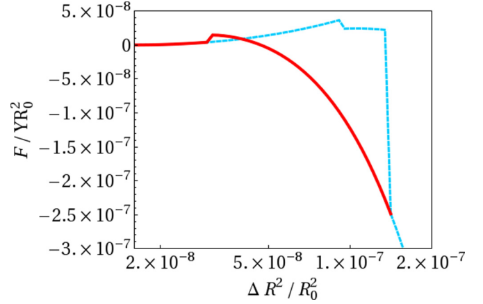
FIG. 15. Shape hysteresis and minimal enthalpy as a function of \Delta R^2 . The light blue dashed line shows the minimum enthalpy for increasing \Delta R^2 , starting from the spherical shape, and the dark red solid line shows the minimum enthalpy found for decreasing \Delta R^2 , starting with a concavely indented shape. The reverse red path with concavely indented shapes exhibits a lower global enthalpy maximum than the blue forward path and becomes unstable for small \Delta R^2 , where shapes become convex again.
