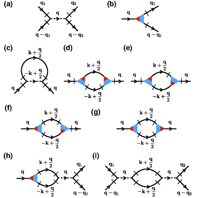
FIG. 17. Feynman diagrams approximating (A4) to one-loop order. The legs correspond to \tilde{f}(\mathbf{q}) , legs with slashes correspond to derivatives of \tilde{f}(\mathbf{q}) , i.e., q_i \tilde{f}(\mathbf{q}) . Connected legs represent the propagator G(\mathbf{q}) . The blue parts of the three-point vertices connect to the derivatives, whereas the red parts connect to legs without slashes. Three-point vertices carry the factor Y/R_0 , and four-point vertices carry the factor Y . Image taken from Ref. [44].
