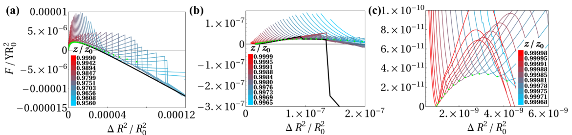
FIG. 13. Minimal enthalpy as a function of \Delta R^2 obtained by the two outlined approaches, i.e., for constrained z (colored lines) or unconstrained z (thick black lines) for \gamma = 100\,000 , \nu = 0.3 , and p/p_c = 0.3 (a), p/p_c = 0.85 (b), and p/p_{c,SE} \approx 0.998 (c). Lines of different colors correspond to different values of z . Green dots show local energy minima for different values of z/z_0 with z_0 being the initial value of z , before deformation. (a) The colored lines of the z -constrained enthalpy touch the black line for unconstrained z (i.e., the black line is the envelope of the colored lines) indicating that the optimal buckled configuration consists of a single dimple. (b) Jumps in the colored and black curves are caused by large inward moves of a vertex in the center of the indentation when the indentation switches from its initial concave into its final convex shape. These jumps occur behind the initial energy barrier. The black line shows small deviations from the envelope of the colored lines for small \Delta R^2 because the location of a single dimple is determined by the z constraint (colored lines), whereas the initial formation and location of dimples is strongly influenced by the presence of disclinations for unconstrained z (black line). (c) Close to the critical pressure, the influence of the disclinations is even stronger (therefore, data for unconstrained z is not shown).
