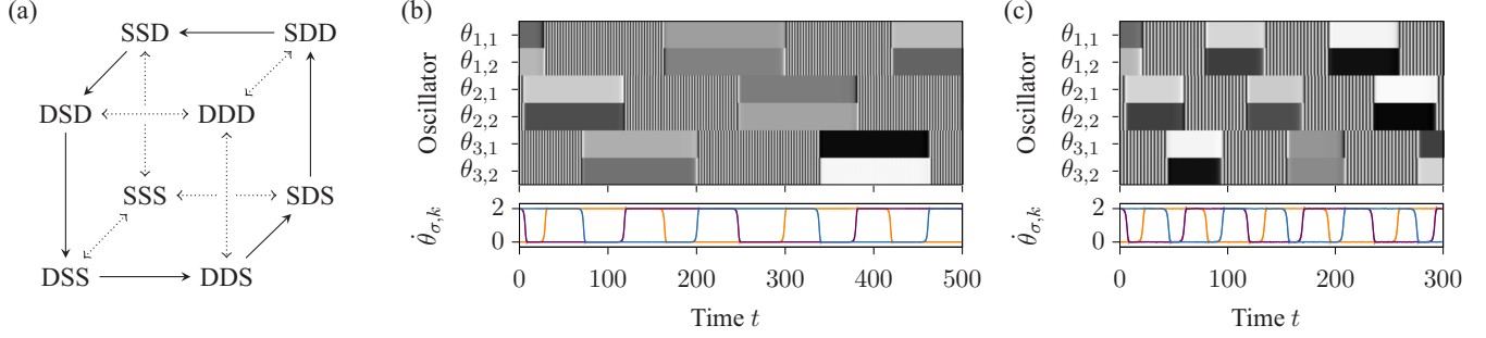
FIG. 1. Heteroclinic networks appear in networks of M = 3 populations of N = 2 oscillators (5) with coupling function (2) and \alpha = \frac{\pi}{2} , r = -0.1 , K = 0.1 . Panel (a) shows the heteroclinic cycle between saddle weak chimeras (the solid lines); stability is indicated by arrows. Panel (b) shows switching of localized frequency synchrony close to the heteroclinic cycle for \delta = 0 in the presence of noise \eta = 10^{-7} : The oscillators' phases (shading; black if \theta_{\sigma,k} = \pi , white if \theta_{\sigma,k} = 0 ) and frequencies (colors; shading indicates a population's frequency range [\min_k \dot{\theta}_{\sigma,k}, \max_k \dot{\theta}_{\sigma,k}] , a line its average (\dot{\theta}_{\sigma,k})_k ) are plotted over time. The frequencies of different populations synchronize and desynchronize sequentially. Panel (c) shows irregular switching dynamics without noise \eta = 0 when the symmetries are broken, \delta = 0.01 .
