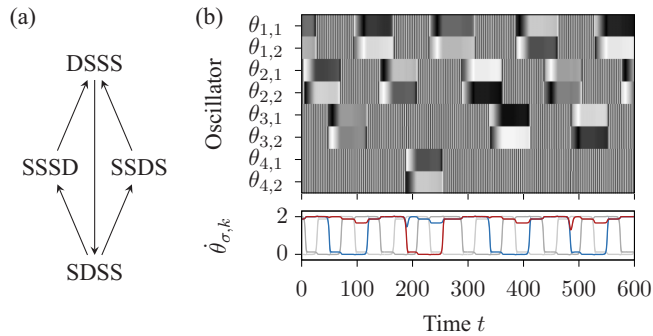
FIG. 3. The network of M = 4 populations of N = 2 oscillators with dynamics (13) shows noise induced random switching from SDSS to either SSDS or SSSD. This relates to a Kirk-Silber type network sketched in panel (a). Panel (b) depicts evolution of phases and frequencies (populations 3 and 4 are highlighted in color) for coupling (2) with r = -0.1 , \alpha = \frac{\pi}{2} , K = 0.35 , and \eta = 10^{-4} .
