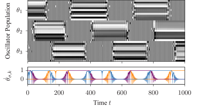
FIG. 2. Switching between localized frequency synchrony is observed in networks of M = 3 populations of N = 11 oscillators with dynamics (5) and vector field (11). As in Fig. 1 the evolution of phases and order parameters the oscillators populations synchronize in frequency sequentially. Coupling for K = 0.2 is given by (6) with a = 22 , r = -0.001 , \alpha = \frac{\pi}{2} , symmetry breaking \delta = 0.001 and no noise \eta = 0 .
