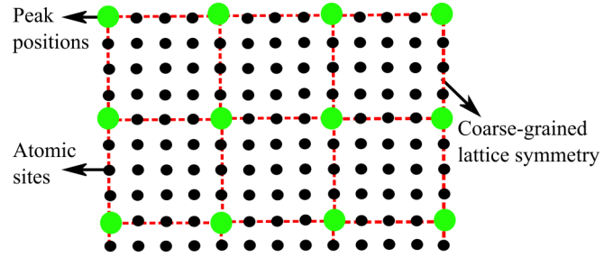
FIG. 5. Schematic illustration of the atomic sites, peak positions, and coarse-grained lattice symmetry in a square phase system. The small-black dots represent atomic sites of the unit cell. The big-green dots schematically indicate peak positions in a CH-PFC simulation. The dashed-red lines connecting the peaks highlight an example of a coarse-grained lattice symmetry of the underlying unit cells. Note, in this figure the coarse-grained symmetry is four times the unit cell size.
