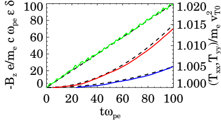
FIG. 2. Evolution of the averaged B_z due to the perpendicular density and temperature gradients (top, green), and anisotropic temperatures T_{xx} (bottom, blue) and T_{yy} (middle, red), vs time along with the predicted curves at y = 0 from Eqs. (19) and (14) (black dashed lines).
