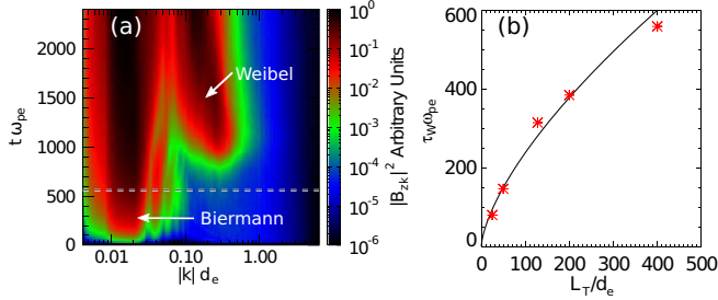
FIG. 1. (a) Magnetic energy spectra of B_z (with respect to |k| = \sqrt{k_x^2 + k_y^2} ) vs time from the simulation with system size L_T/d_e = 400 ( L_T/\lambda_D = 2000 ) reported in Ref. [9]. The time when the Weibel instability begins to grow exponentially is identified with a dashed line. This estimate of the onset time \tau_W is plotted vs system size (b) along with the predicted curve where Eq. (16) is satisfied, indicating where the Weibel growth rate exceeds that of the anisotropy predicted in Eq. (15).
