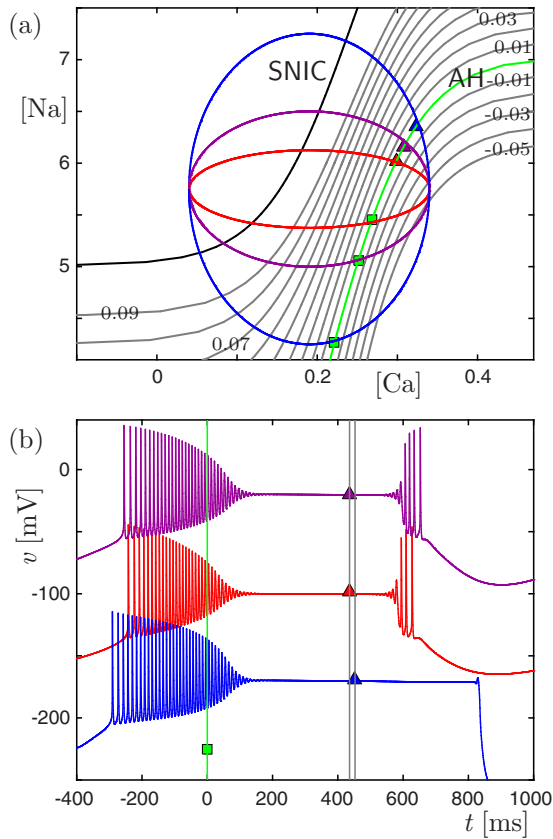
FIG. 7. Contraction to and expansion away from the depolarization block state depends on the real part \text{Re}(\lambda) of the eigenvalues of the associated equilibria in the fast subsystem that are encountered along the imposed path. (a) Shows SNIC and AH in the ([Ca], [Na]) plane along with contours (gray) of \text{Re}(\lambda) . Overlaid are paths with [Ca]_c = 0.19 , [Na]_c = 5.75 , [Ca]_0 = 0.04 , and \varepsilon = 0.004 , and varying d = 0.1 (blue, outermost ellipse), d = 0.2 (purple, central ellipse), and d = 0.4 (red, innermost ellipse). The corresponding time courses of v are shown in (b) with time shifted so that the first crossing occurs at t = 0 (green square on the vertical line at t = 0 ), and voltage shifted down by 200 and 100 mV for the time courses with d = 0.1 (blue, lowermost trace) and d = 0.4 (red, middle trace), respectively; the second crossing of AH is marked with triangles.
