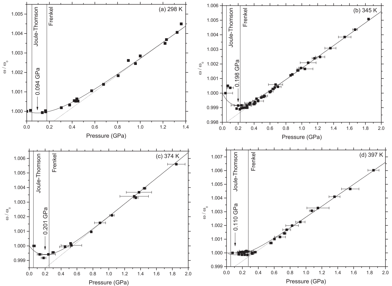
FIG. 3. Plot of reduced frequency of \text{CH}_4 Raman-active vibration as a function of pressure at (a) 298 K, (b) 345 K, (c) 374 K, and (d) 397 K. Solid lines following the data are fits performed using Eq. (6) and arrows signify the minimum of this fit. Dotted lines are linear fits to data collected above 0.6 GPa [Eq. (5)]. Vertical solid lines are expected positions of the Joule-Thomson line and Frenkel line.
