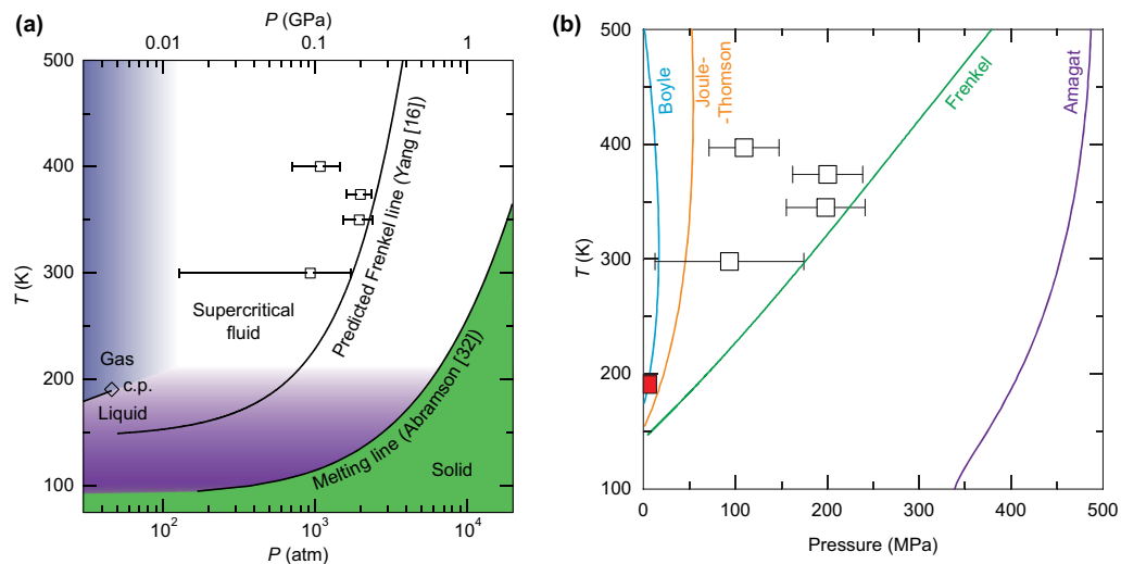
FIG. 5. Phase diagram of CH 4 . (a) The theoretically predicted Frenkel line in CH 4 [16] is marked along with the experimentally observed melting curve [32]. The data points are the crossovers we observe experimentally and attribute to the Frenkel line. (b) The position of the theoretically predicted Frenkel line compared to the Boyle curve, Joule-Thomson curve, and Amagat curve. Open squares are our Frenkel line data points and the red closed square is the critical point (c.p.).
