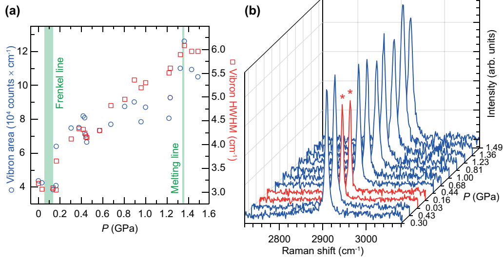
FIG. 4. (a) Plot of Raman peak area (integrated intensity, blue circles) and HWHM (red squares) as a function of pressure at 298 K, showing discontinuous decrease in both area and HWHM when the gaslike side of the Frenkel line is reached. The green shaded region is the area in which the minimum in vibration frequency [fitted using Eq. (6)] lies, which we associate with the Frenkel line and the green line marks the experimentally measured melting line [32]. (b) Waterfall plot of spectra collected at 298 K in order collected, demonstrating the reversible nature of the crossover. Red spectra (marked with asterisks) are those on the gaslike side of the Frenkel line.
