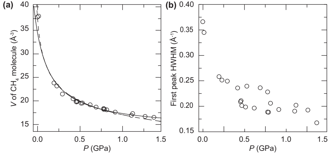
FIG. 2. (a) Equation of state (EOS) of fluid CH 4 at 298 K. Circles: experimental data. Solid line: Fit of ideal gas EOS modified with van der Waals correction [Eq. (4)]. Dotted line: Fit of Murnaghan EOS [Eq. (1)]. (b) HWHM of first peak in S(q) plotted as a function of pressure at 298 K.
