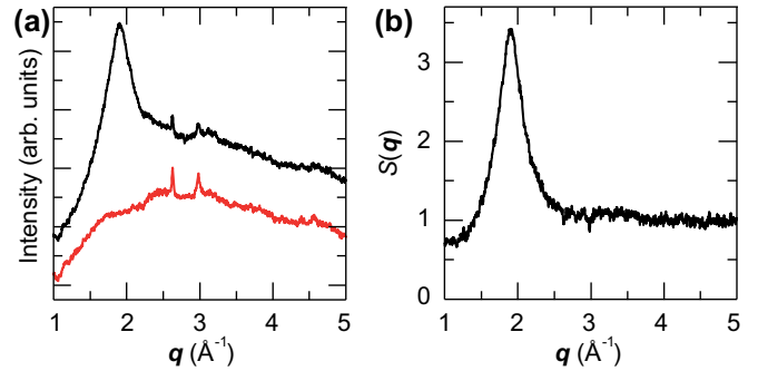
FIG. 1. Background correction of integrated diffraction patterns. (a) Diffraction pattern of fluid CH 4 at 0.69 GPa (black, upper) and background from empty DAC (red, lower). (b) Static structure factor S(q) of CH 4 at 0.69 GPa obtained by subtracting background and normalizing in the high- q limit.
