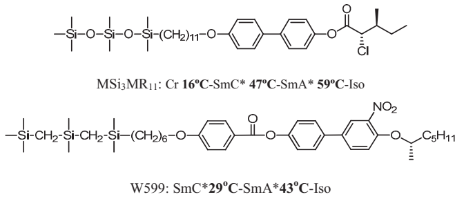
FIG. 2. The molecular structures of MSi 3 MR 11 (top) and W599 (bottom) with their corresponding phase transition temperatures (MSi 3 MR 11 : Cr16°C, Sm-C* 47°C, Sm-A* 59°C, Iso; W599: Sm-C* 29°C, Sm-A* 43°C, Iso) obtained by polarized optical microscopy at a cooling rate of 1°C/min are specified.
