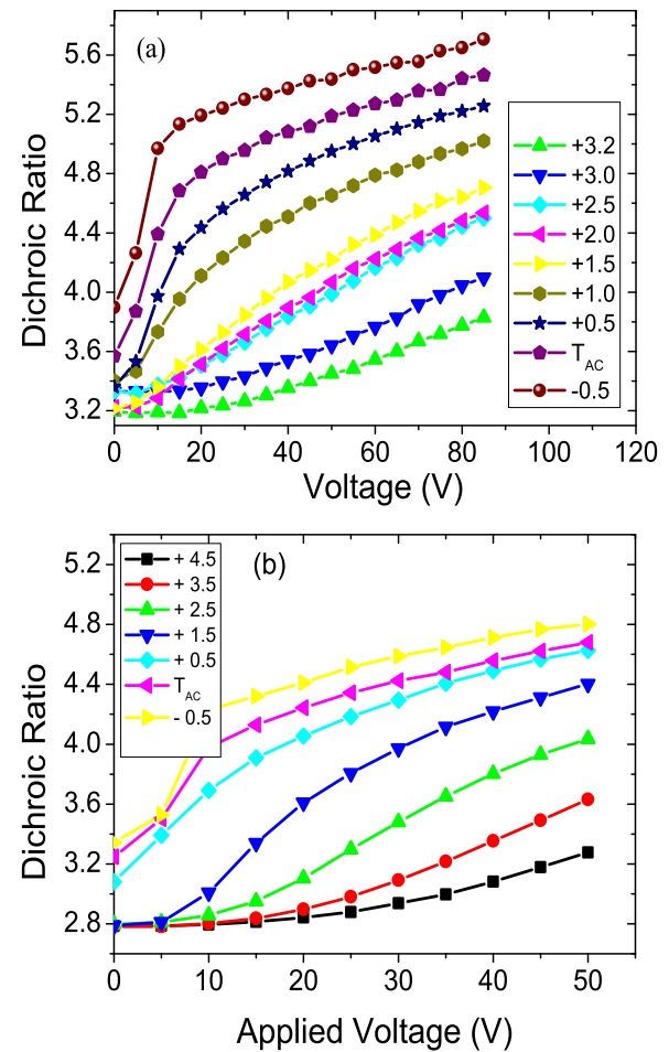
FIG. 6. Dichroic ratio ( R = A_{\parallel}/A_{\perp} ) versus the applied dc voltage for the phenyl band 1608 cm -1 at different temperatures for a homogeneous planar-aligned cell of 5 μm thickness for (a) MSi 3 MR 11 and (b) W599. (+) Temperatures in the inset denote above T_{AC} transition temperature in the Sm-A* phase and (-) denote below it in the Sm-C* phase.
