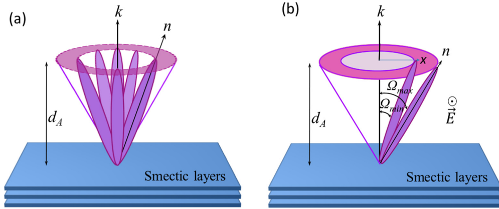
FIG. 1. Schematic illustration of the de Vries diffuse-cone model in the Sm- A^* phase. Here \vec{k} is the layer normal, \vec{n} is the direction of long molecular axis, d_A is the layer spacing, while \Omega_{\max} is the maximum tilt angle at a large field, and \Omega_{\min} is evaluated from the experimental data on birefringence at zero field. The azimuthal angle is distributed on the cone at zero field. The apparent tilt angle is thus zero. For higher fields, the azimuthal angle condenses to an almost single value leading to the maximum apparent angle, \Omega_{\max} . The apparent tilt angle \Omega_0 varies with the field.
