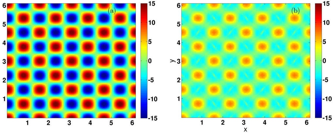
FIG. 1. Pseudocolor plots of the Okubo-Weiss parameter \Delta for (a) \Omega = 1 and Wi = 0 and (b) \Omega = 20 and Wi = 1 ; these show vortex-crystal states. Given our color bar in (a), vortical regions are red and strain-dominated regions are dark blue.
