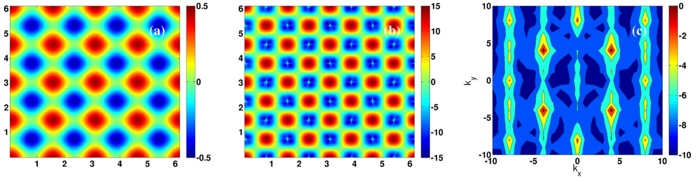
FIG. 4. Pseudocolor plots for \Omega = 1 and Wi = 1 : (a) the stream function \psi and (b) the Okubo-Weiss parameter \Lambda ; (c) a filled contour plot of the E_\Lambda , reciprocal-space spectrum; this shows peaks at the forcing wave vectors.
