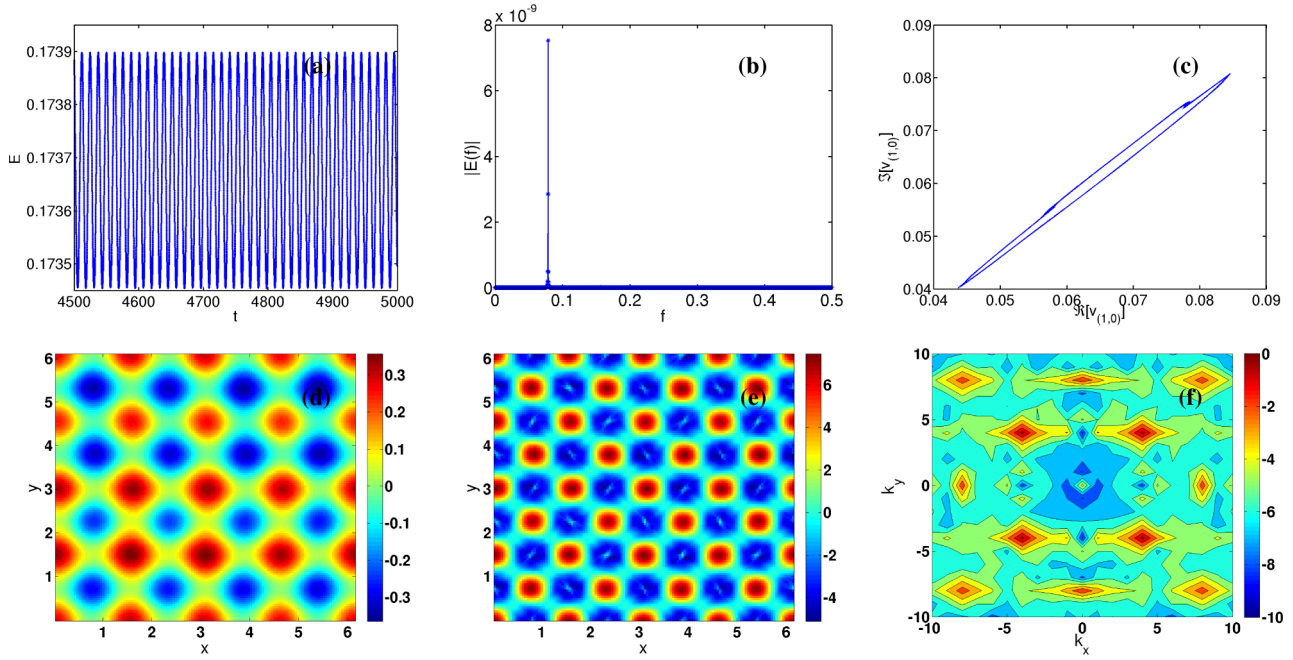
FIG. 10. Plots for \Omega = 22 and Wi = 0.7 : (a) the time evolution of the energy E(t) , (b) the power spectrum |E(f)| versus the frequency f , and (c) the Poincaré-type section in the plane (\Re[\hat{v}(1,0)], \Im[\hat{v}(1,0)]) . Pseudocolor plots of (d) the stream function \psi and (e) the Okubo-Weiss parameter \Lambda ; and (f) a filled contour plot of the reciprocal-space spectrum E_\Lambda .
