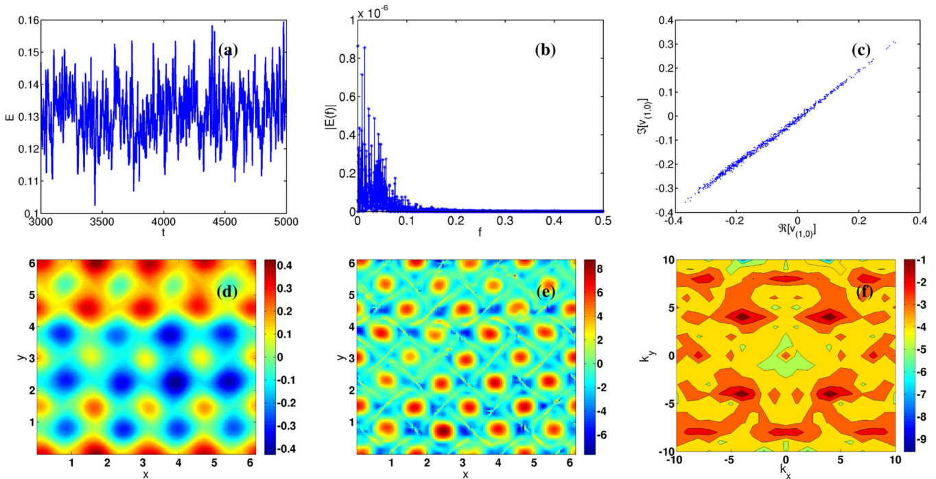
FIG. 11. Plots for \Omega = 22 and Wi = 20 : (a) the time evolution of the energy E(t) , (b) the power spectrum |E(f)| versus the frequency f , and (c) the Poincaré-type section in the plane (\Re[\hat{v}(1,0)], \Im[\hat{v}(1,0)]) . Pseudocolor plots of (d) the stream function \psi and (e) the Okubo-Weiss parameter \Lambda ; and (f) a filled contour plot of the reciprocal-space spectrum E_\Lambda .
