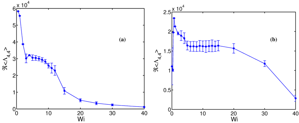
FIG. 12. Plots of \langle\hat{\Lambda}_{k=(4,4)}\rangle versus Wi for (a) \Omega = 1 and for (b) \Omega = 22 ; in (b) \langle\hat{\Lambda}_{4,4}\rangle first increases with Wi , goes through a maxima, which corresponds to an OPXA state, and then decreases after that.
