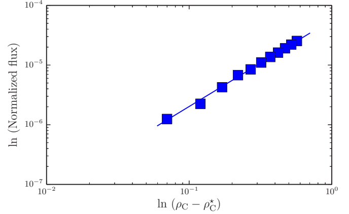
FIG. 5. Time-averaged tracer flux as a function of (\rho_C - \rho_C^*) at a temperature corresponding to k_B T_s / J_{\text{int}} = 0.1 . Squares represent simulation data, and the solid line is a linear fit to the simulated data with scaling exponent \alpha \approx 4/3 .
