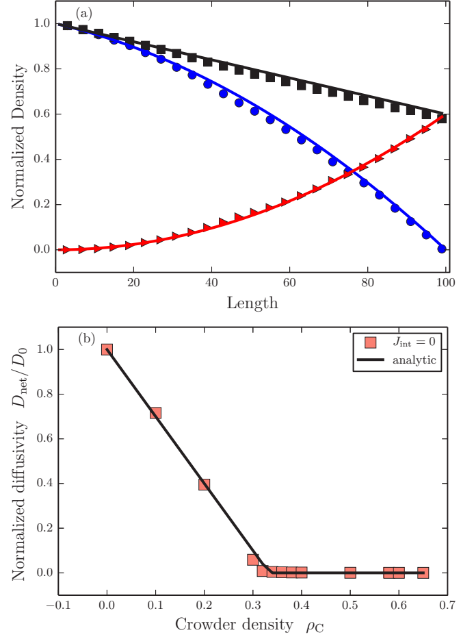
FIG. 4. (a) Density profiles of crowders (red triangles), tracers (blue circles), and their sum (black squares) for the high-temperature limit at a value of crowder density \rho_C = 0.2 . Solid lines represent analytic solutions given by Eqs. (4)–(5) and their sum. (b) Normalized diffusivity as a function of crowder density for the scenario where the exchange coefficient of interaction, J_{\text{int}} = 0 . Squares represent simulated data points, and the solid line represents analytic solution for diffusivity.
