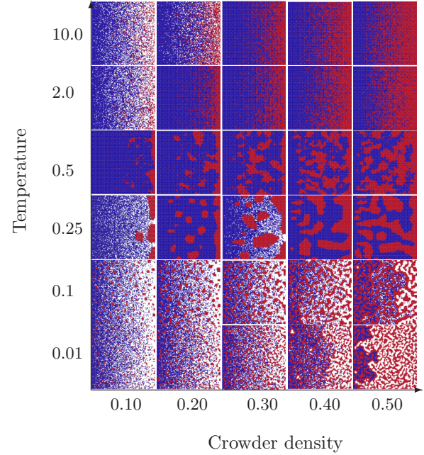
FIG. 2. Final configurations for varying values of crowder density and temperature. The x axis represents crowder density ( \rho_C ), and the y axis represents scaled temperature ( k_B T_s / J_{\text{int}} ). Tracers are shown in blue and crowders are shown in red.
