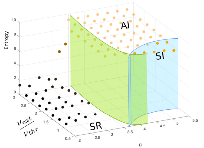
FIG. 4. Computation of the entropy (circles) of the network in the Brunel's model [27] for distinct values of the input intensity v_{\text{ext}} and inhibition ratio g . The color code indicates the entropy amplitude. Parameters as in the original model [[27], Fig. 2(b)]. The blue surface represents the boundary between SI and AI regimes, and the green surface separates SR regimes from SI regimes. We observe a clear transition from low entropy (SR) to high entropy (SI+AI).
