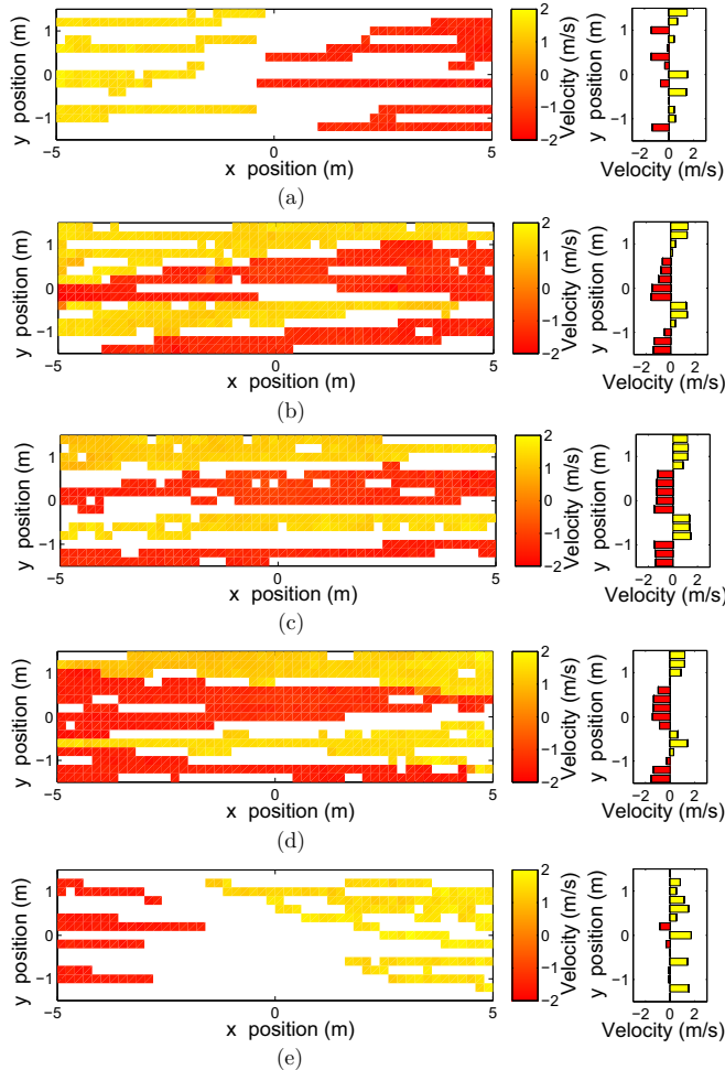
FIG. 14. 2D plot of the average x velocity in different locations for each phase: (a) unidirectional free flow, (b) lane formation, (c) full bidirectional flow, (d) lane dissolution, and (e) unidirectional free flow. The bar graph on the right side gives the average velocity across the different rows. Grid size is 0.2 \text{ m} \times 0.2 \text{ m} and white spots indicate unavailable data. Major flow has a yellow (light gray) gradation and minor flow is represented with red (dark gray) gradation.
