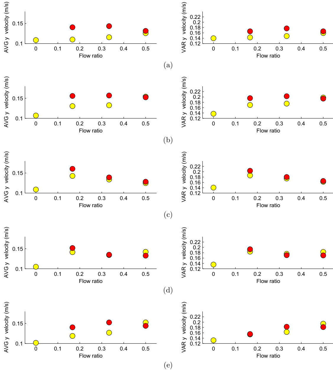
FIG. 11. y velocity for the different phases: (a) unidirectional free flow, (b) lane formation, (c) full bidirectional flow, (d) lane dissolution, and (e) unidirectional free flow. Yellow (light gray) dots refer to the major flow and red (dark gray) dots to the minor flow. AVG stands for average, VAR for variance.
