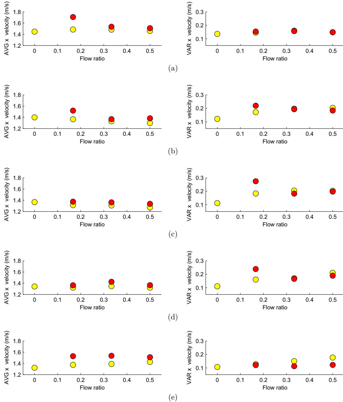
FIG. 10. x velocity for the different phases: (a) unidirectional free flow, (b) lane formation, (c) full bidirectional flow, (d) lane dissolution, and (e) unidirectional free flow. Yellow (light gray) dots refer to the major flow and red (dark gray) dots to the minor flow. AVG stands for average, VAR for variance.
