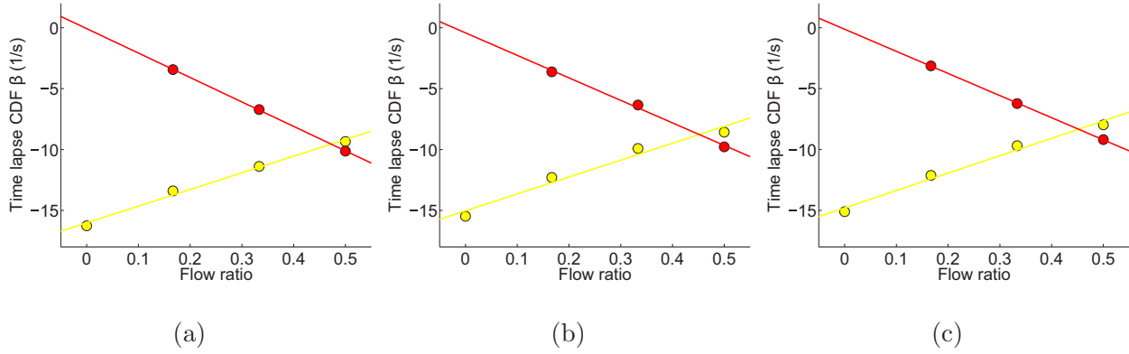
FIG. 13. Time lapse distribution width in function of the flow ratio for different positions: (a) entrance, (b) x position = 0 m, and (c) exit. Yellow (light gray) is used for the major flow and red (dark gray) for the minor flow.
