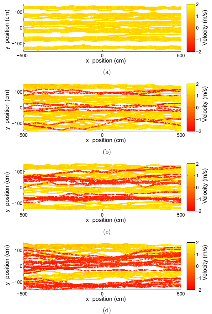
FIG. 6. Trajectories recorded in a selected run for each of the different configurations: (a) 6/0 configuration, (b) 5/1 configuration, (c) 4/2 configuration, and (d) 3/3 configuration. Path color (gradation) indicates the x component of the velocity. It is important to remind that each configuration was repeated four times, so the trajectories represented here are only for reference. Major flow [positive velocity, yellow (light gray)] goes from left to right, minor flow [negative, red (dark gray)] from right to left.
