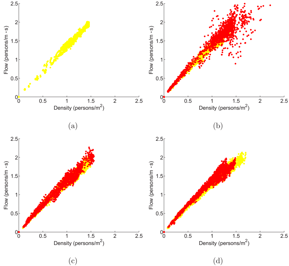
FIG. 8. Fundamental diagrams for each configuration: (a) 6/0 configuration, (b) 5/1 configuration, (c) 4/2 configuration, and (d) 3/3 configuration. Diagrams were obtained by combining the results of the four runs in each case. Dots' color indicates the group considered: yellow (light gray) stands for major flow and red (dark gray) for minor flow.
