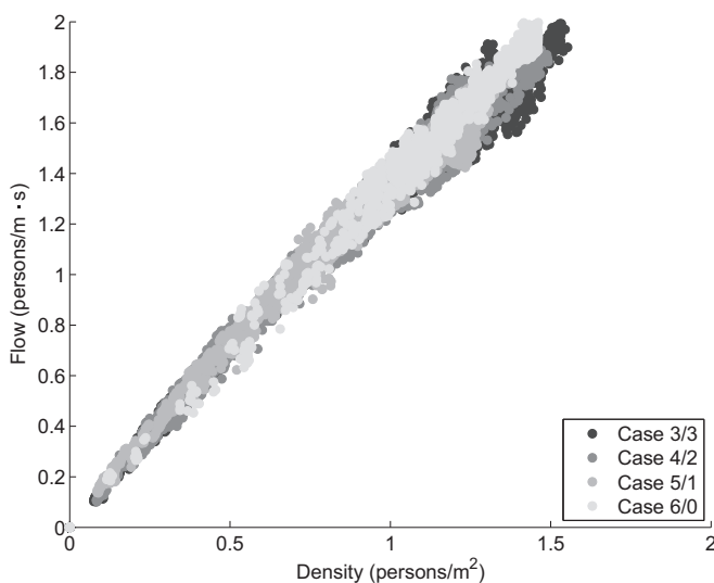
FIG. 7. Comparison of the different fundamental diagrams; no differentiation is made between minor and major flows. Uncongested, comparable flow was observed in all the cases. Without further investigations, differences between the different configurations cannot be easily identified.
