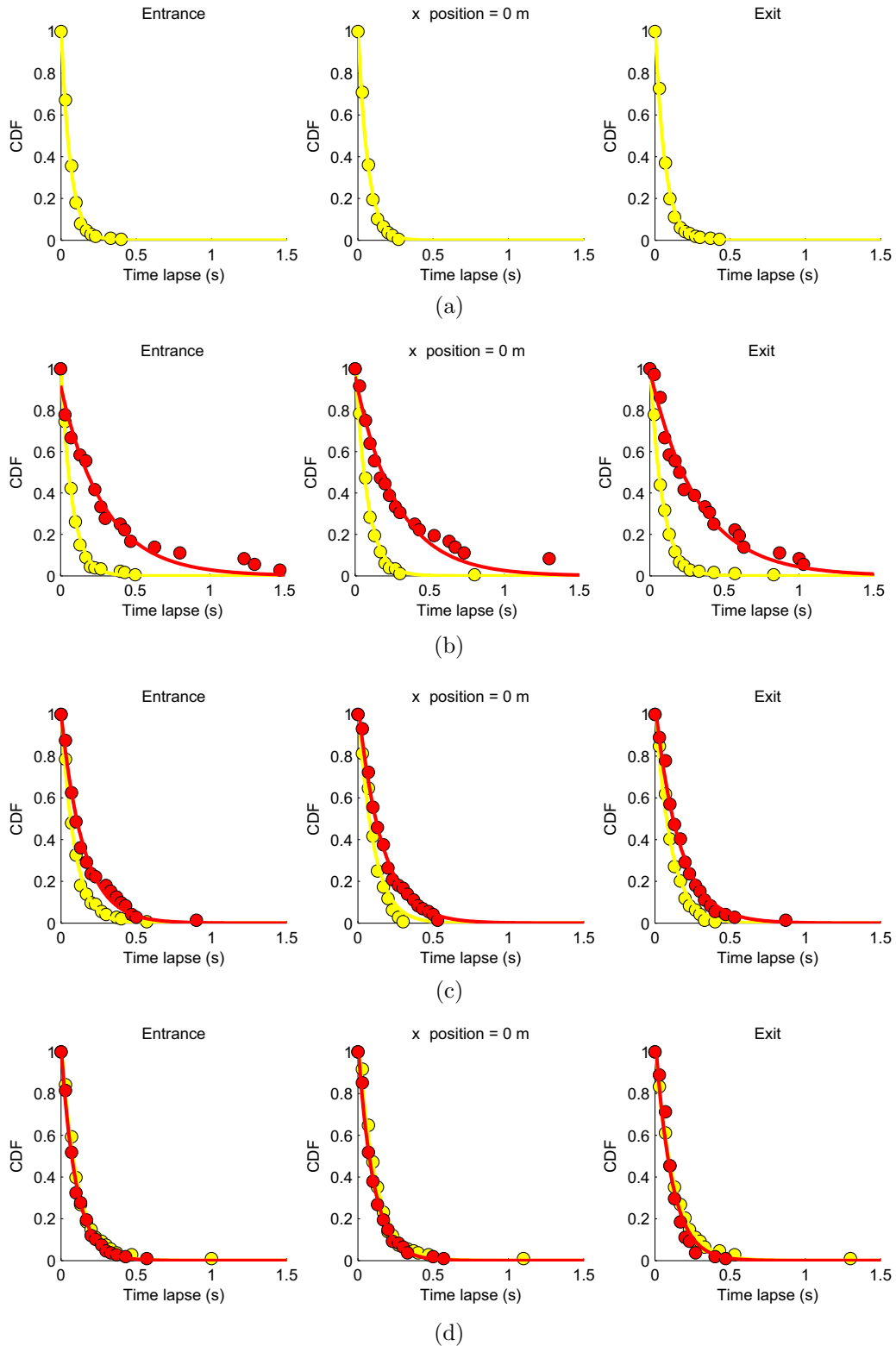
FIG. 12. Time lapse distribution for the different configurations: (a) 6/0 configuration, (b) 5/1 configuration, (c) 4/2 configuration, and (d) 3/3 configuration. Each distribution fits well with the exponential function. Yellow (light gray) is used for the major flow and red (dark gray) for the minor flow. CDF stands for cumulative density function.
