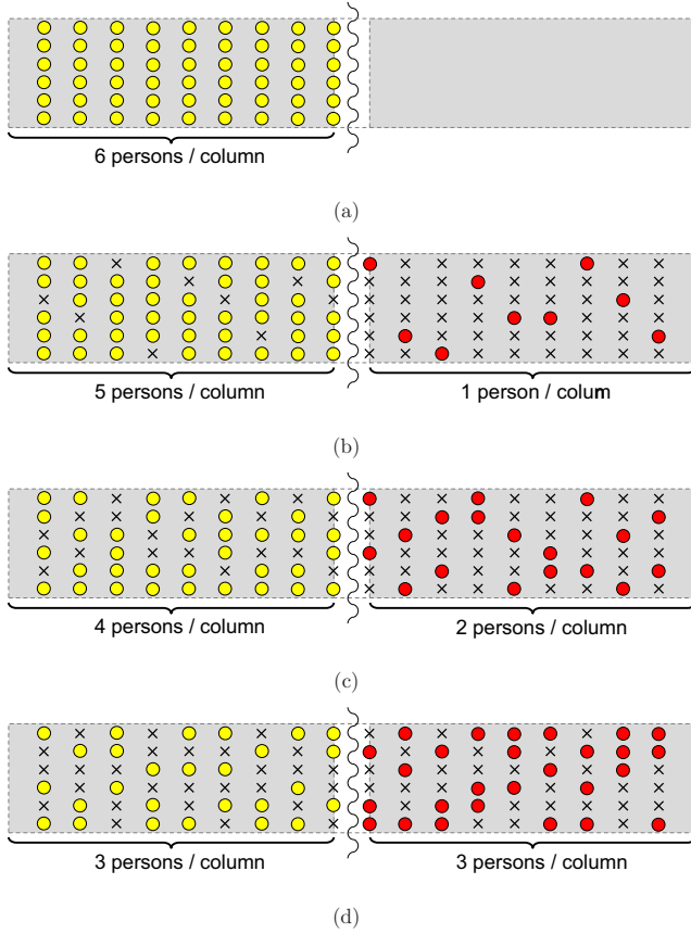
FIG. 4. Starting positions during the different configurations: (a) unidirectional 6/0 configuration, (b) bidirectional 5/1 configuration, (c) bidirectional 4/2 configuration, and (d) bidirectional 3/3 configuration. Positions given in the diagram do not necessarily coincide with the actual positions taken by participants during the experiment and are only for illustrative purpose. Crosses represent empty positions, while circles stand for occupied positions. Yellow (light gray) circles symbolize participants of the major flow and red (dark gray) circles are representative of the minor flow.
