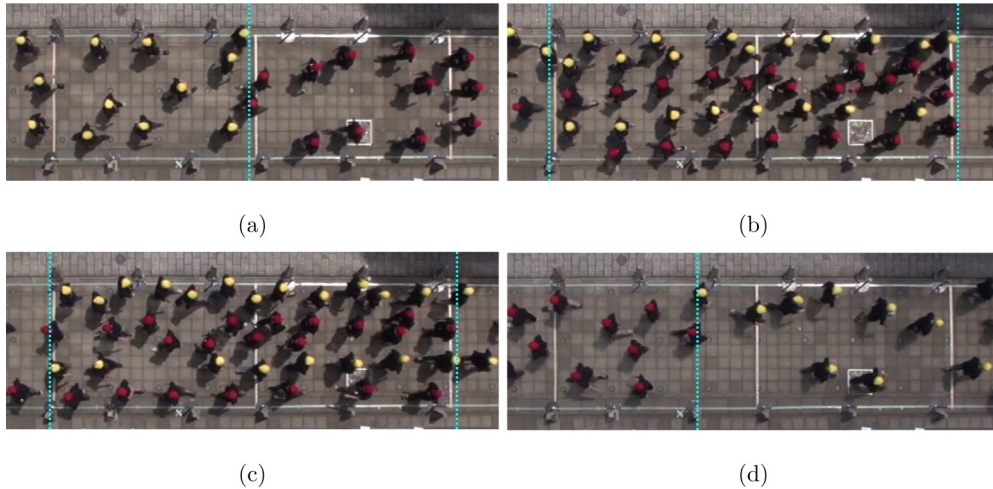
FIG. 9. Relevant moments during the process of lane formation and dissolution in a balanced bidirectional flow: (a) time t_1 (beginning of lane formation), (b) time t_2 (beginning of full bidirectional flow), (c) time t_3 (beginning of lane dissolution), and (d) time t_4 (end of bidirectional flow). Major flow pedestrians wear yellow (light gray) caps, minor flow participants use red (dark gray) caps.
