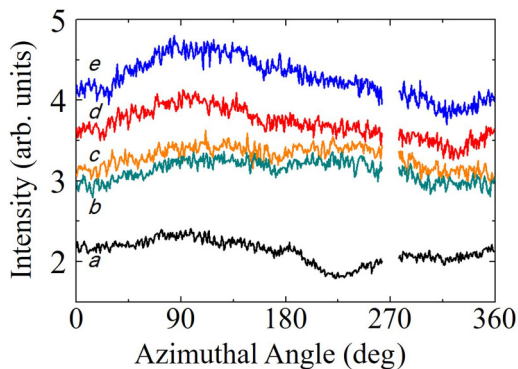
FIG. 5. Azimuthal intensity profiles of the WA peaks shown in the fits of Fig. 2: peak p_1 of BCN \mathbf{1} at 155 °C (curve a), peaks p_1 (curve c) and p_2 (curve d) of BCN \mathbf{2} at 100 °C, and peaks p_1 (curve b) and p_2 (curve e) of BCN \mathbf{2} at 30 °C. The gap at 270° is due to the shadow of the beamstop.
