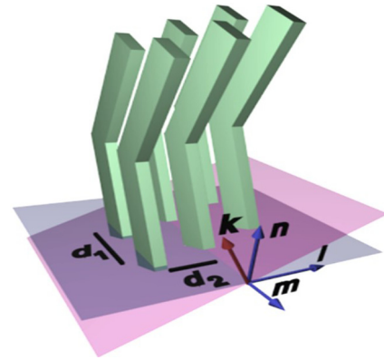
FIG. 3. Schematic drawing of the molecular ordering within a cybotactic cluster: k indicates the normal to the smectic plane (purple); n , m , and l are the three orthogonal molecular directors; and d_1 and d_2 are the intermolecular distances in the plane normal to n (gray).
