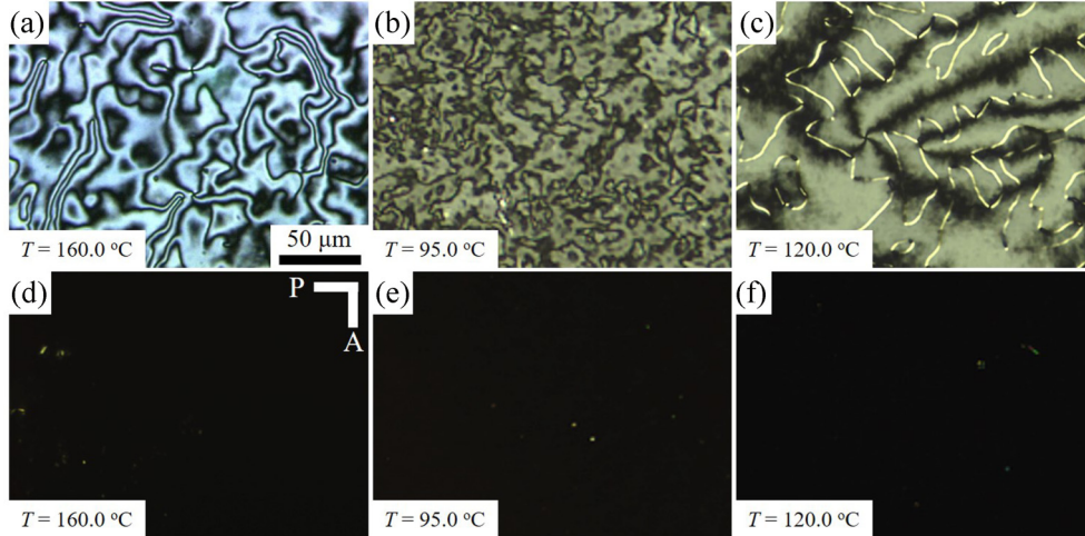
FIG. 6. The POM textures of BCNs 1–3 in (a)–(c) SE5661 and (d)–(f) RM-SE5661 cells of h = 1.3 \mu\text{m} . The left column is with BCN 1 at T = 160.0^\circ\text{C} , the central column is with BCN 2 at T = 95.0^\circ\text{C} , and the right column is with BCN 3 at T = 120.0^\circ\text{C} . Here P and A indicate the polarization of the polarizer and analyzer, respectively.
