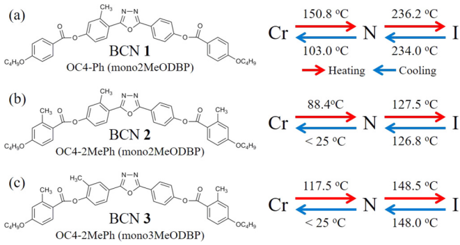
FIG. 1. Chemical structures and phase diagrams of the ODBP bent-core nematic (BCN) liquid crystals (a) OC4-Ph(mono2MeODBP), (b) OC4-2MePh(mono2MeODBP), and (c) OC4-2MePh(mono3MeODBP); Cr, N , and I represent crystal, nematic, and isotropic phases, respectively.
