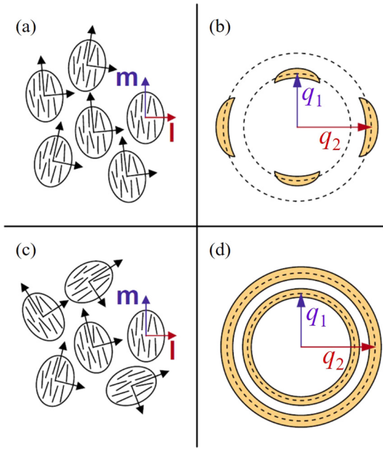
FIG. 4. Orientation of the transverse molecular directors \mathbf{m} and \mathbf{l} in N_b with \mathbf{n} perpendicular to the drawing: transverse directors aligned by (a) an external field or (c) randomly distributed in the plane orthogonal to \mathbf{n} . The ellipses represent micron-sized domains (each one consisting of uniformly aligned nanometer-sized cybotactic clusters) where the orientation of the molecular director is spontaneously uniform. (b) and (d) Corresponding WA diffraction patterns. The latter would be indistinguishable from that of a composite N_u comprised of randomly oriented nanometer-sized biaxial clusters.
