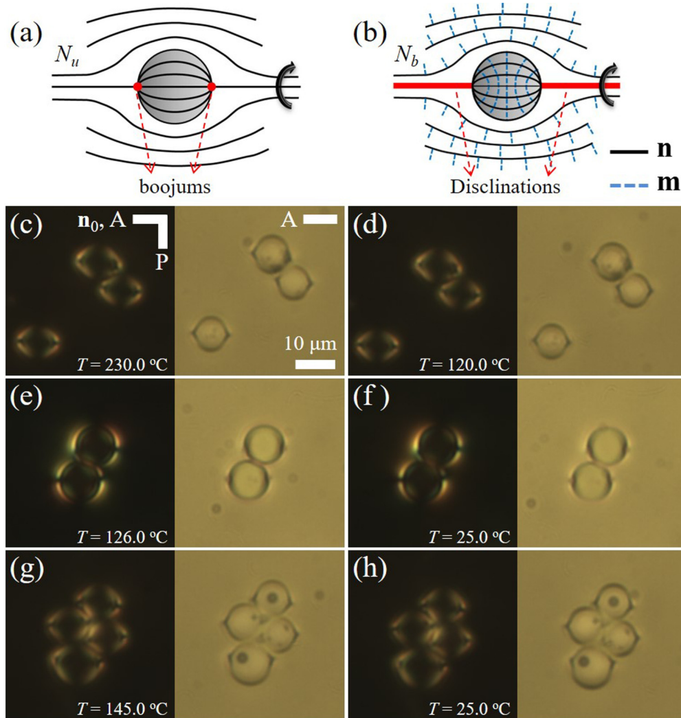
FIG. 8. (a) Scheme of the director configuration around a sphere with tangential alignment placed in a planar N_u cell; note two point-defect boojums at the poles. (b) Hypothetical configuration of the main and secondary directors around a similar sphere placed in an N_b cell. Note two disclination lines, which are formed by the secondary director \mathbf{m} , emerging from the poles. (c)–(h) The POM textures of isolated glass spheres and their clusters in the planar N cells ( h = 20\text{ }\mu\text{m} ) at the temperatures indicated in the figures for (c) and (d) BCN 1, (e) and (f) BCN 2, and (g) and (h) BCN 3. Here P, A, and \mathbf{n}_0 represent the polarization of the polarizer and analyzer and the overall director set by the rubbing direction, respectively.
