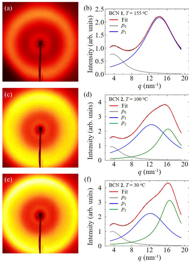
FIG. 2. (a), (c), and (e) The XRD patterns measured with B parallel to the x-ray beam and fits of the corresponding radial intensity profiles (averaged over a \pi azimuthal angle) with (b) two or (d) and (f) three Voigt line shapes: (a) and (b) BCN 1 at 155 °C, (c) and (d) BCN 2 at 100 °C, and (e) and (f) BCN 2 at 30 °C. p_0 is the peripheral scattering of the small-angle region.
