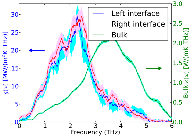
FIG. 2. Spectral interface conductance g(\omega) = |q(\omega)|/\Delta T_s at the left and right liquid-solid interfaces versus frequency. For reference, also the spectrally decomposed bulk conductivity of the solid is shown.
