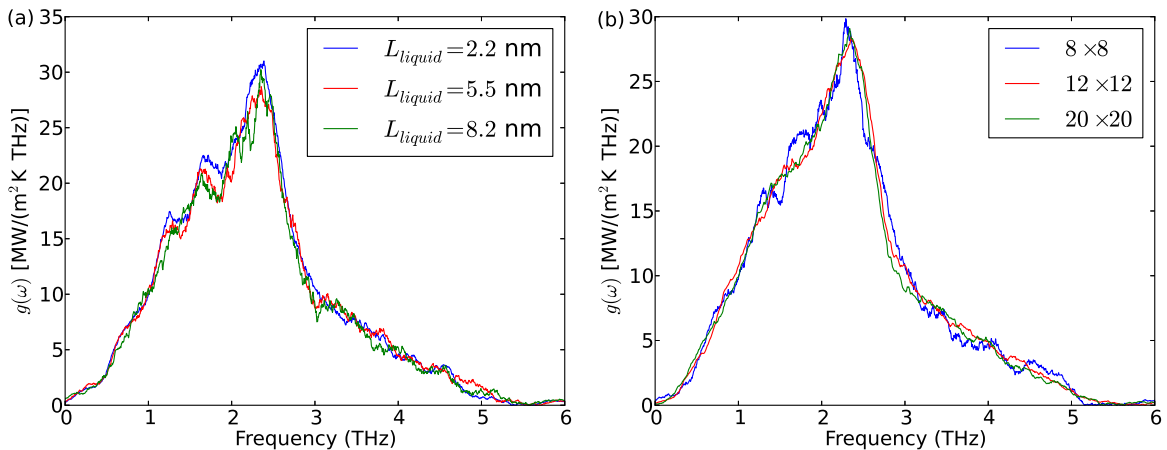
FIG. 5. (a) Spectral conductance g(\omega) at the left interface for various lengths of the liquid at T = 150 K and P = 50 MPa. (b) Spectral conductance for various numbers of unit cells in the cross-section.
