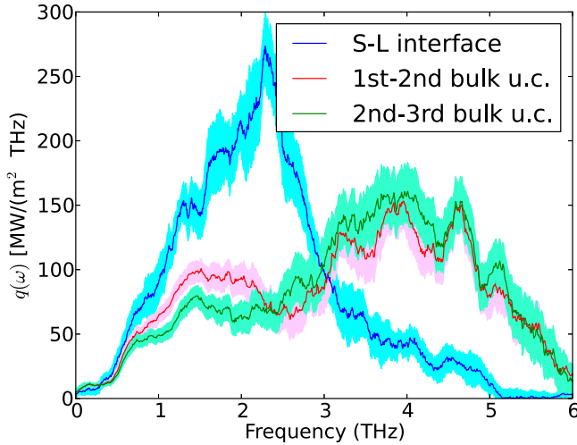
FIG. 6. Spectral heat current q(\omega) inside the solid in the immediate vicinity of the interface, compared to the current at the solid-liquid interface. In the labeling of heat currents in the solid, the first unit cell (u.c.) refers to the two solid monolayers closest to the liquid, second unit cell refers to the third and fourth monolayers away from the interface, etc.
