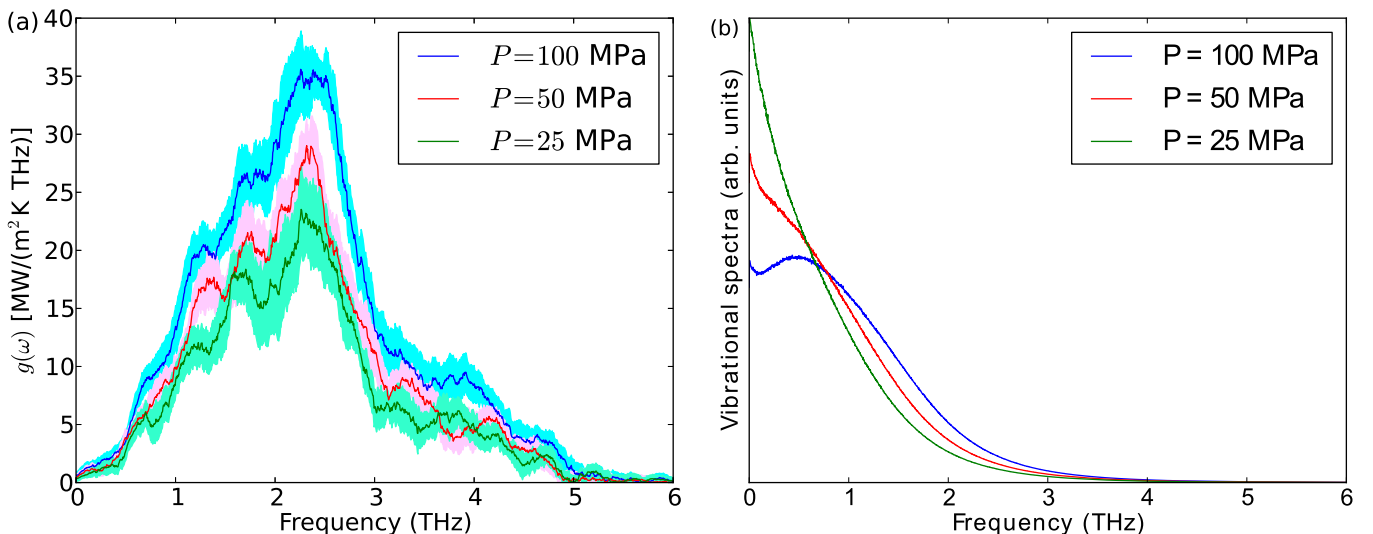
FIG. 7. (a) Spectral conductance g(\omega) at the left liquid-solid interface for different pressures P . (b) Vibrational spectrum in the liquid in the three cases.
