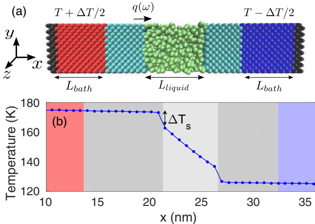
FIG. 1. (a) Schematic illustration of the studied system: Lennard-Jones liquid sandwiched between two Lennard-Jones solids arranged in a face-centered cubic lattice. The spectral heat current q_{1 \rightarrow s}(\omega) is calculated at the solid-liquid interfaces by monitoring the force and velocity trajectories of the atoms located within the potential cutoff distance from the liquid. (b) Typical temperature profile in the nonequilibrium simulation. The spectral conductance is defined as g(\omega) = |q_{1 \rightarrow s}(\omega)|/\Delta T_s , where \Delta T_s is the temperature jump at the surface.
