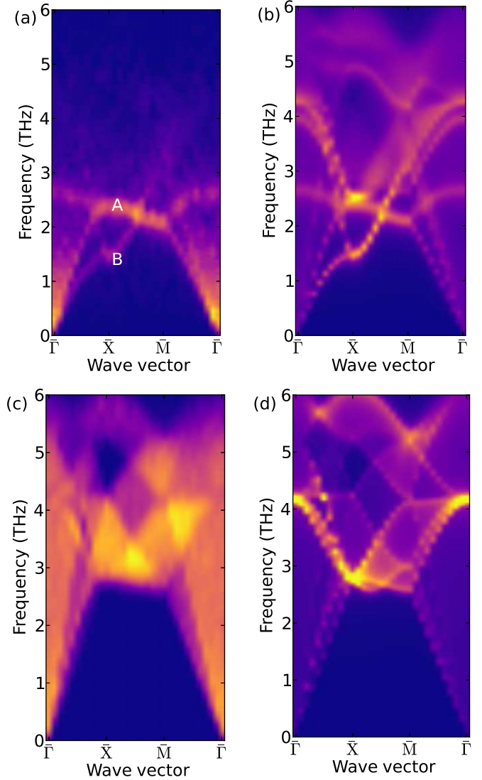
FIG. 3. (a) Wave-vector-decomposed spectral heat flux and (b) interfacial density of states versus wave vector and frequency at the solid-liquid interface (arbitrary units, brighter colors correspond to larger values). (c) Wave-vector-decomposed spectral heat flux and (d) interfacial density of states in the bulk solid. The surface mode labeled as A in (a) and located on the Brillouin zone boundary \bar{X} - \bar{M} contributes strongly to the interfacial conductance at f \approx 2.3 THz. Surface mode labeled B has, on the other hand, smaller effect on energy transfer due to its in-plane polarization. Figures have been calculated for a 20 \times 20 cross-section to improve the wave-vector resolution compared to the 8 \times 8 cross-section used in other calculations.
