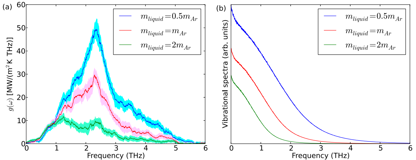
FIG. 8. (a) Spectral heat current q(\omega) at the left liquid-solid interface for different liquid atom masses m_{\text{liquid}} . (b) Vibrational spectrum in the liquid in the three cases. While the calculation of vibrational density of states in the solid would require normalizing S(\omega) by the atomic mass, we have not carried out this normalization for the liquid in order to highlight the effect of liquid mass on diffusion constant [proportional to S(\omega = 0) ].
