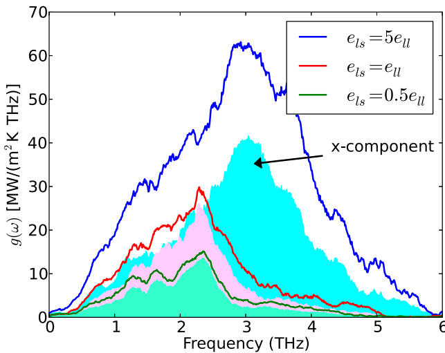
FIG. 4. Spectral conductance at the left liquid-solid interface for various liquid-solid interaction parameters \varepsilon_{ls} . The shaded regions denote the contribution of forces and velocities oriented along the x coordinate (normal to the liquid-solid surface) to the total conductance [Eq. (8)].
