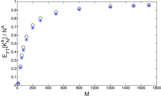
FIG. 6. \mathbb{E}_{\text{FT}}\{K_N^a\}/N^a as a function of M , for N = 11 , a = 6.2 (black circles) and N = 25 , a = 3.2 (blue stars). The convergence to the theoretical value 1 is quite convincing.
