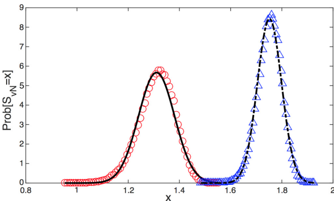
FIG. 4. Full probability density of S_{vN} from numerical diagonalization with N = 5 , M = 8 (red circles) and N = 8 , M = 12 (blue triangles), compared with Gaussian curves with mean and variance as in (53) and (57), respectively.
