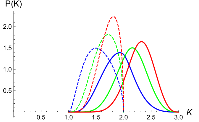
FIG. 5. Probability distribution function P_{N=2}(K) for N = 2 [Eq. (62)] (dashed lines) and P_{N=3}(K) for N = 3 [Eq. (63)] (solid lines). The curves from the left to the right correspond to M = 4, 6 , and 8 .
