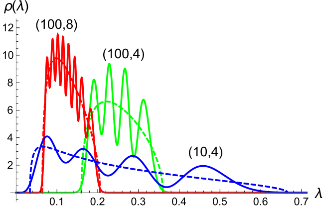
FIG. 1. The spectral density \rho_1^{(\text{FT})}(\lambda) for the unitary fixed-trace ensemble in (47) for M = 100 and N = 8 (red), M = 100 and N = 4 (green), and M = 10 and N = 4 (blue). The dashed lines define the Marčenko-Pastur-type distribution in (43) corresponding to these values of M and N .
