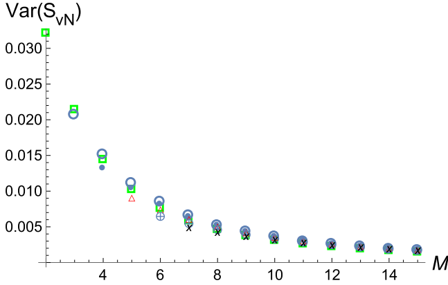
FIG. 3. The variance \text{Var}(S_{vN}) in (57), as a function of M for N = 2 (squares), N = 3 (open circles), N = 4 (filled circles), N = 5 (triangles), N = 6 (crossed triangles), and N = 7 (crosses).
