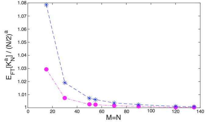
FIG. 7. \mathbb{E}_{\text{FT}}\{K_N^a\}/(N/2)^a as a function of M=N . Numerical simulations for a=3.2 (purple dots) and a=6.2 (blue stars) confirm that the ratio converges to 1, as predicted theoretically.
