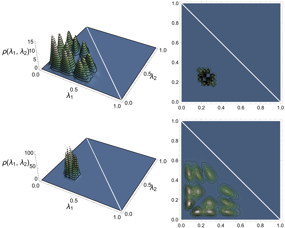
FIG. 2. The two-level density \rho_2^{(\text{FT})}(\lambda_1, \lambda_2) for the fixed-trace ensemble in (50) versus \lambda_1 and \lambda_2 . Top: M = 10 and N = 4 , side view (left) and top view (right). Bottom: M = 100 and N = 4 , side view (left) and top view (right).
