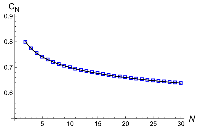
FIG. 8. Normalization constant C_N [Eq. (99)] (symbols), as a function of N . The solid curve is the asymptotic result in (D10).
