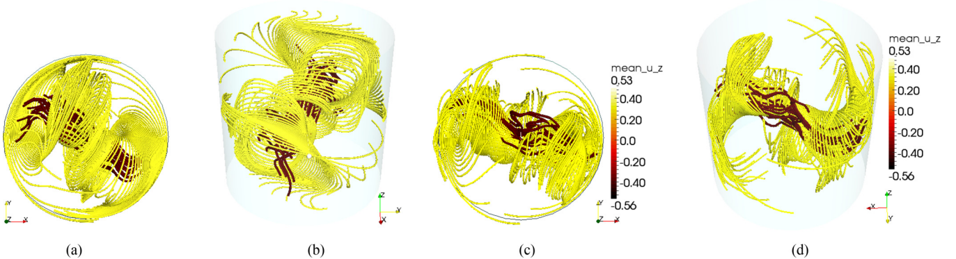
FIG. 6. Streamlines of the mean velocity field [in yellow (light gray)] and of the mean vorticity field [in red (dark gray)] in the precession frame. Illustrated are 100 streamlines for \mathbf{u} with endpoints distributed uniformly on the Ox axis and 20 streamlines for \nabla \times \mathbf{u} with endpoints distributed uniformly on a sphere of radius 0.2: (a–b) R_e = 1200 and (c–d) R_e = 4000 .
