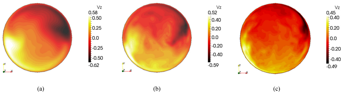
FIG. 4. Snapshots of contours of the axial velocity in the equatorial plane in the precession frame: (a) at t = 302 and Re = 1200 , (b) at t = 235 and Re = 4000 , and (c) at t = 850 and Re = 15000 .
