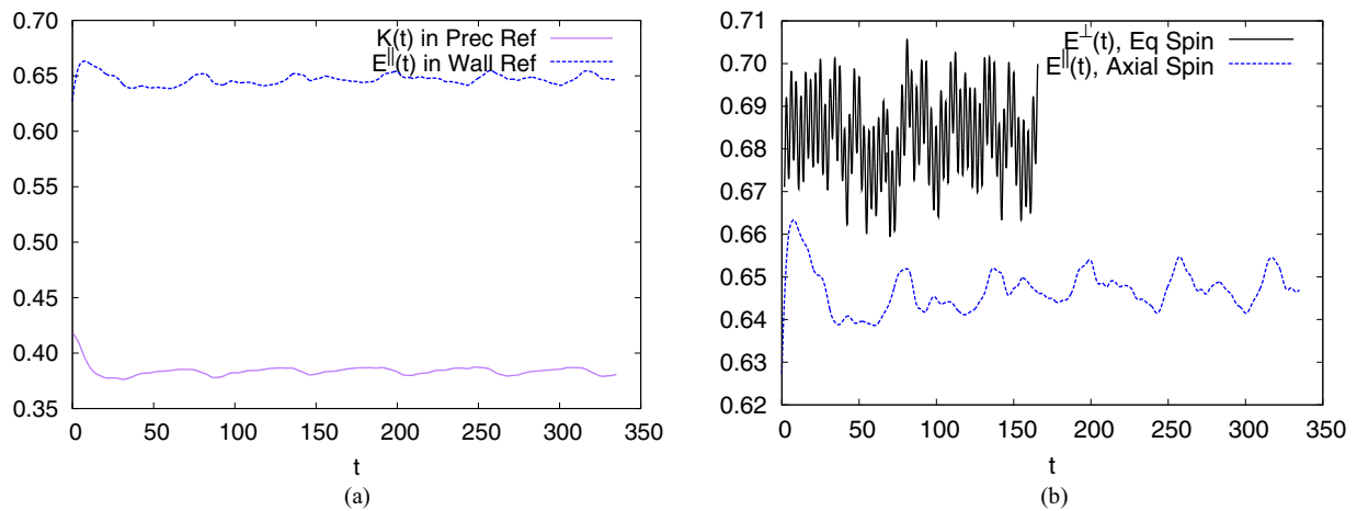
FIG. 8. (a) Time evolution at R_e = 1200 of the kinetic energy K(t) in the precession frame as in Fig. 2(a) and of the transformed kinetic energy E^{ll}(t) in the mantle frame for the axial spin case. (b) Comparison of the kinetic energy in the mantle frame for the axial and the equatorial spin cases at R_e = 1200 .
