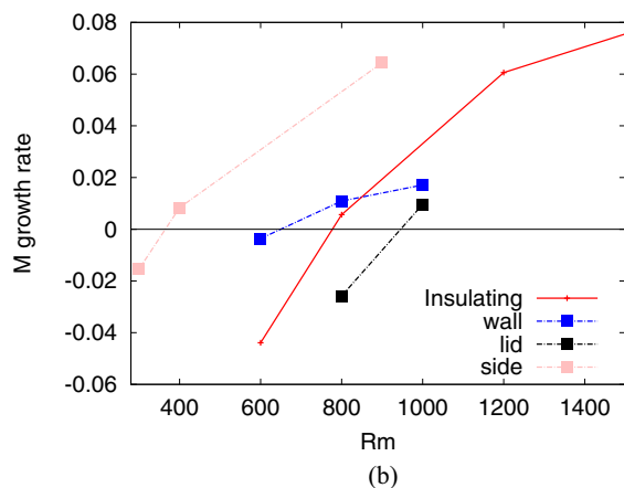
FIG. 14. Conducting walls: (a) Time evolution of the magnetic energy M(t) in the conducting fluid at R_e = 1200 and various R_m as indicated (in lin-log scale) for the “side” case; (b) Growth rates of the magnetic field energy as a function of R_m for various configurations. The values are for R_e = 1200 , and the thickness of either conducting wall type is taken as 0.1R , with a relative conductivity \sigma_r = 4.5 and relative magnetic permeability \mu_r = 1 .
