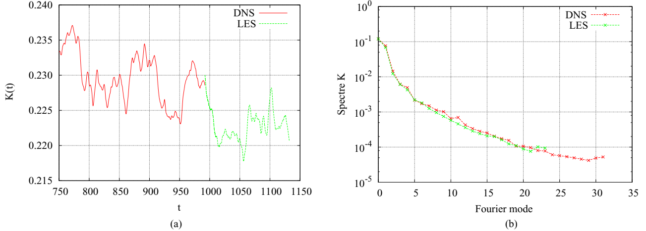
FIG. 19. Comparisons between DNS and LES results at R_e = 4000 in the hydrodynamic regime. (a) Evolution of total kinetic energy K(t) [zoom from Fig. 2(b)], (b) kinetic energy spectrum at final time as a function of the Fourier modes ( 0 \leq m \leq 31 with DNS and 0 \leq m \leq 23 with LES).
