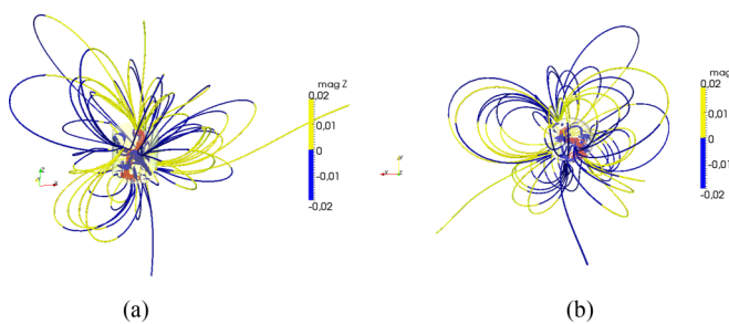
FIG. 18. Equatorial spin case: snapshot in the mantle frame at t = 395 at R_e = 1200 and R_m = 2400 of the vorticity field lines [gray (red)] and the magnetic field lines colored by the axial component [light gray (yellow) for positive axial magnetic field component and black (blue) for negative axial magnetic field component]. (a) The view is seen from the side ( Ox is the spin axis, Oz the precession axis), (b) from the top.
