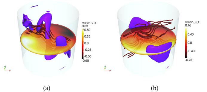
FIG. 12. Time-averaged velocity field at Re = 1200 for the axial and equatorial spin cases: vorticity field lines [red (dark gray)], contours of the axial velocity component in the equatorial plane and isosurface of |\mathbf{u}|^2 : (a) axial spin case (with |\mathbf{u}|^2 at 0.3% of maximum in the precession frame), (b) equatorial spin case (with |\mathbf{u}|^2 at 70% of maximum in the mantle frame).
