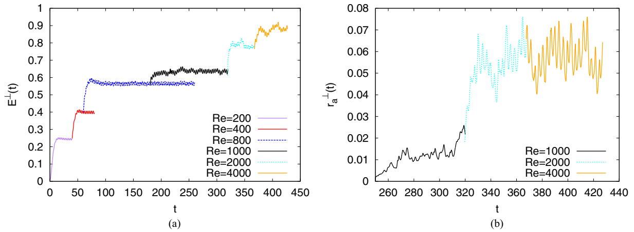
FIG. 7. Time evolution of (a) the total kinetic energy E^\perp(t) and (b) the asymmetry ratio r_a^\perp(t) = E_a^\perp(t)/E^\perp(t) in the mantle frame at different Reynolds numbers R_e in the equatorial spin case.
