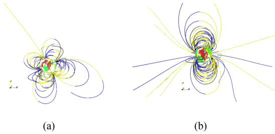
FIG. 15. Conducting walls: Snapshots at (a) R_e = 1200 , R_m = 1000 for the “lid” case and (b) R_e = 1200 , R_m = 900 for the “side” case showing vorticity field lines (red lines inside the cylinder) and magnetic field lines colored by the axial component [yellow (blue) for positive (negative) h_z component].
