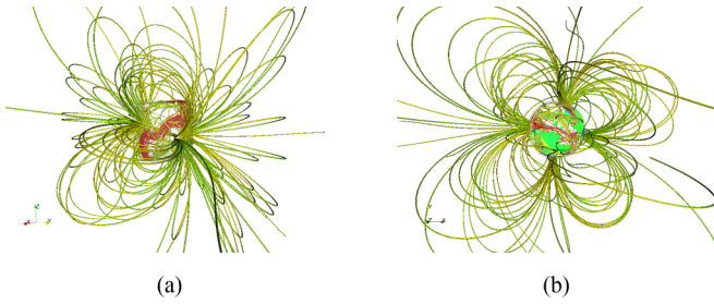
FIG. 13. Snapshot at R_e = 1200 , R_m = 2400 for the “insulating” case showing vorticity field lines (red lines inside the cylinder) and magnetic field lines colored by the axial component [yellow (green) for positive (negative) h_z component]: (a) perspective view, (b) from the top of the cylinder (in the precession frame). From Ref. [10].
