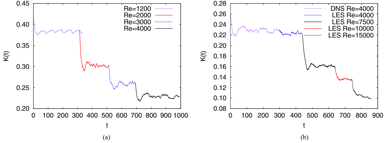
FIG. 2. Time evolution of the total kinetic energy K(t) in the precession frame for different Reynolds numbers as indicated: (a) DNS at R_e = 1200, 2000, 3000, 4000 ; (b) DNS computation at R_e = 4000 and LES computations at R_e = 4000, 7500, 10000, 15000 .
