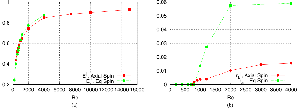
FIG. 10. Comparisons between the axial and equatorial spin cases in the mantle frame: (a) time-averaged kinetic energy E^{\parallel} and E^{\perp} as a function of Re ; (b) time-averaged asymmetry ratio E_a^{\parallel}/E^{\parallel} and E_a^{\perp}/E^{\perp} as a function of Re .
