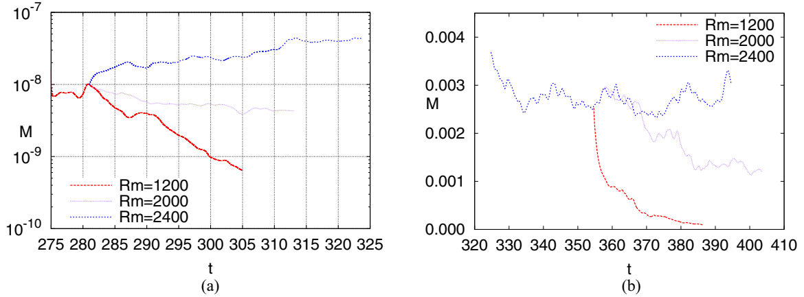
FIG. 17. Equatorial spin case: Time evolution of the magnetic energy M(t) in the conducting fluid (a) in the linear regime from t = 275 at R_e = 1200 and various R_m as indicated (in lin-log scale) and (b) in the nonlinear regime.
