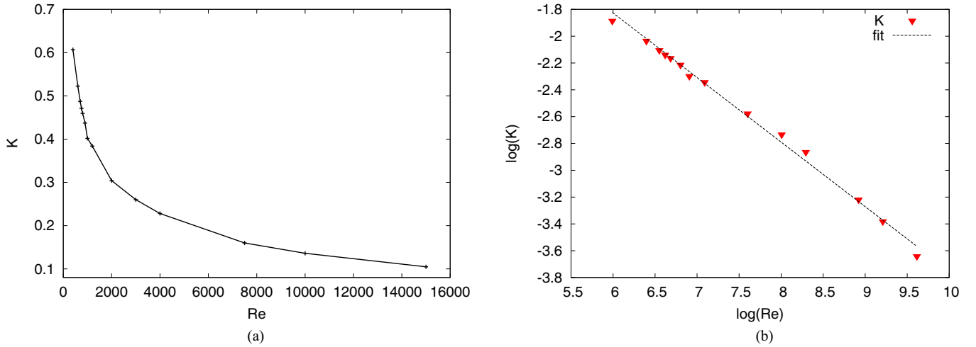
FIG. 3. Total (time-averaged) kinetic energy K in the precession frame as a function of the Reynolds number Re : (a) in linear scale and (b) in log-log scale with the fit Re^{-0.48} .
