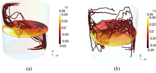
FIG. 5. Streamlines of the instantaneous vorticity field [in red (dark gray)] from a perspective point of view and contours of the axial velocity in the equatorial plane: (a) R_e = 1200 and (b) R_e = 15000 .
