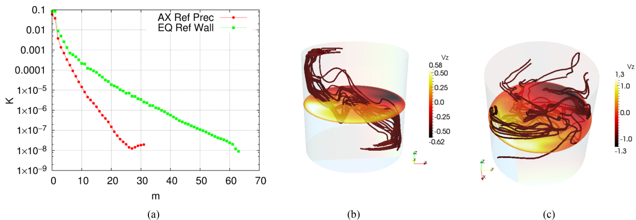
FIG. 9. Comparison between the axial and equatorial spin cases: kinetic energy azimuthal spectra as a function of the azimuthal mode m (a) and snapshot at R_e = 1200 of the vorticity field lines [red (dark gray)] and contours of the axial velocity component in the equatorial plane, (b) axial spin case [same as Fig. 5(a) in the precession frame], (c) equatorial spin case (in the mantle frame).
