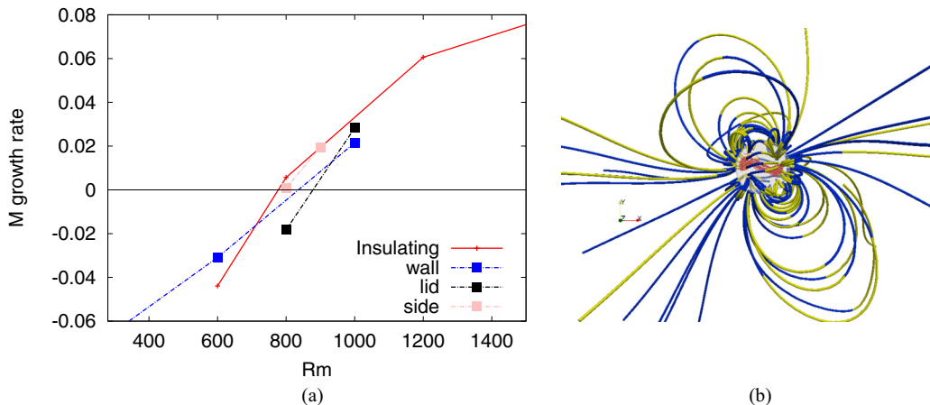
FIG. 16. Ferromagnetic walls: (a) Growth rates of the magnetic field energy as a function of R_m for various configurations. The values are for R_e = 1200 , and the thickness of either ferromagnetic wall type is taken as 0.1R , with a relative conductivity \sigma_r = 1 and relative magnetic permeability \mu_r = 65 . (b) Snapshot at R_e = 1200 , R_m = 1000 for the “wall” case showing vorticity field lines (red lines inside the cylinder) and magnetic field lines colored by the axial component [yellow (blue) for positive (negative) h_z component]. View from the top.
