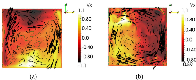
FIG. 11. Equatorial spin case: flow in the mantle frame, in the meridian plane ( x = 0 ) orthogonal to the spin axis, at Re = 1200 and 4000 . The black arrows represent the 2D velocity field (u_y, u_z) in the plane ( x = 0 ), and the contour levels show the u_x component in this plane. The green line shows the contour level u_x = 0 .
