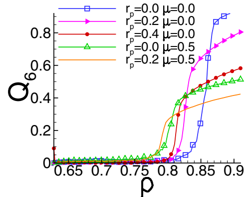
FIG. 8. Order parameter showing distribution of the angles between contacts.
