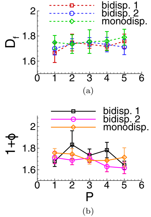
FIG. 11. (a) Fractal dimension, D_f , and (b) 1 + \phi obtained from experiments carried out with photoelastic particles, as a function of the applied pressure. Bidisperse 1 and 2 refer to the systems of large and medium particles and large and small particles, respectively (see the text).
