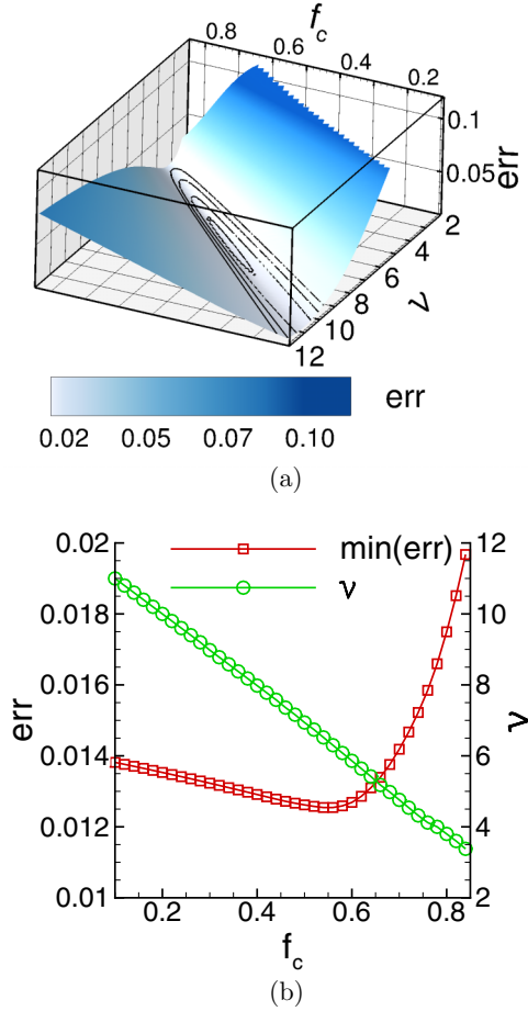
FIG. 10. Error plot for the r_p = 0.0 , \mu = 0.0 system at \rho = 0.9 : (a) err as a function of f_c and \nu ; the black lines are slices through different values of err and (b) minimum of err (red line with squares) as a function of f_c ; here for each f_c value we choose \nu that minimizes err; the used values of \nu are shown by the green line with circles. Note different range compared to Fig. 4.
