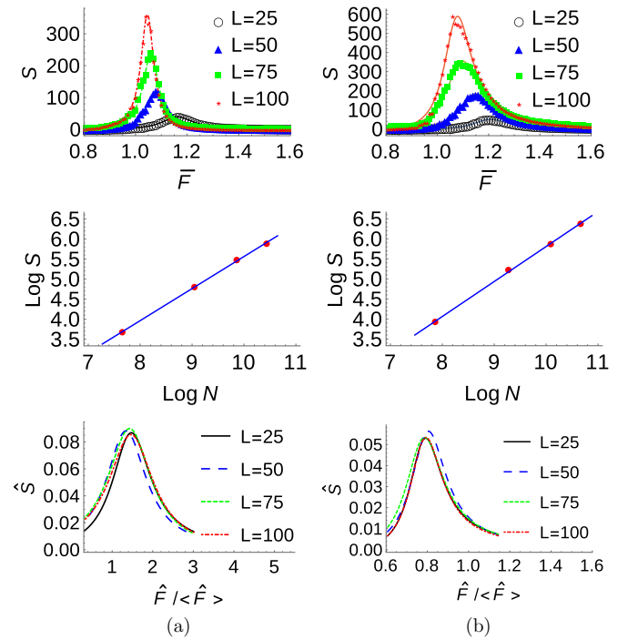
FIG. 3. (a) Reference and (b) r_p = 0.0 , \mu = 0.0 system at \rho = 0.9 showing (top to bottom) mean cluster size S ; magnitude of the peak of S versus the total number of contacts, N , for different system sizes, L ; and collapse of the rescaled curves, \hat{S} vs. force threshold, \hat{F} , normalized by the rescaled average force, \langle \hat{F} \rangle (see the text for definitions of the rescaled quantities). Note different range of axes in (a) and (b).
