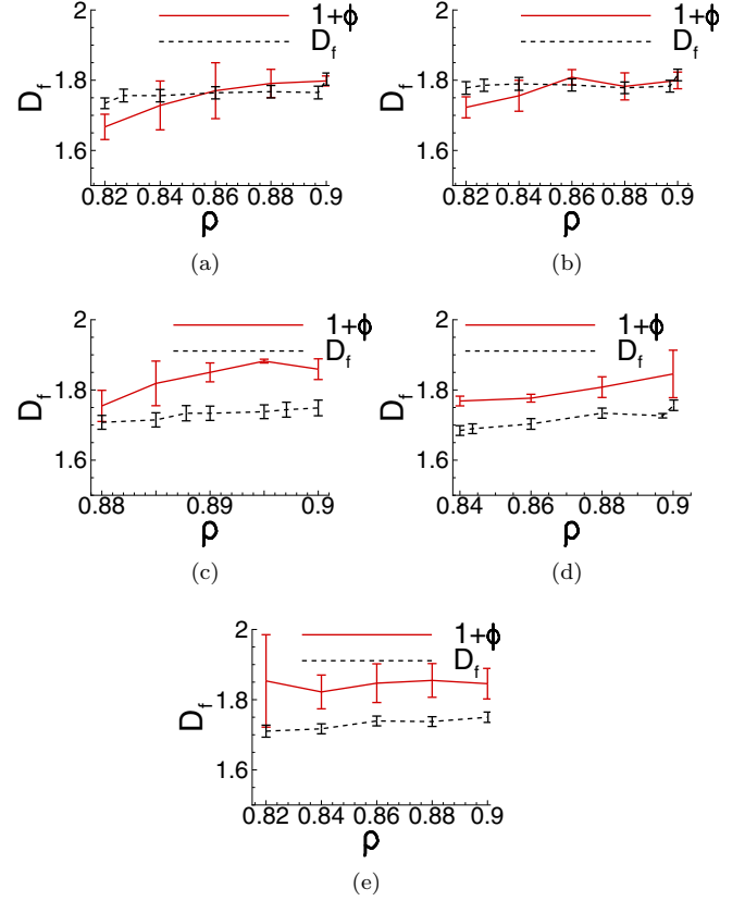
FIG. 6. Fractal dimension, D_f , and scaling exponent 1 + \phi as a function of \rho : (a) r_p = 0.0, \mu = 0.5 (b) r_p = 0.2, \mu = 0.5 (reference system) (c) r_p = 0.0, \mu = 0.0 , (d) r_p = 0.2, \mu = 0.0 , and (e) r_p = 0.4, \mu = 0.0 . For D_f , the error bars represent standard error; for \phi , the error bars are derived from the accuracy of the fit, as explained in the text. The jamming packing fractions for the considered systems are \rho_J = 0.804, 0.789, 0.861, 0.827 , and 0.805 , respectively [24].
