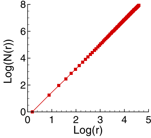
FIG. 5. Number of subdomains covering the percolating cluster, \mathcal{N}(r) , as a function of the distance, r in log-log scale for the reference case at \rho = 0.9 .
