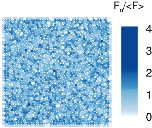
FIG. 2. Reference system at \rho = 0.9 .
