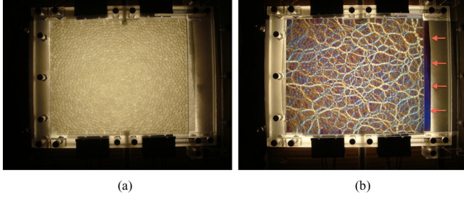
FIG. 1. Experimental images of a two-dimensional system of photoelastic particles, obtained (a) without and (b) with cross-polarizer. The arrows indicate the side of the container where pressure is applied.
