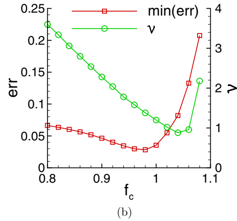
FIG. 4. Error plot for the reference system at \rho = 0.9 : (a) \text{err} as a function of f_c and \nu ; the black lines are slices through different values of \text{err} and (b) minimum of \text{err} (red line with squares) as a function of f_c ; here for each f_c value we choose \nu that minimizes \text{err} ; the used values of \nu are shown by the green line with circles.
