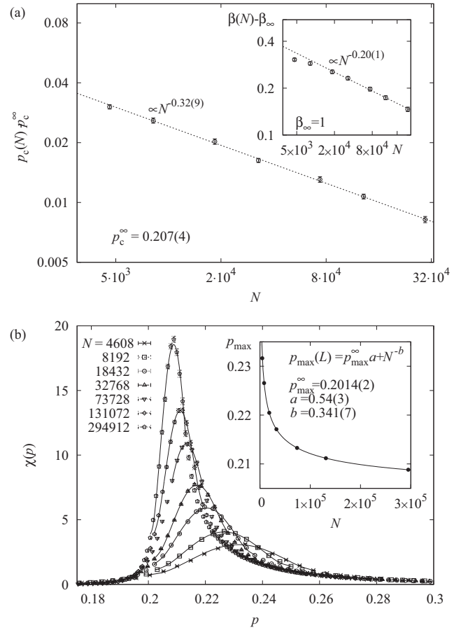
FIG. 5. Finite-size scaling analysis of the relative size s_{\max} of the largest cluster of sites for the site-percolation problem on the small-world enhanced chimera graphs (see Sec. IV D). (a) Scaling of the effective system-size-dependent estimate of p_c(N) . The inset shows a scaling of \beta(N) , as discussed in the text. (b) Fit of fifth-order polynomials to the finite-size fluctuations to estimate the system-size-dependent peak positions p_{\max}(N) . The inset shows the extrapolation to the asymptotic critical point p_{\max}^\infty , as discussed in the text.
