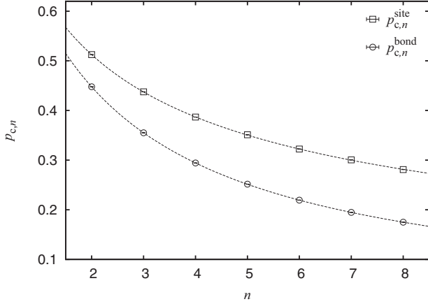
FIG. 4. Bond and site percolation thresholds for chimeralike graphs built from K_{n,n} subgraphs. The percolation thresholds decrease with increasing average vertex degree and thus of n , the cell size. The dashed lines represent fits to functions of the form f(n) = a(n - \Delta n)^{-b} (see text for details).
