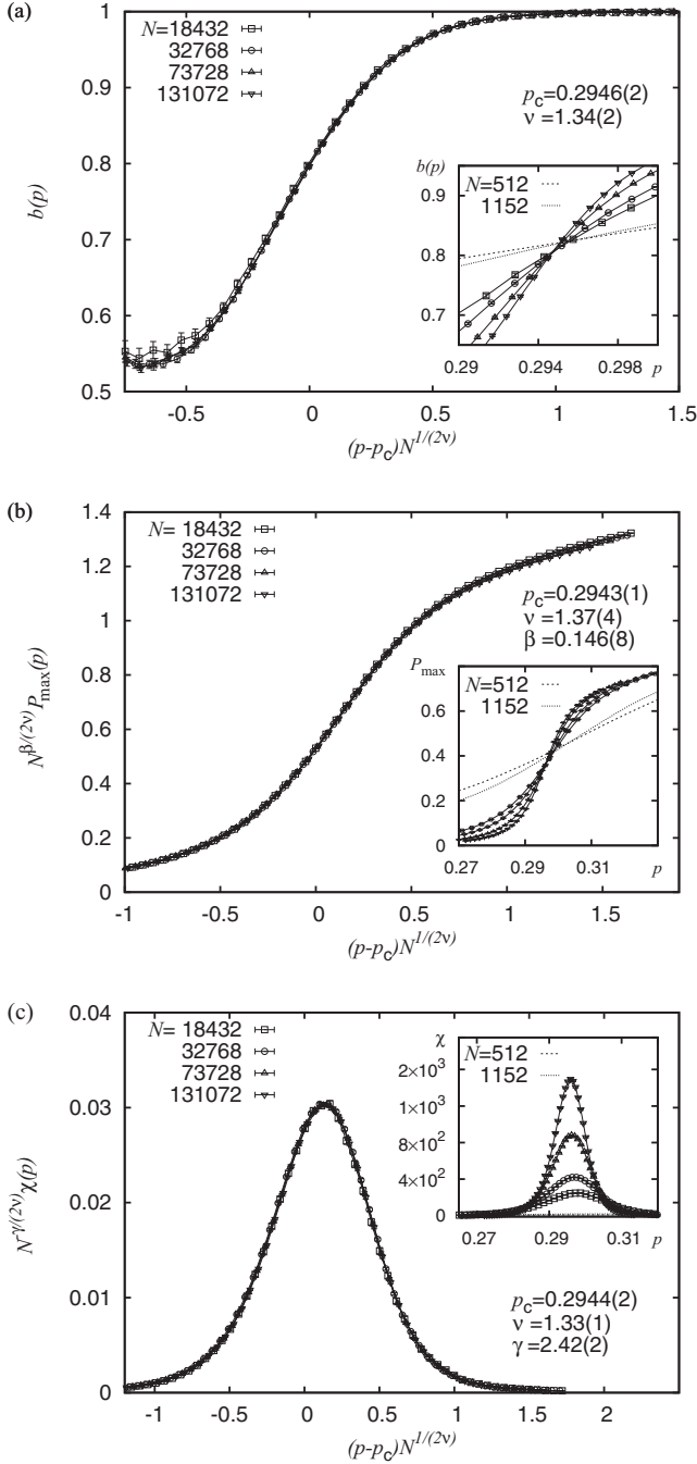
FIG. 3. Finite-size scaling analysis of the relative size s_{\max} of the largest cluster of sites for the bond-percolation problem on chimera graphs. The main panels always show the scaled data according to Eq. (1), whereas the insets display the unscaled data in the vicinity of the critical point. (a) Binder ratio b(p) , (b) disorder-averaged order parameter P_{\max}(p) , and (c) fluctuation \chi(p) = N \times \text{var}(s_{\max}) of the order parameter. Note that the insets feature two additional data curves, illustrating the statistical properties of small chimera graphs of current quantum annealing machines with N = 512 and 1152 qubits (sites).
