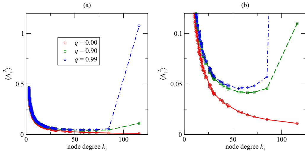
FIG. 3. (Color online) (a) Average size of the fluctuations at the nodes as a function of their degree for a BA network with N = 1000 and \langle k \rangle \approx 6 . Open symbols correspond to results based on exact numerical diagonalization of the Laplacian and employing Eqs. (14) and (15). Plus symbols (of matching colors) correspond to the direct numerical integration of the stochastic delay-differential Eq. (5) with \Delta t = 5 \times 10^{-6} . The connecting lines are the average of the degree class from these numerical integrations. (b) Same data as in (a) but on smaller vertical scales.
