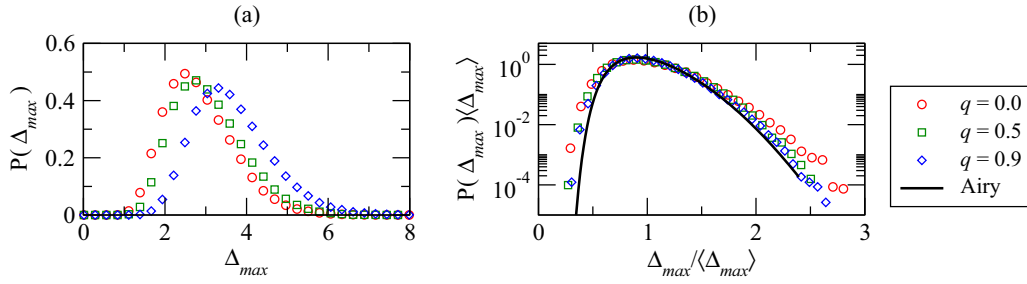
FIG. 8. (Color online) (a) Extreme fluctuation distributions and (b) scaled version of the same data for several delays for a regular one-dimensional lattice with N = 1000 . Symbols are the results found by numerically integrating Eq. (5) using \Delta t = 5 \times 10^{-6} . The solid line corresponds to the predicted asymptotic Airy limit distribution [57,58].
