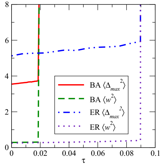
FIG. 1. (Color online) The typical behavior of the steady-state average width and the expected extreme as a function of the delay \tau for an ER and a BA network with N = 1000 and \langle k \rangle \approx 6 .
