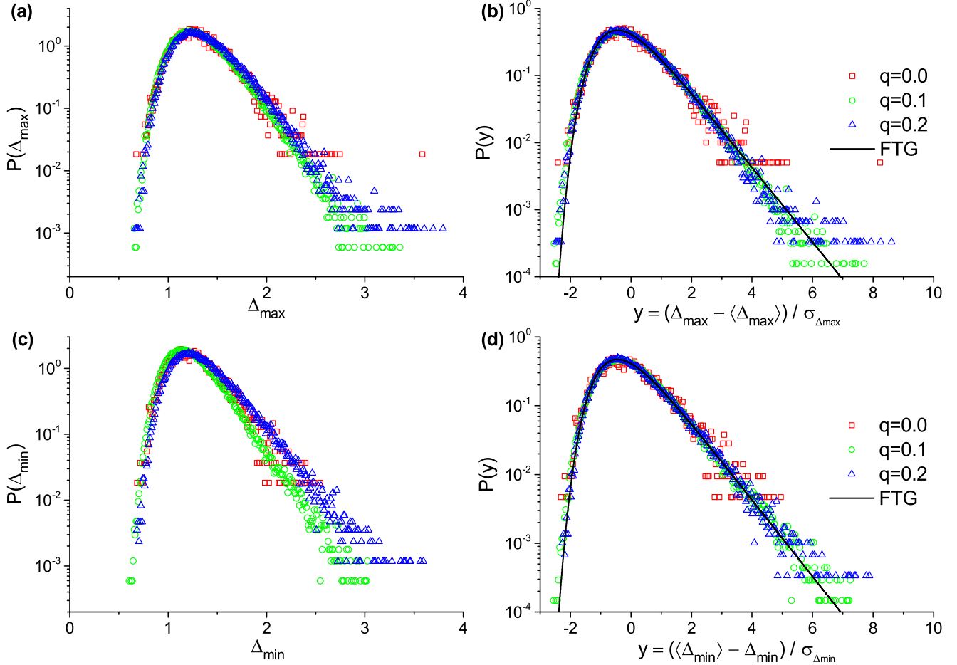
FIG. 15. (Color online) Extreme fluctuation distribution (in the quasistationary period) in SW networks with N = 100 , \langle k \rangle \approx 6 , nonlinear coupling \nu = 0.1 [Eq. (20)], and various relative time delays q = \tau/\tau_c . (a) Distributions of the extreme fluctuations above the mean, \Delta_{\max} = h_{\max} - \bar{h} ; (b) scaled distributions of the extreme fluctuations above the mean (with zero mean and unit variance); (c) distributions of the extreme fluctuations below the mean, \Delta_{\min} = \bar{h} - h_{\min} ; (d) scaled distributions of the extreme fluctuations below the mean (with zero mean and unit variance). The solid line in (b) and (d) corresponds to the FTG limit distribution [Eq. (4)].
