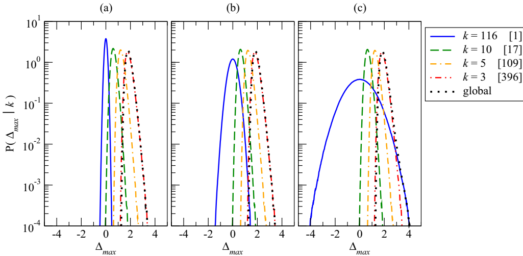
FIG. 7. (Color online) Contribution of a few selected degree classes for a BA network (including k_{\min} = 3 and k_{\max} = 116 ) with N = 1000 and \langle k \rangle \approx 6 for (a) q = 0.0 , (b) q = 0.9 , and (c) q = 0.99 . Results are obtained from numerical integration of the stochastic delay-differential equations Eq. (5) with \Delta t = 5 \times 10^{-6} . The numbers in brackets in the legends indicate the number of nodes in the corresponding degree class.
