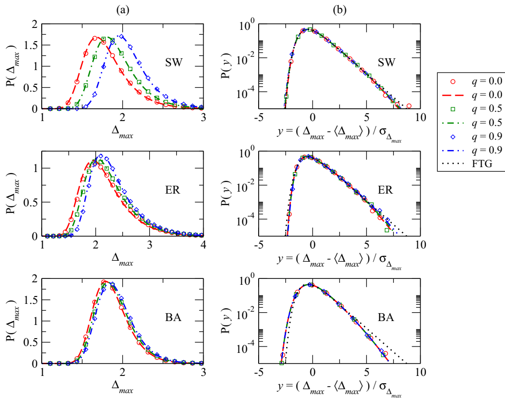
FIG. 5. (Color online) (a) Extreme fluctuation distributions and (b) rescaling of the same for several delays for SW, ER, and BA networks with N = 1000 and \langle k \rangle \approx 6 . The various curves correspond to the same delay fraction q for both (a) and (b). Lines are predictions based on exact numerical diagonalization and employing Eqs. (14), (15), and (19). Symbols correspond to the numerical integration of the stochastic delay-differential equations Eq. (5) with \Delta t = 5 \times 10^{-6} . The dotted curves in all panels correspond to the scaled FTG density, Eq. (4).
