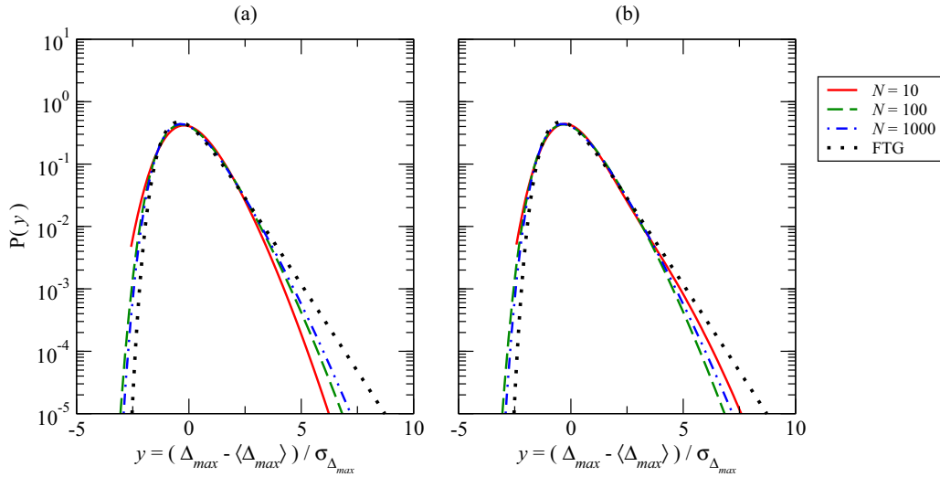
FIG. 4. (Color online) Finite-size behavior of the distribution of the extreme fluctuations for BA networks with \langle k \rangle \approx 6 and relative delays (a) q = 0.5 and (b) q = 0.9 obtained by numerically integrating Eq. (5) using \Delta t = 5 \times 10^{-6} . The dotted curves in both panels correspond to the scaled FTG density, Eq. (4).
