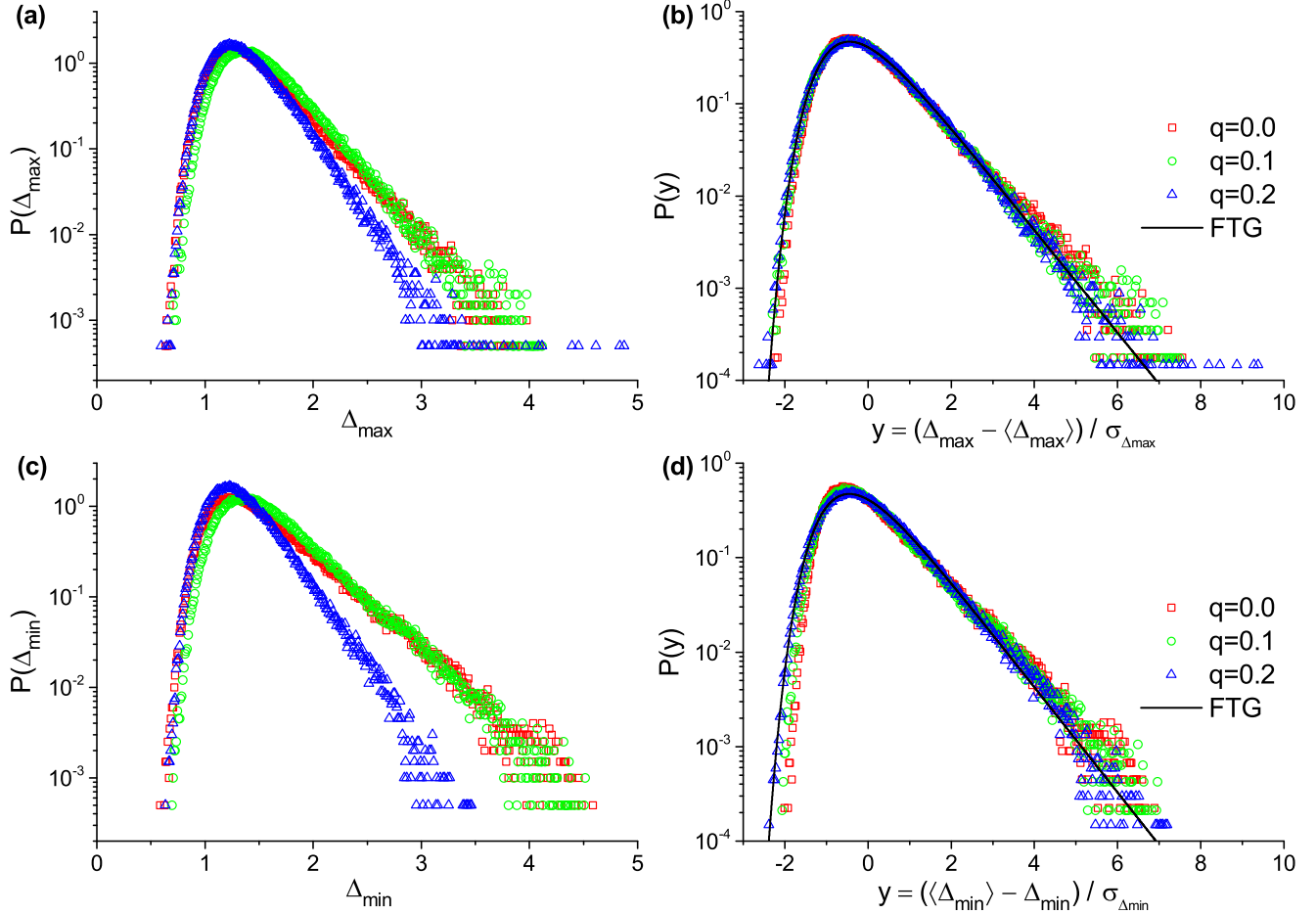
FIG. 14. (Color online) Extreme fluctuation distribution (in the quasistationary period) in ER networks with N = 100 , \langle k \rangle \approx 6 , nonlinear coupling \nu = 0.1 [Eq. (20)], and various relative time delays q = \tau/\tau_c . (a) Distributions of the extreme fluctuations above the mean, \Delta_{\max} = h_{\max} - \bar{h} ; (b) scaled distributions of the extreme fluctuations above the mean (with zero mean and unit variance); (c) distributions of the extreme fluctuations below the mean, \Delta_{\min} = \bar{h} - h_{\min} ; (d) scaled distributions of the extreme fluctuations below the mean (with zero mean and unit variance). The solid line in (b) and (d) corresponds to the FTG limit distribution [Eq. (4)].
