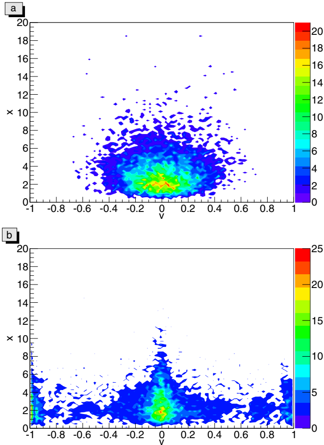
FIG. 1. (Color online) Test 1: The particles solution with N = 10000 particles and linear H . (a) High diffusion in conviction and reduced self-thinking compared to (b) low diffusion in conviction and high self-thinking.
