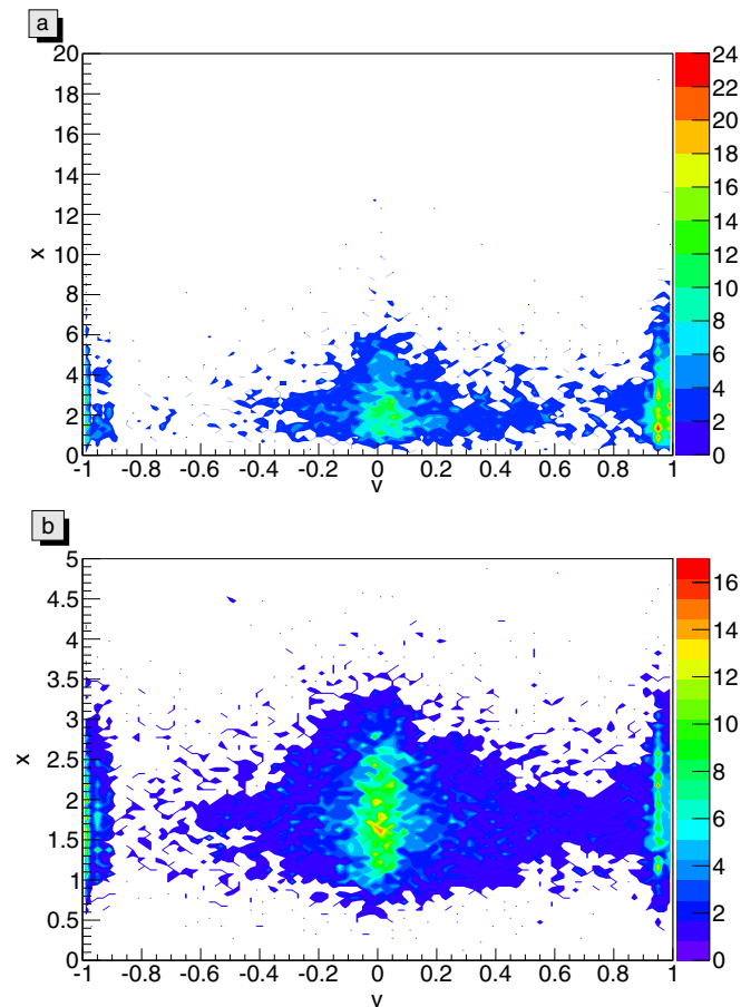
FIG. 3. (Color online) Initial asymmetry in opinion leads to different opinion-conviction distributions. (a) H(x) = x and (b) H(x) = \sqrt{x} .
