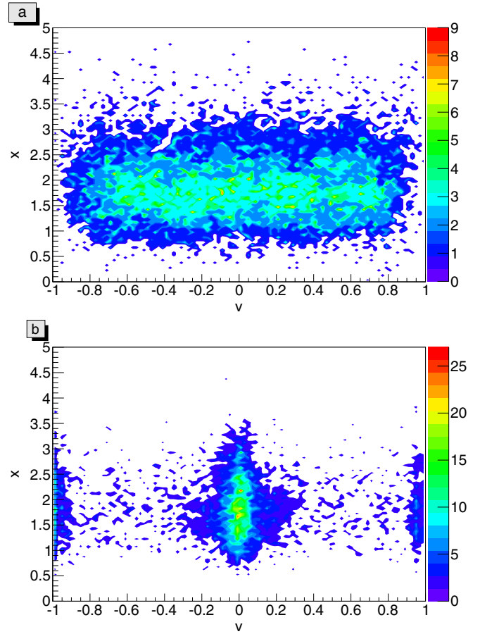
FIG. 2. (Color online) Test 2: The particles solution with N = 10000 particles and H(x) = \sqrt{x} . (a) High diffusion in conviction and reduced self-thinking compared to (b) low diffusion in conviction and high self-thinking.
