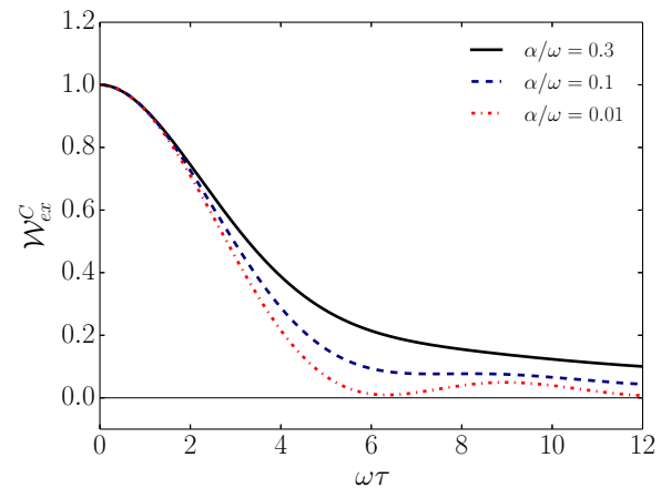
FIG. 8. (Color online) Excess work \mathcal{W}_{\text{ex}}^C in units of (\delta\varphi)^2\Psi(0)/2 for the linear protocol g_\varphi(t) = t/\tau and the relaxation function (33).
