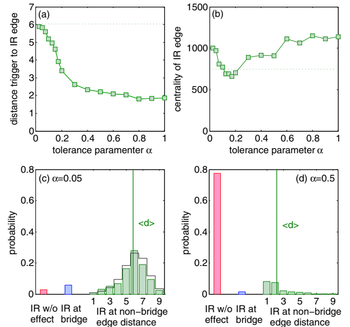
FIG. 8. (Color online) Nonlocality of intentional removal for preventing cascading failures. (a) Average distance of the intentionally removed edge and the trigger edge as a function of the tolerance parameter \alpha . (b) Average betweenness centrality of the intentionally removed edge as a function of the tolerance parameter \alpha . In panels (a) and (b) we disregard cases where IR has no effect or disconnects the grid. The dashed line shows the average shortest path distance L and the average centrality, respectively, for comparison. (c, d) Histogram of the distances of the intentionally removed edge and the trigger edge in the case that IR leads to an increase of the final cluster size without disconnecting the network (green bars on the right) for two values of \alpha . Gray lines show the distance distribution for all edges in the network for comparison. The left red bar indicates the probability that IR has no effect and the middle blue bar the probability that IR disconnects the grid. Results are averaged over all trigger edges for a WS network with N = 500 , k = 4 , and q = 0.2 .
