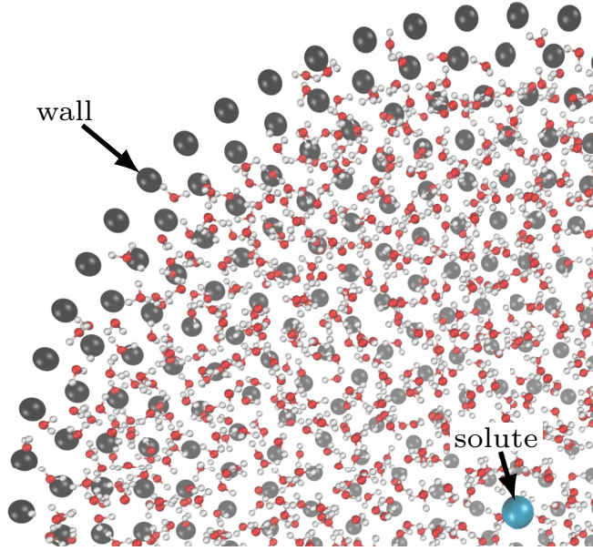
FIG. 1. (Color online) Cut through the simulated system: the sphere in the center of the droplet is the solute; the black spheres are the wall particles.
