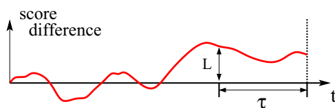
FIG. 10. (Color online) One team leads by L points when a time \tau is left in the game.
