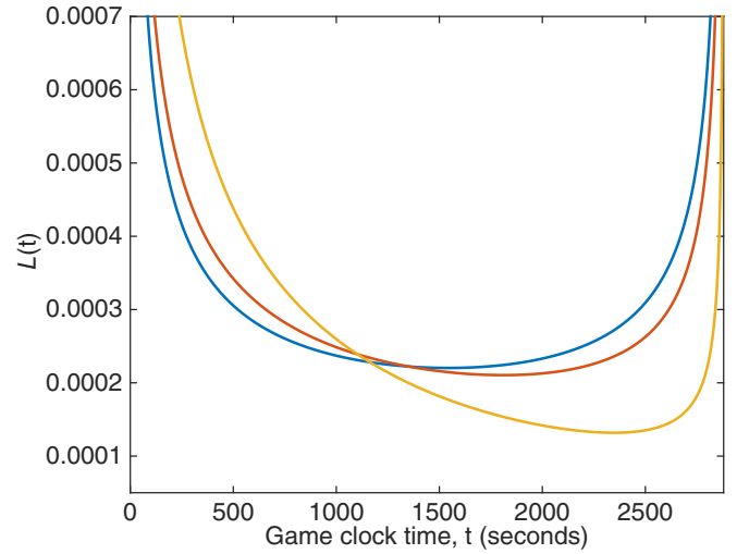
FIG. 7. (Color online) The distribution \mathcal{L}(t) for nonzero bias [Eq. (12)]. The diffusion coefficient is the empirical value D = 0.0391 , and bias values are v = 0.002 , v = 0.004 , and v = 0.008 (increasingly asymmetric curves). The central value of v roughly corresponds to average NBA game-scoring bias if diffusion is neglected.
