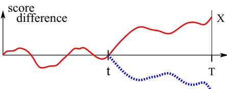
FIG. 4. (Color online) Schematic score evolution in a game of time T . The subsequent trajectory after the last lead change must always be positive (solid) or always negative (dashed).
