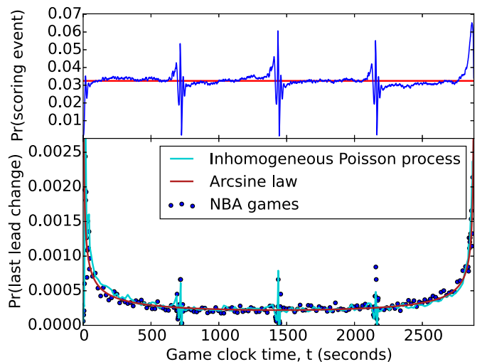
FIG. 5. (Color online) Upper: Empirical probability that a scoring event occurs at time t , with the game-average scoring rate shown as a horizontal line. The data is aggregated in bins of 10 sec. each; the same binning is used in Fig. 14. Lower: Distribution of times \mathcal{L}(t) for the last lead change.
