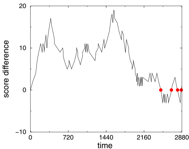
FIG. 1. (Color online) Evolution of the score difference in a typical NBA game: the Denver Nuggets vs the Chicago Bulls on 26 November 2010. Dots indicate the four lead changes in the game. The Nuggets led for 2601 out of 2880 total seconds and won the game by a score of 98–97.
