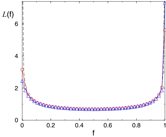
FIG. 6. (Color online) The distribution of time for the last lead change, \mathcal{L}(f) , as a function of the fraction of steps f for a 94-step random walk with persistence parameter p = 0.36 as in the NBA ( \circ ) and p = 0.25 corresponding to stronger persistence ( \Delta ). The smooth curve is the arcsine law for p = 0.5 (no antipersistence).
