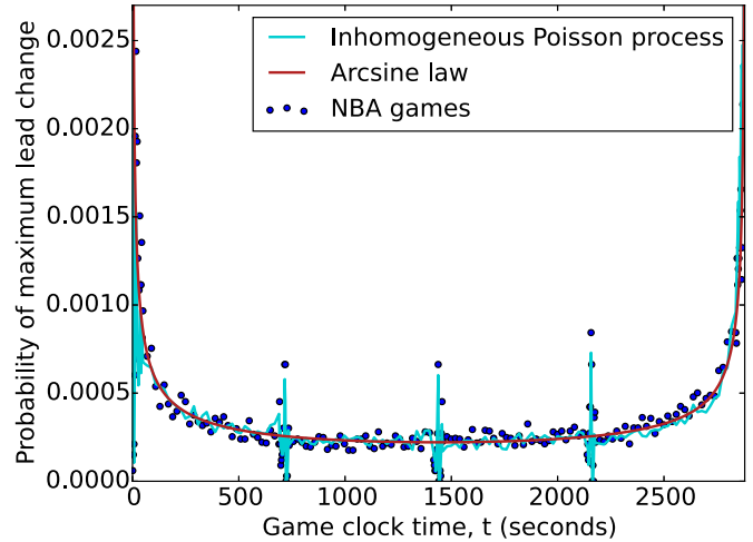
FIG. 9. (Color online) Distribution of times \mathcal{M}(t) for the maximal lead.
