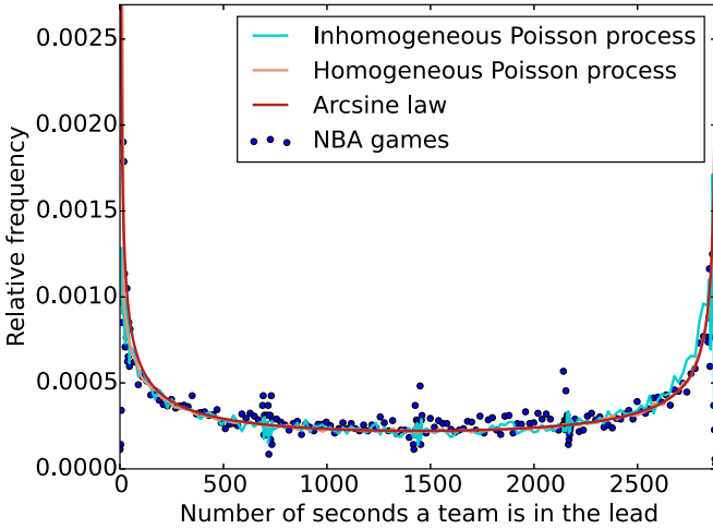
FIG. 3. (Color online) The distribution of the time that a given team holds the lead, \mathcal{O}(t) . The homogeneous Poisson process data is virtually indistinguishable from the arcsine law, while the inhomogeneous Poisson process roughly accounts for the end-of-quarter enhanced scoring rate.
