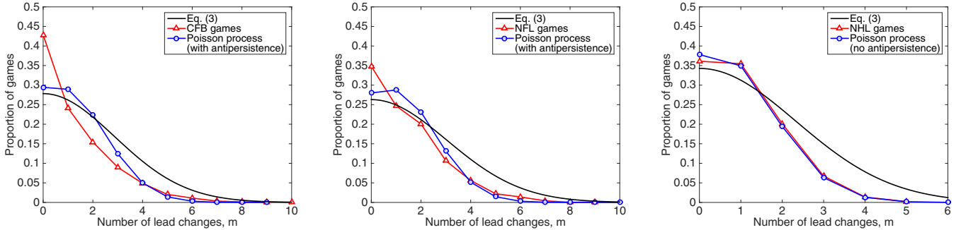
FIG. 13. (Color online) Distribution of the average number of lead changes per game, for CFB, NFL, and NHL, showing the prediction of Eq. (3), the empirical data, and the results of a simulation in which scoring events occur by a Poisson process with the game-specific scoring rate.
