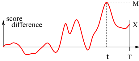
FIG. 8. (Color online) The maximal lead (which could be positive or negative) occurs at time t .
