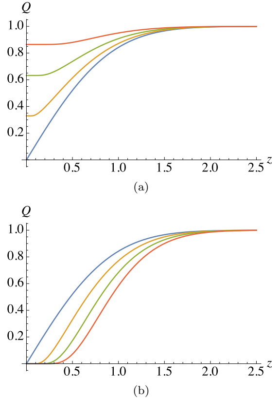
FIG. 12. (Color online) Probability that a lead is safe versus z = L/\sqrt{4D\tau} for (a) the stronger team is leading for Pe = \frac{1}{5}, \frac{1}{2}, and 1 (progressively flatter curves), and (b) the weaker team is leading for Pe = -\frac{2}{5}, -\frac{4}{5}, and -\frac{6}{5} (progressively shifting to the right). The case Pe = 0 is also shown for comparison.
