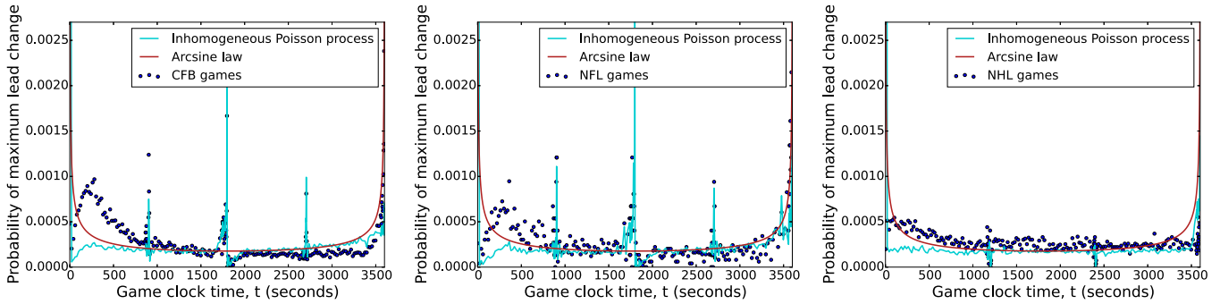
FIG. 15. (Color online) Distribution of times \mathcal{M}(t) for the maximal lead, for games of CFB, NFL, and NHL.
