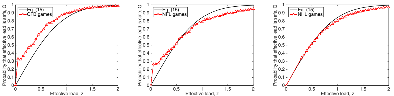
FIG. 16. (Color online) Probability that a lead is safe, for CFB, NFL, and NHL, versus the dimensionless lead z = L/\sqrt{4D\tau} . Each figure shows the prediction from Eq. (15) and the corresponding empirical pattern.
