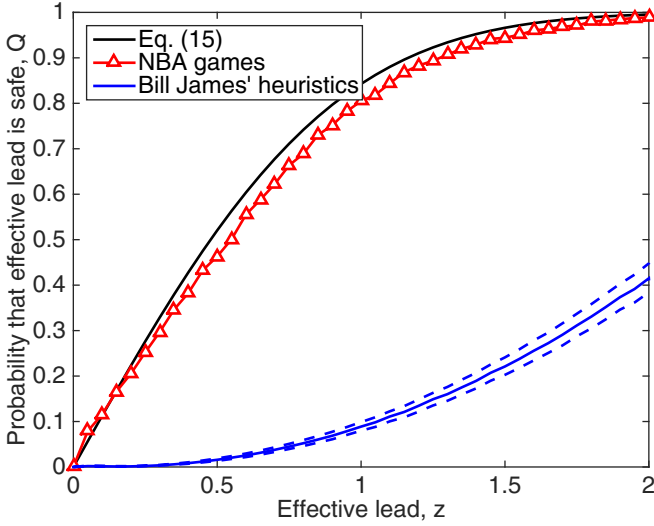
FIG. 11. (Color online) Probability that a lead is safe versus the dimensionless lead size z = L/\sqrt{4D\tau} for NBA games, showing the prediction from Eq. (15), the empirical data, and the mean prediction for Bill James' well-known "safe lead" heuristic.
