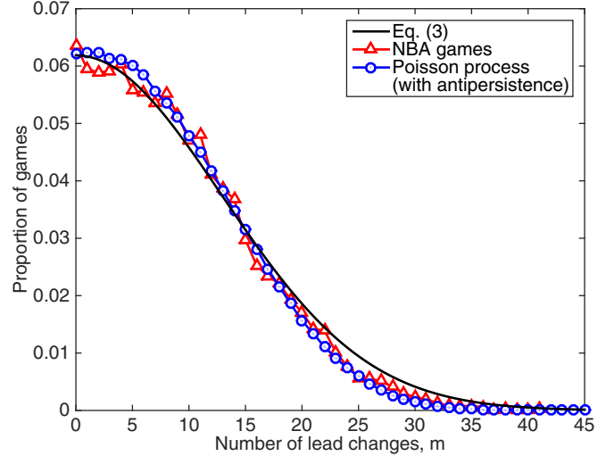
FIG. 2. (Color online) Distribution of the average number of lead changes per game in professional basketball.
