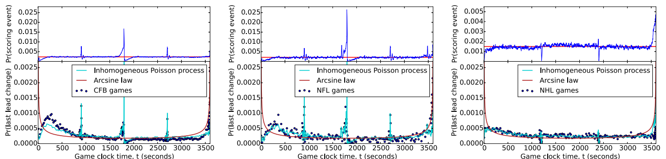
FIG. 14. (Color online) Upper: Empirical probability that a scoring event occurs at time t , with the game-average scoring rate shown as a horizontal line, for games of CFB, NFL, and NHL. Lower: Distribution of times \mathcal{L}(t) for the last lead change.
