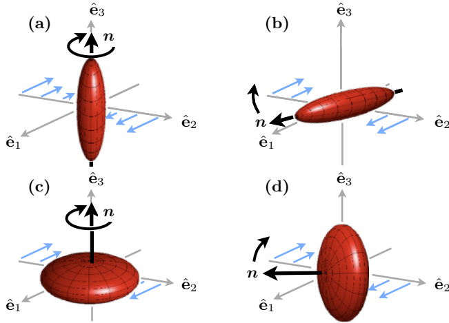
FIG. 1. (Color online) Spheroid in a simple shear. The flow direction is \hat{e}_1 , shear direction \hat{e}_2 , and the vorticity points in the negative \hat{e}_3 -direction. (a) Log-rolling of a prolate particle, \mathbf{n} is a unit vector along the symmetry axis of the particle. (b) Tumbling in the shear plane of a prolate particle. (c) Log-rolling of an oblate particle. (d) Tumbling of an oblate particle.
