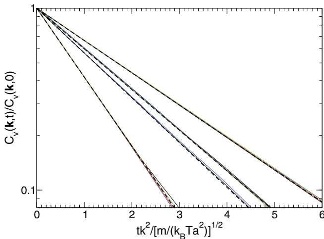
FIG. 1. (Color online) Transverse velocity autocorrelation functions of a MPC fluid for the collision-time steps h/\tau = 0.1, 1.0, 0.2 , and 0.5 (left to right). The k values are k = 2\pi n/L , with L = 30a and n = 1, 2, 3 , and 4 . The fit of the exponential function (17) (dashed lines) yields the kinematic viscosities presented in Table I.
