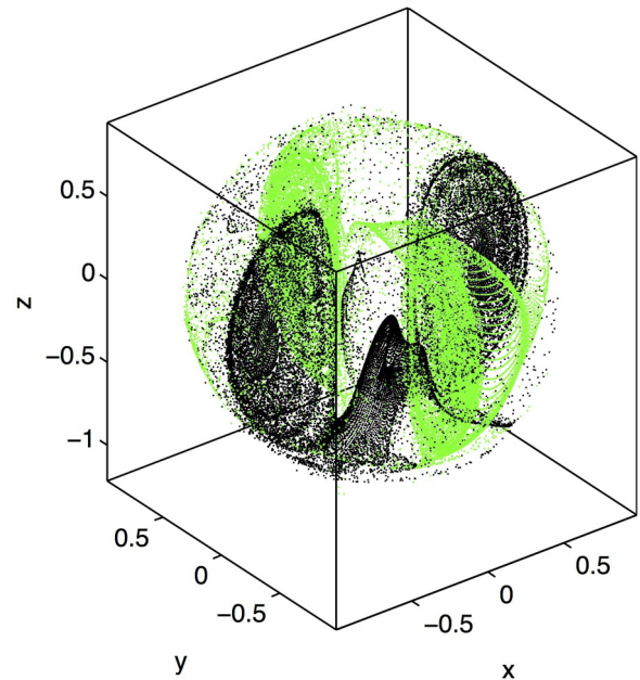
FIG. 7. (Color online) Complicated mixing structure is illustrated by advecting the coordinate planes with x = 0 (light gray; green online) and y = 0 (black) over 10 periods of the forcing.
