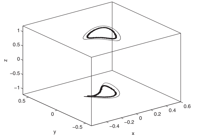
FIG. 5. Two periodic hyperbolic trajectories in (x, y, z) space for \varepsilon = 0.2 as defined by (20) and (21) parametrized over time interval [0, 2\pi] . The thin solid curves represent the desired motion. The thick curves with smaller radius correspond to the numerically approximated trajectories based on the controlled system (22).
