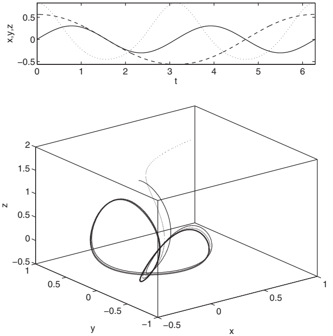
FIG. 1. Periodic hyperbolic trajectory \mathbf{x}_{(p)} for \varepsilon = 0.6 as defined by (15) over time interval [0, 2\pi] , with (x, y, z) represented by solid, dashed, and dotted curves, respectively (top panel). Solution curves (dotted and solid) of two initial conditions approaching the trajectory \mathbf{x}_{(p)}(t) (thick curve) in phase space (bottom panel).
