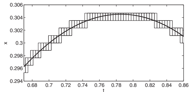
FIG. 3. A zoom in on Fig. 1 to show the numerical grid element method for determining the hyperbolic trajectories.
