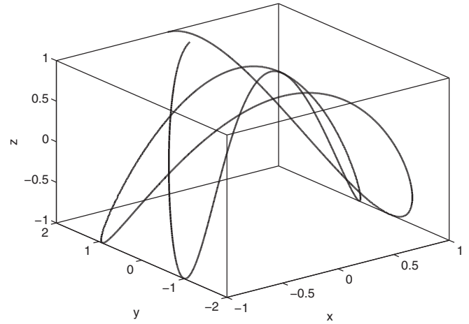
FIG. 2. Quasiperiodic hyperbolic trajectory \mathbf{x}_{(q)} for \varepsilon = 1 as defined by (17) on time interval [0, 4\pi] .
