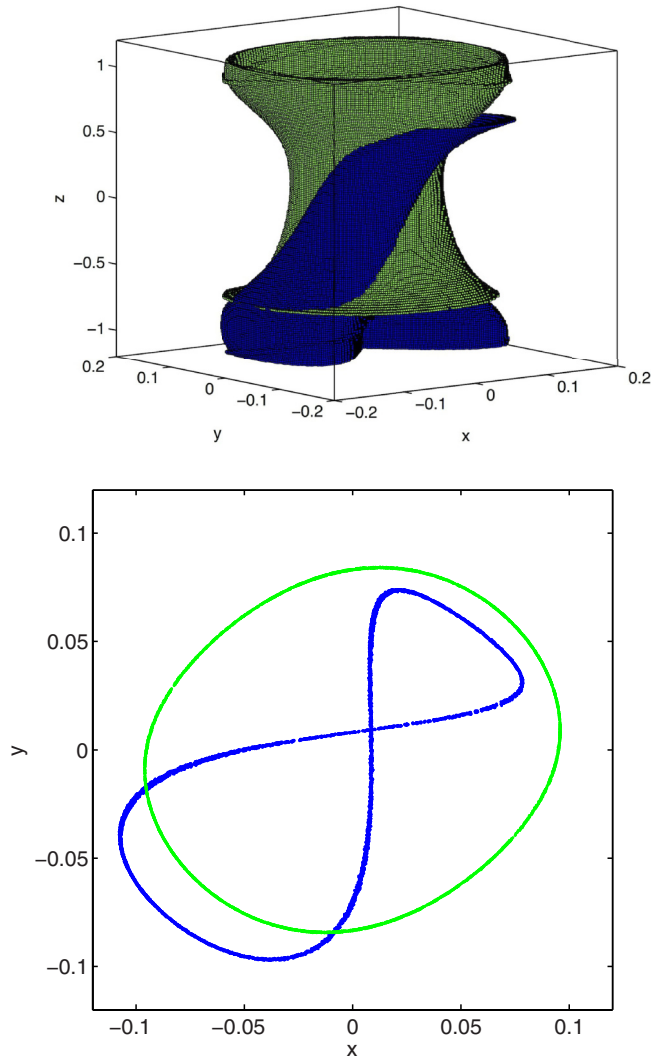
FIG. 6. (Color online) Time trace of the stable manifold of the hyperbolic periodic orbit at the north pole (light gray; green online) and of the unstable manifold of the hyperbolic periodic orbit at the south pole (black; dark blue online) in (x, y, z) space (top panel) and intersection of these entities in the (x, y) plane (bottom panel).
