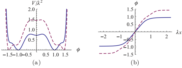
FIG. 9. (Color online) Kink solutions between the first and second first-order phase transition [ T_c^I(II) < T < T_c^I(I) ] and below the second first-order phase transition [ T < T_c^I(II) ] in \phi^{10} field theory. (a) The potentials (67) (solid curve) and (69) (dashed curve). (b) The corresponding kinks computed by solving the equation of motion d\phi/dx = \sqrt{2V(\phi)} numerically subject to the symmetry condition \phi(0) = 0 .
