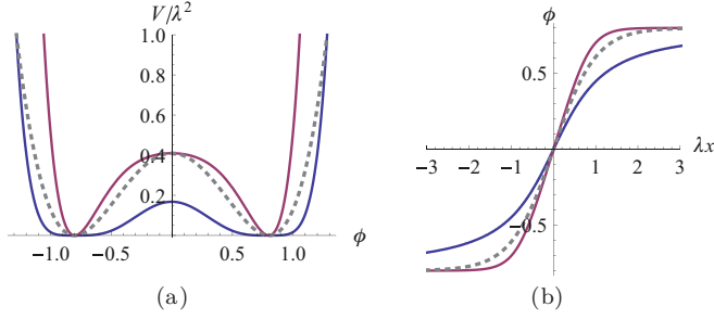
FIG. 5. (Color online) \phi^8 field theory with two degenerate minima. (a) The potentials (31) (bottom curve, blue), (35) (top curve, red), and a representative \phi^4 potential V(\phi) = \lambda^2(\phi^2 - a^2)^2 (dotted curve). (b) The corresponding kinks (32) (inner curve, blue) and (37) (outer curve, red) connecting -a to +a , and the corresponding \phi^4 kink \phi(x) = a \tanh(\lambda x) (dotted curve). In all panels, a = 4/5 and b = 1 .
