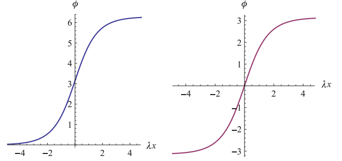
FIG. 17. (Color online) Kink solutions (201) of the n \rightarrow \infty limiting field theories V(\phi) = \lambda^2(1 - \cos \phi) on the left (blue) and V(\phi) = \lambda^2(1 + \cos \phi) on the right (red).
