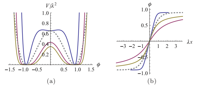
FIG. 11. (Color online) \phi^{10} field theory with two degenerate minima. (a) The potentials: (89) (top curve, blue), (94) (middle curve, red), (99) (bottom curve, yellow), and a representative \phi^4 potential V(\phi) = \lambda^2(\phi^2 - a^2)^2 (dotted curve). (b) The kink solutions connecting -a to a : (91) (outer curve, blue), (96) (inner curve, red), (100) (middle curve, yellow), and the corresponding \phi^4 kink \phi(x) = a \tanh(\lambda x) (dotted curve). In all panels, a = 9/10 and b = 1 .
