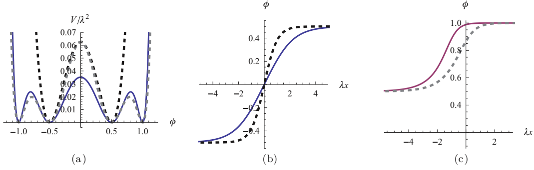
FIG. 8. (Color online) \phi^{10} field theory at the second first-order phase transition, T = T_c^I(II) . (a) The potential (45) (solid curve), a representative \phi^8 potential with four degenerate minima (3) (gray dotted curve), and a representative \phi^4 potential V(\phi) = \lambda^2(\phi^2 - a^2)^2 (black dotted curve). (b) The kink solution (60) (solid curve) connecting -a to +a and the corresponding \phi^4 kink \phi(x) = a \tanh(\lambda x) (black dotted curve). (c) The kink solution (63) (solid curve) connecting a to b and the corresponding \phi^8 kink (15) (gray dotted curve). In all panels, a = 1/2 , b = 1 , and c = 3/4 .
