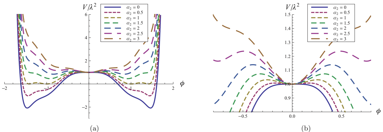
FIG. 6. (Color online) (a) Example potentials of the form (52) for various illustrative values of the coefficient of the quadratic term, \alpha_2 , showing the various phases and phase transitions in the \phi^{10} theory. (b) Magnification of (a) near the origin.
