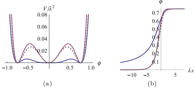
FIG. 4. (Color online) \phi^8 field theory with three degenerate minima. (a) The potentials (22) (bottom curve, blue), (26) (top curve, red), and a representative \phi^6 potential V(\phi) = \lambda^2 \phi^2 (\phi^2 - a^2)^2 (dotted curve). (b) The kink solutions (23) (top curve, blue) and (28) (bottom curve, red) connecting 0 to a , and the corresponding \phi^6 kink \phi(x) = a/\sqrt{1 + e^{-2\sqrt{2}a^2\lambda x}} (dotted curve). In all panels, a = 3/4 and b = 1 .
