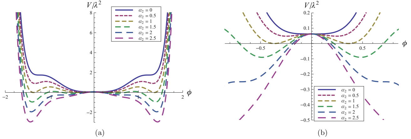
FIG. 1. (Color online) (a) Example potentials of the form (7) for various illustrative values of the coefficient of the quadratic term, \alpha_2 , showing the various phases and phase transitions in the \phi^8 theory. (b) Magnification of (a) near the origin.
