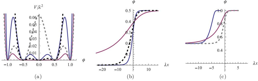
FIG. 13. (Color online) \phi^{12} field theory with five degenerate minima. (a) The potentials: (123) (top curve, blue), (130) (bottom curve, red), a representative \phi^8 potential with four degenerate minima (3) (gray dotted curve), and a representative \phi^6 potential with three degenerate minima V(\phi) = \lambda^2 \phi^2 (\phi^2 - a^2)^2 (black dotted curve). (b) The kink solutions connecting 0 to a : (124) (outer curve, blue), (132) (inner curve, red), and the corresponding \phi^6 kink \phi(x) = a/\sqrt{1 + e^{-2\sqrt{2}a^2\lambda x}} (black dotted curve). (c) The kink solutions connecting a to b : (127) (outer curve, blue), (135) (inner curve, red), and the corresponding \phi^8 kink (15) (gray dotted curve). In all panels, a = 1/2 , b = 1 , and c = 2 .
