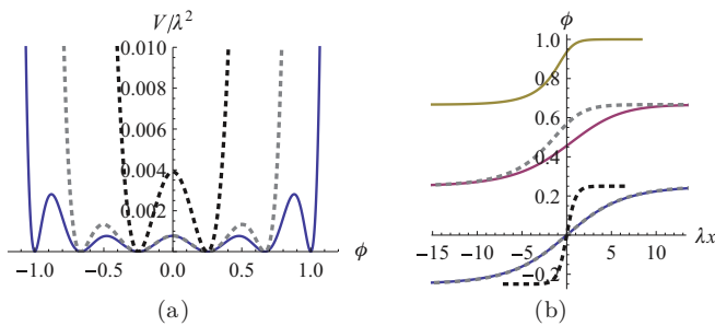
FIG. 12. (Color online) \phi^{12} field theory with six degenerate minima. (a) The potential (113) (solid curve), a representative \phi^8 potential (3) (gray dotted curve), and a representative \phi^4 potential V(\phi) = \lambda^2(\phi^2 - a^2)^2 (black dotted curve). (b) Kink solutions connecting -a to +a (114) (bottom curve, blue), a to b (117) (middle curve, red), b to c (120) (top curve, yellow), the corresponding \phi^8 kinks connecting -a to +a (11) and a to b (15) (both gray dotted curves), and the corresponding \phi^4 kink \phi(x) = a \tanh(\lambda x) (black dotted curve). In all panels, a = 1/4 , b = 2/3 , and c = 1 .
