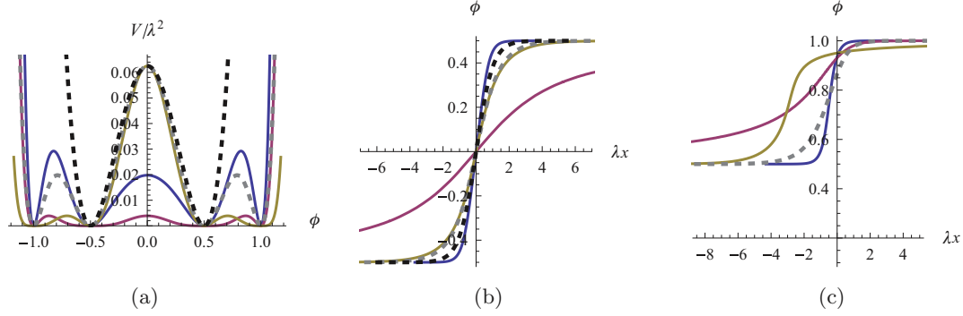
FIG. 14. (Color online) \phi^{12} field theory with four degenerate minima. (a) The potentials: (138) (second curve from top, blue), (145) (third curve from top, red), (153) (top curve, yellow), a representative \phi^8 potential with four degenerate minima (3) (gray dotted curve), and a representative \phi^4 potential V(\phi) = \lambda^2(\phi^2 - a^2)^2 (black dotted curve). (b) The kink solutions connecting -a to +a : (139) (outer curve, blue), (147) (inner curve, red), (155) (middle curve, yellow), the corresponding \phi^8 kink (11) (gray dotted curve), and the corresponding \phi^4 kink \phi(x) = a \tanh(\lambda x) (black dotted curve). (c) The kink solutions connecting a to b : (142) (outer curve, blue), (150) (inner curve, red), (158) (middle curve, yellow), and the corresponding \phi^8 kink (15) (gray dotted curve). In all panels, a = 1/2 , b = 1 , and c = 3/4 .
