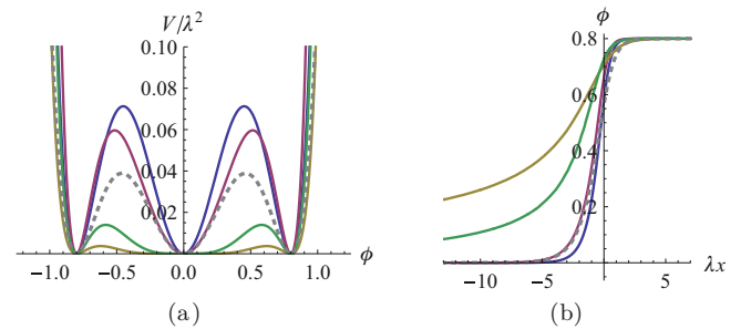
FIG. 10. (Color online) \phi^{10} field theory with three degenerate minima. (a) The potentials: (70) (top curve, blue), (75) (second curve from top, red), (80) (fourth curve from top, yellow), (84) (third curve from top, green), and a representative \phi^6 potential V(\phi) = \lambda^2 \phi^2 (\phi^2 - a^2)^2 (dotted curve). (b) The kink solutions connecting 0 to a : (72) (fourth curve from top, blue), (77) (third curve from top, red), (81) (first curve from top, yellow), (86) (second curve from top, green), and the corresponding \phi^6 kink \phi(x) = a/\sqrt{1 + e^{-2\sqrt{2}a^2\lambda x}} (dotted curve). In all panels, a = 4/5 , b = 1 , and c = 1 .
