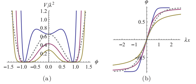
FIG. 16. (Color online) \phi^{12} field theory with two degenerate minima. (a) The potentials: (184) (top curve, blue), (189) (middle curve, red), (194) (bottom curve, yellow), and a representative \phi^4 potential V(\phi) = \lambda^2(\phi^2 - a^2)^2 (dotted curve). (b) The kink solutions connecting -a to +a : (186) (outer curve, blue), (191) (middle curve, red), (195) (inner curve, yellow), and the corresponding \phi^4 kink \phi(x) = a \tanh(\lambda x) (dotted curve). In all panels, a = 9/10 and b = 1 .
