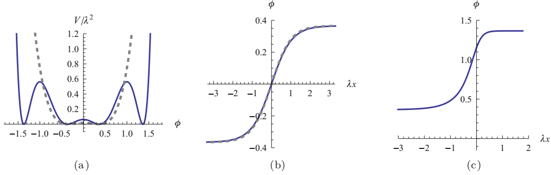
FIG. 2. (Color online) \phi^8 field theory at the first-order phase transition, T = T_c^I . (a) Example \phi^8 potential with four degenerate minima (3) and a representative \phi^4 potential V(\phi) = \lambda^2(\phi^2 - a^2)^2 superimposed as the dotted curve. (b) Kink solution (11) connecting -a to +a and the generic \phi^4 kink \phi(x) = \frac{1}{2}(\phi_{+\infty} + \phi_{-\infty}) + \frac{1}{2}(\phi_{+\infty} - \phi_{-\infty}) \tanh(\lambda x) = a \tanh(\lambda x) for \phi_{\pm\infty} = \pm a superimposed as the dotted curve. (c) Kink solution (15) connecting a to b . In all panels, a = (-1 + \sqrt{3})/2 and b = (1 + \sqrt{3})/2 .
