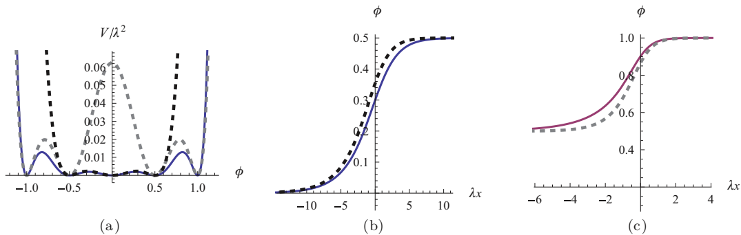
FIG. 7. (Color online) \phi^{10} field theory with five degenerate minima. (a) The potential (44) (solid curve), a representative \phi^8 potential with four degenerate minima (3) (gray dotted curve), and a representative \phi^6 potential with three degenerate minima V(\phi) = \lambda^2 \phi^2 (\phi^2 - a^2)^2 (black dotted curve). (b) The kink solution (54) (solid curve) connecting 0 to a and the corresponding \phi^6 kink \phi(x) = a/\sqrt{1 + e^{-2\sqrt{2}a^2\lambda x}} (black dotted curve). (c) The kink solution (57) (solid curve) connecting a to b and the corresponding \phi^8 kink (15) (gray dotted curve). In all panels, a = 1/2 and b = 1 .
