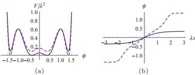
FIG. 3. (Color online) Away from the first-order phase transition, T \neq T_c^I , in \phi^8 field theory. (a) The potentials (19) (solid curve, T > T_c^I ) and (21) (dashed curve, T < T_c^I ). (b) The corresponding kinks computed by solving the equation of motion d\phi/dx = \sqrt{2V(\phi)} numerically subject to the symmetry condition \phi(0) = 0 .
