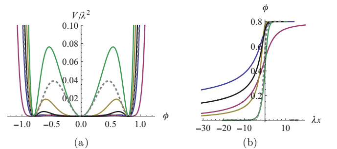
FIG. 15. (Color online) \phi^{12} field theory with three degenerate minima. (a) The potentials: (161) (fourth curve from top, blue), (165) (fifth curve from top, red), (169) (second curve from top, yellow), (174) (top curve, green), (179) (third curve from top, black), and a representative \phi^6 potential V(\phi) = \lambda^2 \phi^6 (\phi^2 - a^2)^2 (gray dotted curve). (b) The kink solutions connecting 0 to a : (162) (top curve, blue), (166) (third curve from top, red), (171) (fourth curve from top, yellow), (176) (fifth curve from top, green), (181) (second curve from top, black), and the corresponding \phi^6 kink \phi(x) = a/\sqrt{1 + e^{-2\sqrt{2}a^2\lambda x}} (gray dotted curve). In all panels, a = 4/5 and b = 1 .
