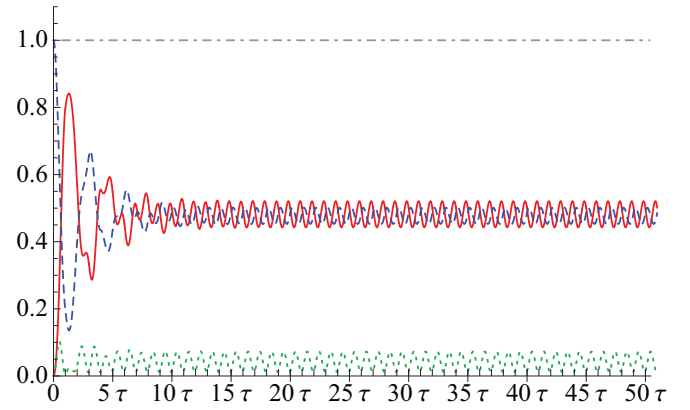
FIG. 3. (Color online) Occupation probabilities p_A(t) (red solid line), p_B(t) (blue dashed line), and p_C(t) (green dotted line) as a function of time for \gamma = \gamma_2 (18) and initial state (21); \tau in arbitrary units.
