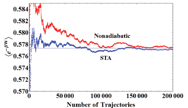
FIG. 2. (Color online) Numerical average value of \langle e^{-\beta W} \rangle vs the number of classical trajectories used, with \omega_i = 10 , \beta = 0.2 , and \omega_i\tau = 0.001 . The upper red (lower blue) line is for a bare nonadiabatic process (STA). The horizontal thin line indicates the theoretical value 1/\sqrt{3} . The protocol for \omega(t) is the same as in Fig. 1.
