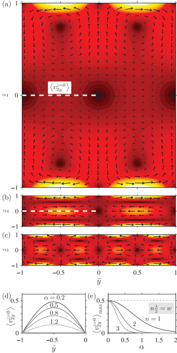
FIG. 2. (Color online) Analytical results for the streaming velocity \langle \mathbf{v}_2 \rangle in parallel-plate channels. (a) Plot of the analytical expressions (19) and (20) for \langle \mathbf{v}_2 \rangle (arrows) and its magnitude [color plot from 0 (black) to v_{\text{str}} (white)] in the vertical yz cross section of a parallel-plate channel (Fig. 1) with \lambda/2 = w ( n = 1 ) and aspect ratio \alpha = 1.2 . (b) The same as (a), but for \alpha = 0.2 . (c) The same as (b) but for a standing full wave \lambda = w ( n = 2 ). (d) Line plot of the amplitude \langle v_{2y}(\tilde{y}, 0) \rangle of the streaming velocity, in units of v_{\text{str}} , along the first half of the center axis [white dashed lines in (a) and (b)] with \lambda/2 = w for aspect ratios \alpha = 0.2, 0.5, 0.8, and 1.2 . (e) Line plot of the maximum \langle v_{2y}(\tilde{y}, 0) \rangle_{\text{max}} of the center-axis streaming velocity, in units of v_{\text{str}} , as function of aspect ratio for the resonances n\lambda/2 = w , with n = 1, 2, and 3 , respectively.
