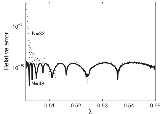
FIG. 2. The relative errors of the calculated ground state energy as a function of \lambda for N = 32 and N = 48 .
