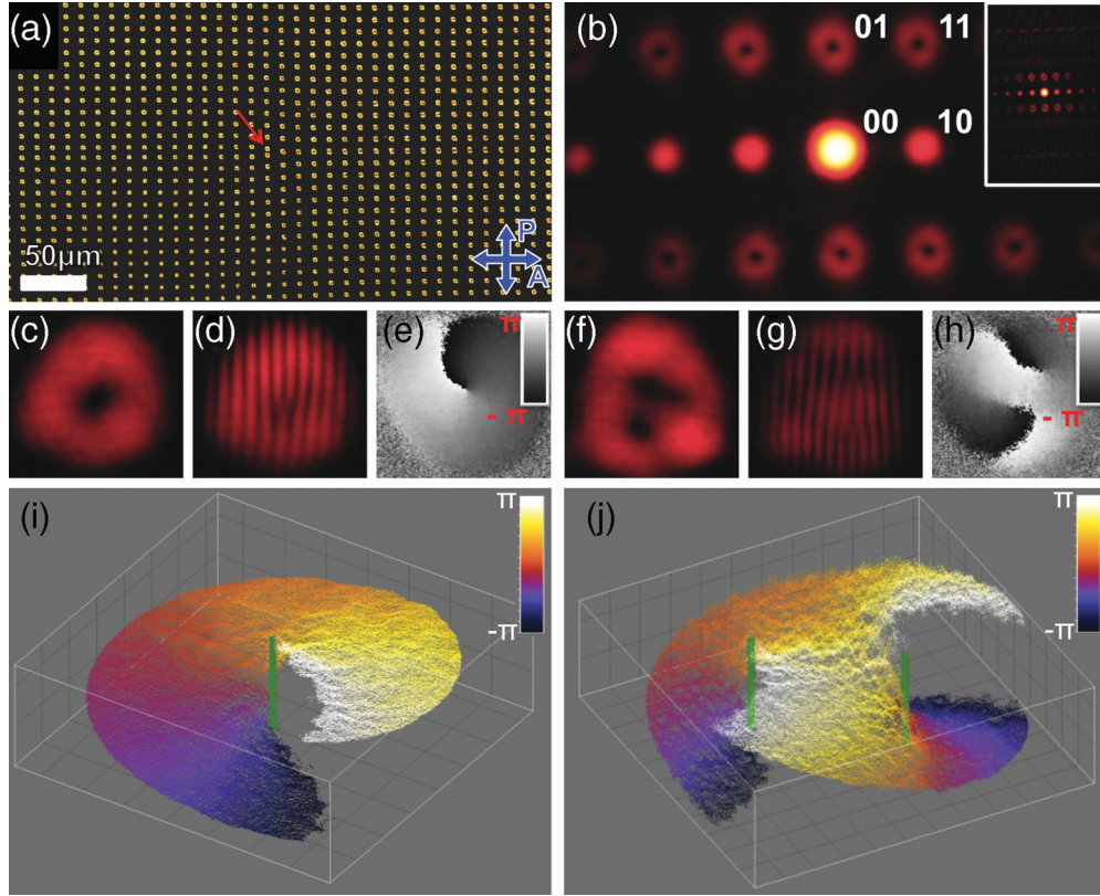
FIG. 9. (Color online) Control of phase singularities by defects in toron gratings. (a) POM texture of a square-periodic array of torons with an edge dislocation labeled by a red arrow (located near the center of the image) and (b) a corresponding diffraction pattern with diffraction orders marked on the image and a large-area view containing higher diffraction order beams shown in the inset. (c) An enlarged image of the first-order diffracted beam and (d) an interference pattern of the first-order diffraction and reference Gaussian beams obtained for their oblique incidence. (e) Phase profile of the first-order beam shown in (c). (f) An enlarged image of a second-order diffracted beam and (g) interference pattern of this beam and a reference Gaussian beam obtained for their oblique incidence. (h) Phase profile of the second-order beam shown in (f). Three-dimensional plots of the phase vs coordinates in the lateral plane of the diffracted beams of first (i) and second (j) orders, respectively, with green vertical lines showing locations of the phase singularities. The orientation of crossed polarizer and analyzer in (a) is shown by use of blue double arrows marked by “P” and “A”, respectively.
