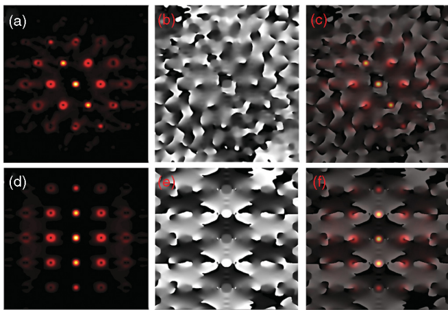
FIG. 12. (Color online) Computer-simulated (a),(d) intensity and (b),(e) phase distributions for diffraction gratings that correspond to the experimental counterparts shown in Figs. 10 and 9, respectively. (c),(f) Overlaid plots of lateral intensity and phase distributions of the diffraction patterns obtained by superimposing parts (a) with (b) and (d) with (e), respectively.
