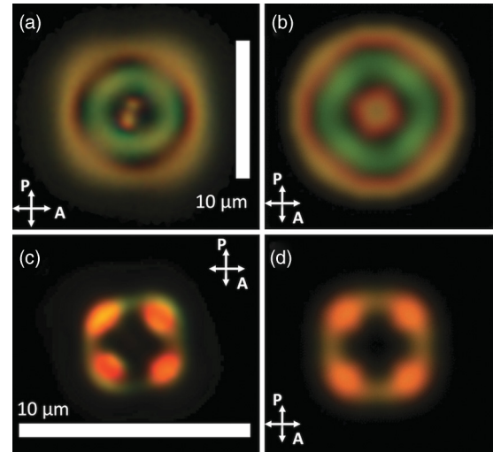
FIG. 3. (Color online) Experimental and computer-simulated POM textures of torons. (a),(c) Experimental and (b),(d) corresponding computer-simulated POM textures of laser-generated torons of different size in a (a),(b) 9- \mu\text{m} -thick cell with CNLC pitch of about 10 \mu\text{m} and (c),(d) 3.5- \mu\text{m} -thick sample with pitch of about 5 \mu\text{m} . The used CNLC materials were mixtures of the nematic host E7 and chiral dopant CB15 at concentrations corresponding to pitch values of 5 and 10 \mu\text{m} . In computer simulations, we utilized values of ordinary refractive index n_o = 1.5 , extraordinary refractive index n_e = 1.7 , and optical anisotropy \Delta n = 0.2 , closely matching that of the used LC mixtures. The crossed polarizer and analyzer are shown by white double arrows and marked by “P” and “A”, respectively.
