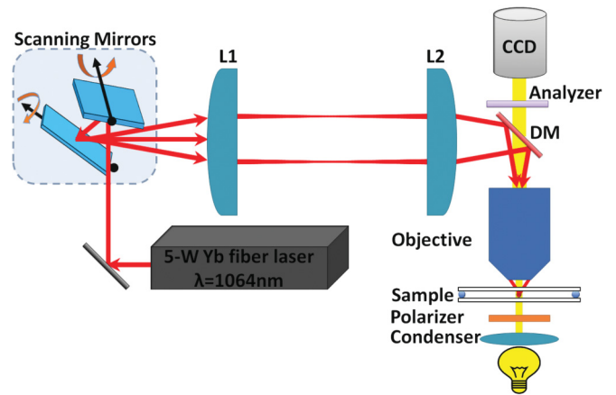
FIG. 1. (Color online) Scanning-mirror laser tweezers setup used to generate 2D patterns of torons. The CW collimated ytterbium fiber laser is controlled with a pair of scanning mirrors. Lenses L1 and L2 in a 4f configuration direct the beam into the back aperture of an objective. The scanning-mirror angles determine the 2D positions of the focused beam within the sample. The dichroic mirror (DM) allows for simultaneous laser scanning for generation of torons and POM studies of the optically controlled samples. The crossed polarizer and analyzer are used to obtain POM textures.
