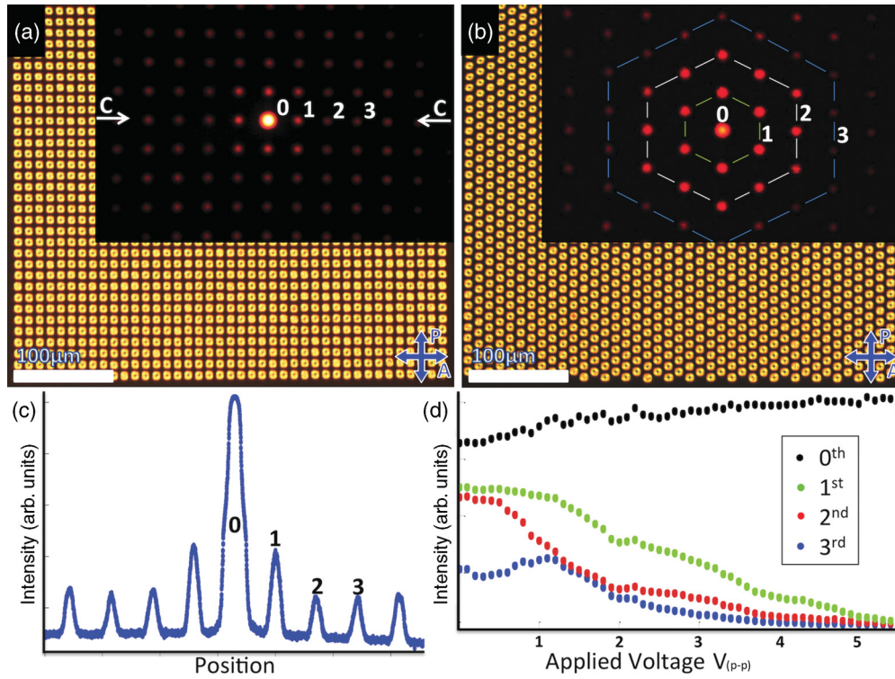
FIG. 5. (Color online) Periodic arrays of torons as voltage-tunable phase gratings. POM textures of (a) square and (b) hexagonal periodic arrays of laser-generated torons with the insets showing the corresponding diffraction patterns obtained using a 633-nm HeNe laser. Thin lines in-between the beams of the same diffraction orders shown in (b) are guides for the eye and have colors (grayscale levels) matched to the colors (grayscale levels) of corresponding data points presented in (d). (c) Horizontal intensity profile of the square-periodic diffraction pattern along the C-C line marked on (a). (d) Intensity of light in the hexagonal diffraction pattern vs applied voltage across the cell with the phase grating of torons for different diffraction orders. The crossed polarizer and analyzer are shown by blue double arrows and marked by “P” and “A”, respectively.
