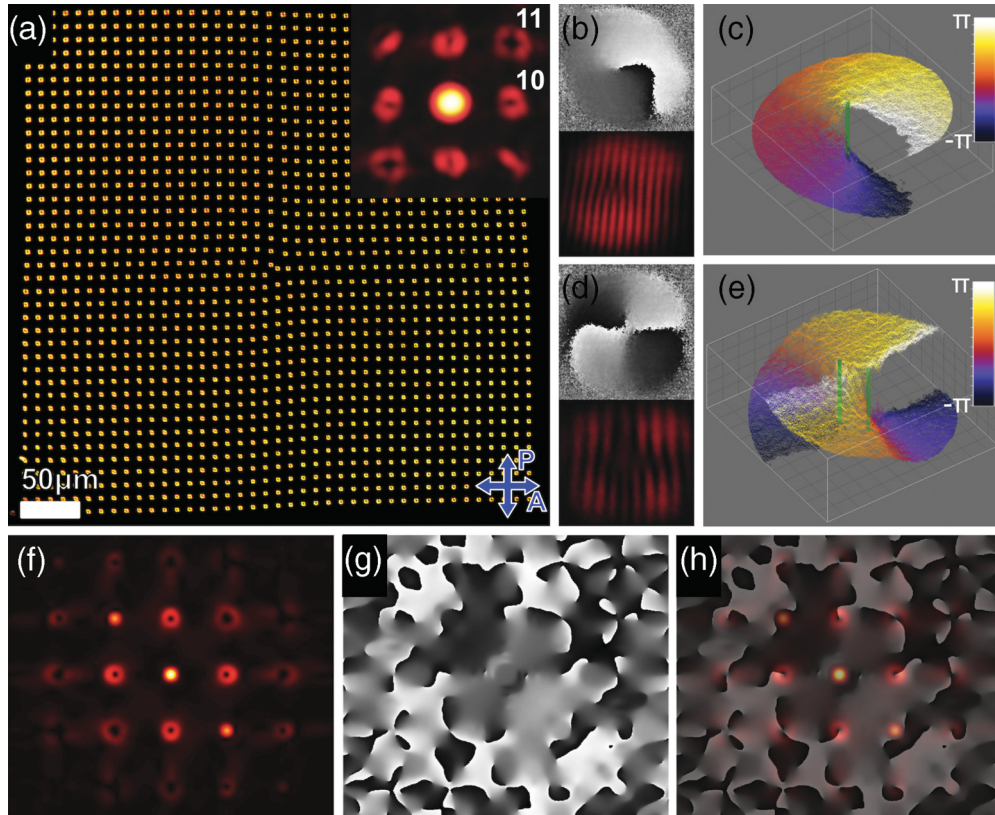
FIG. 11. (Color online) Square-periodic array of torons with defects and the corresponding diffraction pattern. (a) POM texture of the array and the corresponding diffraction pattern shown in the inset obtained for a 633-nm HeNe laser; the two diffracted beams in different diffraction orders are marked in the inset as m_x = 1, m_y = 0 and m_x = 1, m_y = 1 . (b) Phase profile (top) and an interference pattern of the m_x = 1, m_y = 0 diffraction beam and a reference Gaussian beam obtained for their oblique incidence (bottom). (c) A 3D representation of the phase vs coordinates in the lateral plane of the diffracted beam of the m_x = 1, m_y = 0 diffraction order. (d) Phase profile (top) and an interference pattern of the m_x = 1, m_y = 1 diffraction order beam and a reference Gaussian beam obtained for their oblique incidence (bottom). (e) A 3D representation of the phase vs coordinates pattern in the lateral plane of the diffracted beams of the m_x = 1, m_y = 1 diffraction order beam. (f)–(h) Computer simulation of intensity (f) and phase distribution (g) of the diffraction pattern plotted separately [(f),(g)] and then overlaid on top of each other (h). The orientation of crossed polarizer and analyzer in (a) is shown by use of blue double arrows marked by “P” and “A”, respectively.
