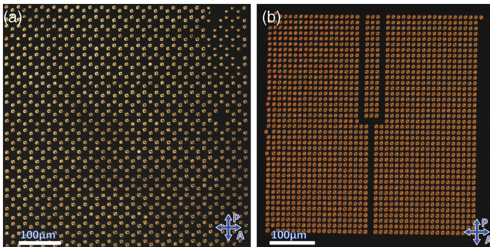
FIG. 14. (Color online) POM images of (a) a honeycomb lattice of torons and (b) a square-periodic array of torons with a bifurcated homeotropic channel. The orientation of crossed polarizer and analyzer in these POM textures is shown by use of blue double arrows marked by “P” and “A”, respectively.
