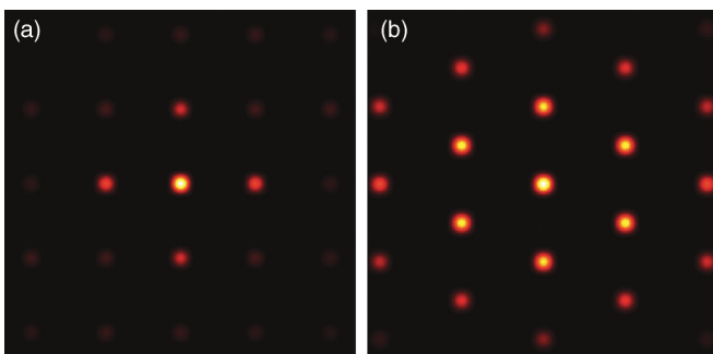
FIG. 8. (Color online) Computer-simulated diffraction patterns obtained for (a) square-periodic and (b) hexagonal arrays of torons.
