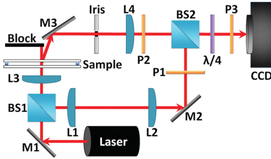
FIG. 2. (Color online) Stokes polarimetry phase characterization setup used to map the phase of diffracted laser light. A Mach-Zehnder-type interferometer is implemented by dividing a He-Ne laser beam into two paths and then recombining these two beams by beam splitters BS1 and BS2, respectively. The block and iris allow for selecting the diffraction order of interest. M1–M3 are silver mirrors used for redirecting the beam. The polarization of the beam is controlled by polarizers P1–P3 and the \lambda/4 plate. The beam is collimated by the use of lens pairs L1–L2 and L3–L4.
