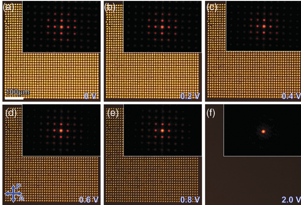
FIG. 7. (Color online) Square-periodic arrays of torons as voltage-tunable phase diffraction gratings. (a)–(f) POM textures of square-periodic arrays of laser-generated torons with the insets showing corresponding diffraction patterns obtained with a 633 nm circularly polarized HeNe laser. The orientation of crossed polarizer and analyzer at all voltages is shown in (d) by use of blue double arrows marked by “P” and “A”, respectively.
