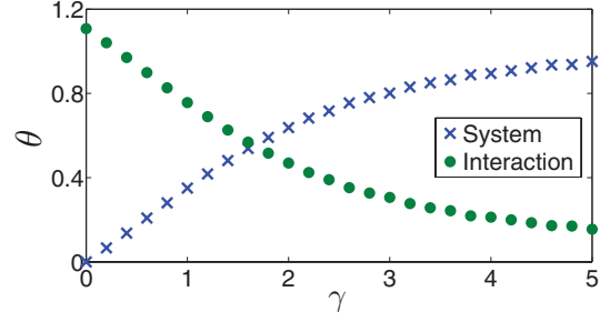
FIG. 4. (Color online) The angle to be rotated on the Bloch sphere to reach the eigenstates of H_S (crosses) or H_{SB} (solid dots) from the eigenstates of the equilibrium RDM as a function of coupling strength, for \beta = 1 , \epsilon = 0.5 , and \omega_c = 5 (in units of \Delta ).
