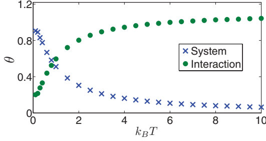
FIG. 5. (Color online) The angle to be rotated in the Bloch sphere to reach the eigenstates of H_S (crosses) or H_{SB} (solid dots) from the eigenstates of the equilibrium RDM as a function of temperature, for \gamma = 1.5 , \epsilon = 0.5 , and \omega_c = 5 (in units of \Delta ).
