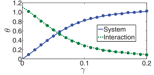
FIG. 1. (Color online) Coupling-strength dependence of the angle to be rotated on the Bloch sphere to reach eigenstates of H_S (solid line) or H_{SB} (dashed line) from eigenstates of equilibrium RDM, for \beta = 1 , \epsilon = 0.5 , and \omega_c = 5 (in units of \Delta ). Solid dots are numerically exact Monte Carlo simulations results (for details of this method, see Ref. [15]).
