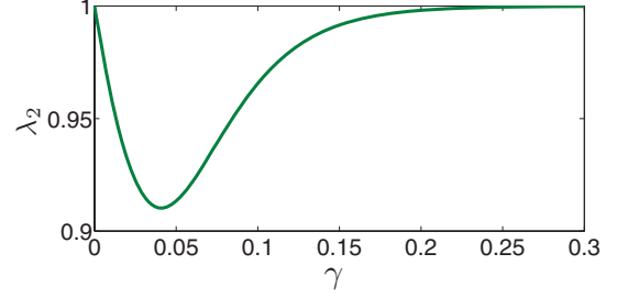
FIG. 6. (Color online) The larger eigenvalue, \lambda_2 of RDM, plotted against the SBC strength \gamma , for T = 0 , \epsilon = 0.5 , and \omega_c = 5 (in units of \Delta ).
