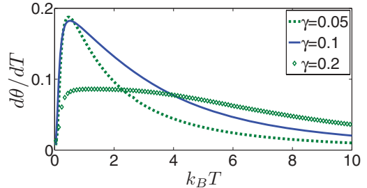
FIG. 3. (Color online) Sensitivity of the RDM diagonal representation to temperature variation, as described by d\theta/dT vs T . \theta is the angle to be rotated to reach eigenstates of H_S from eigenstates of the equilibrium RDM. System parameters are given by \epsilon = 0.5 and \omega_c = 5 (in unit of \Delta ).
