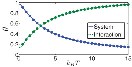
FIG. 2. (Color online) Temperature dependence of the angle to be rotated on the Bloch sphere to reach eigenstates of H_S (solid line) or H_{SB} (dashed line) from eigenstates of equilibrium RDM, for \gamma = 0.1 , \epsilon = 0.5 , and \omega_c = 5 (in unit of \Delta ). Solid dots are numerically exact Monte Carlo simulation results.
